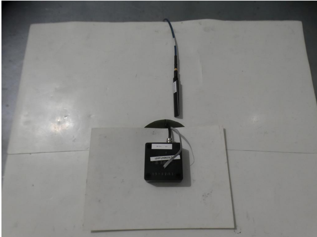
Photo 6: Test setup. EUT detail
