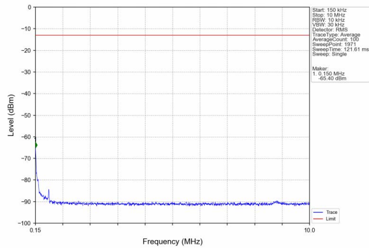
Band66_10MHz_QPSK_HCH_1775MHz_RB_1_0_NTNV
