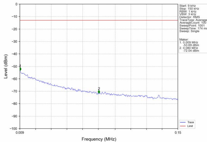
Band2_15MHz_16QAM_HCH_1902.5MHz_RB_1_0_NTNV
