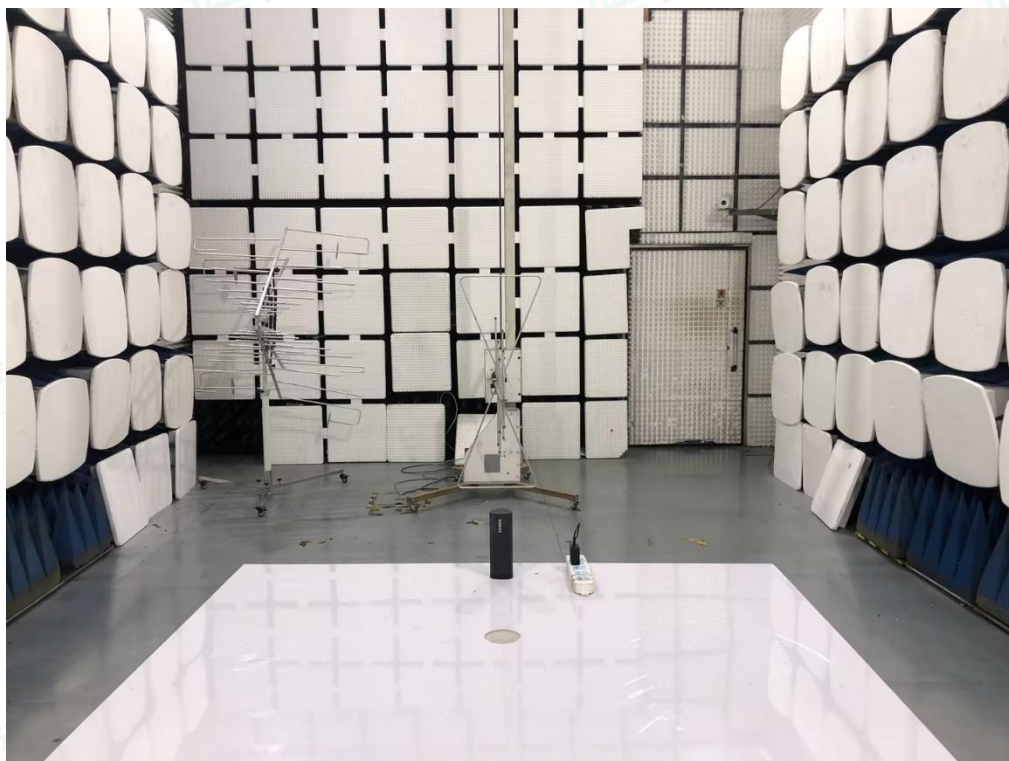
Radiated Emission below 1GHz -AC adapter charge mode
