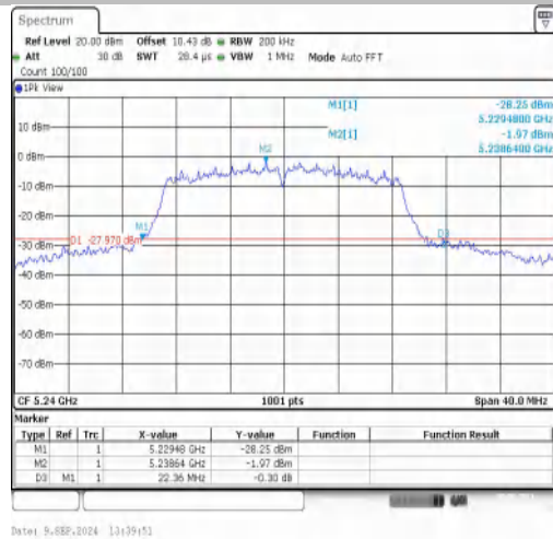
11N20MIMO-Ant2-5240
