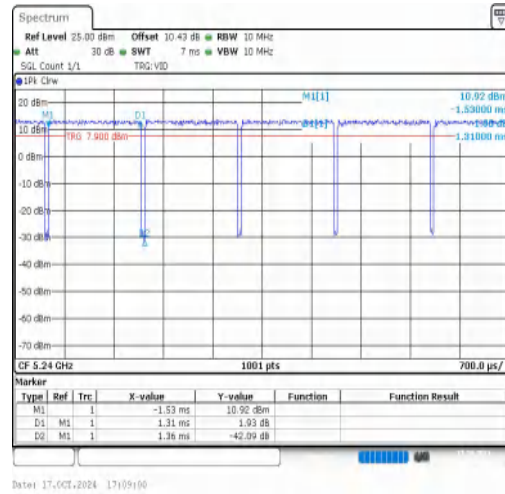
NTNV-11AC20MIMO-Ant2-5240
