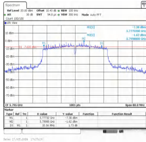
11AC40MIMO-Ant2-5795-PASS
