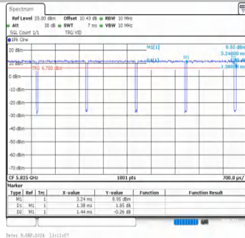
NTNV-11A-CDD-Ant2-5825
