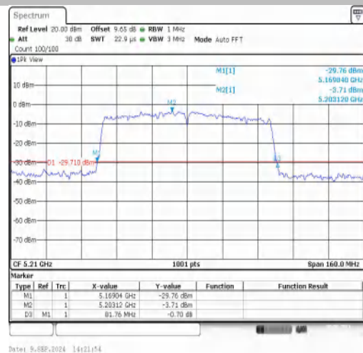
11AC80MIMO-Ant2-5210
