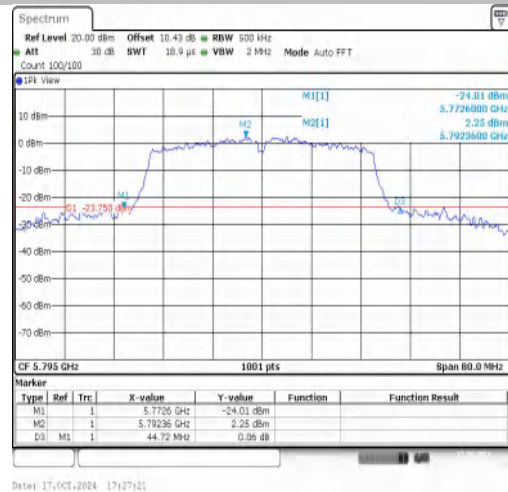
11AC40MIMO-Ant2-5795
