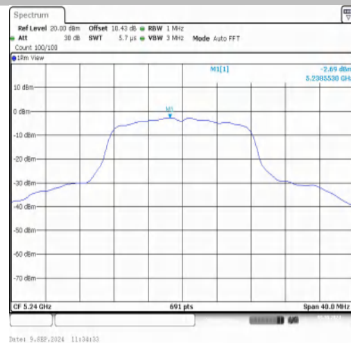
11A-CDD-Ant2-5240-PASS
