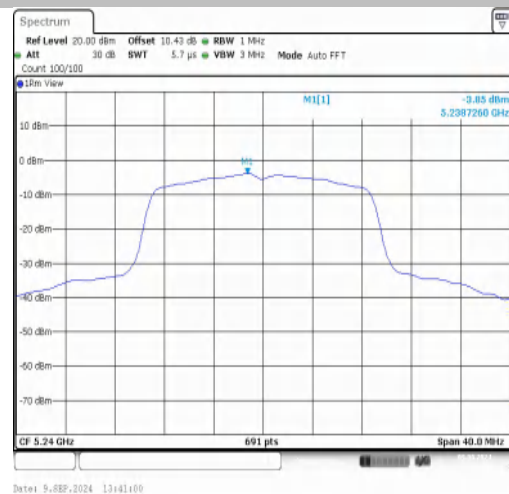
11N20MIMO-Ant2-5240-PASS
