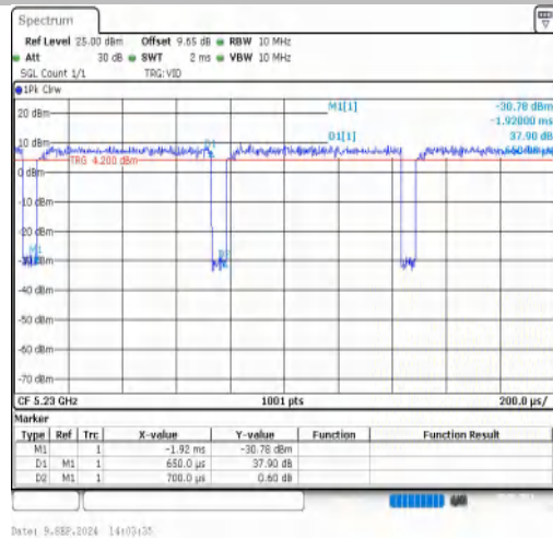
NTNV-11N40MIMO-Ant2-5230
