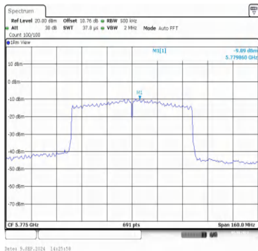
11AC80MIMO-Ant1-5775-PASS
