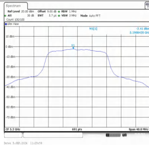
11A-CDD-Ant2-5200-PASS
