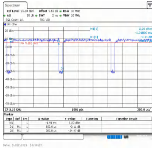
NTNV-11N40MIMO-Ant2-5190
