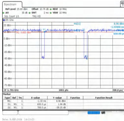
NTVN-11N40MIMO-Ant1-5795
