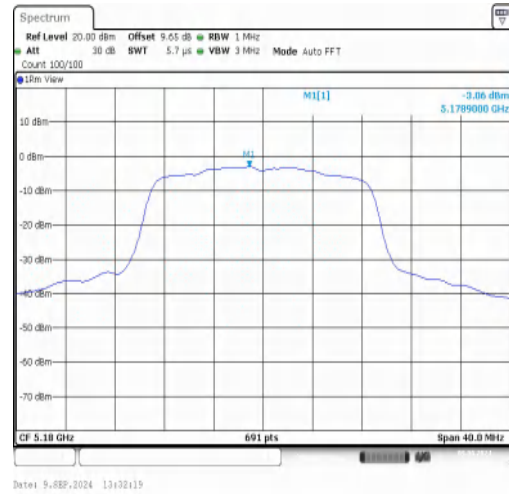
11N20MIMO-Ant2-5180-PASS
