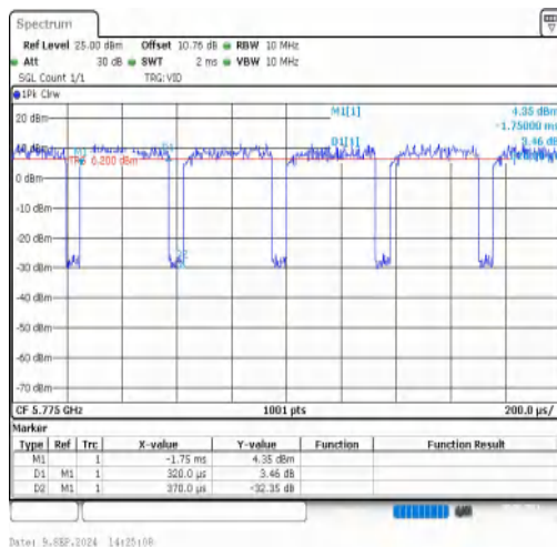
NTNV-11AC80MIMO-Ant1-5775
