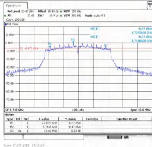
11AC20MIMO-Ant2-5745-PASS
