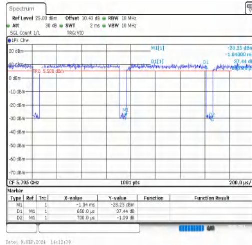
NTVN-11N40MIMO-Ant2-5795
