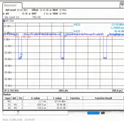
NTNV-11N40MIMO-Ant2-5755
