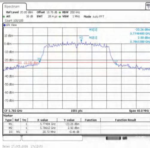
11AC20MIMO-Ant1-5785
