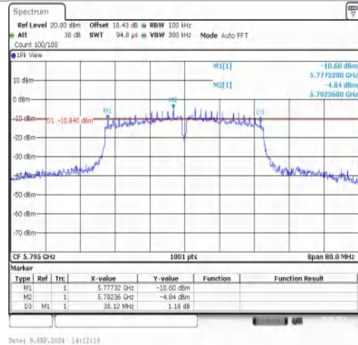
11N40MIMO-Ant2-5795-PASS
