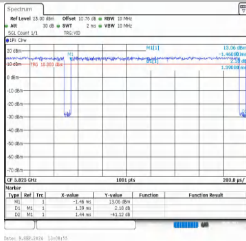
NTNV-11A-CDD-Ant1-5825
