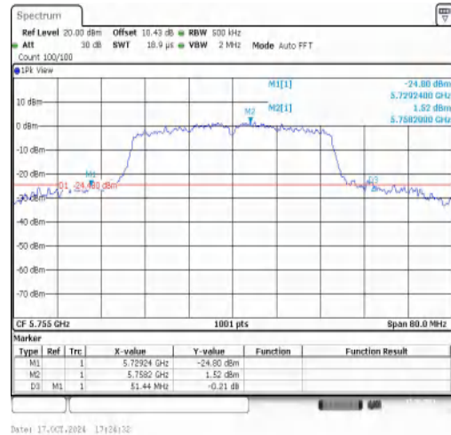
11AC40MIMO-Ant2-5755
