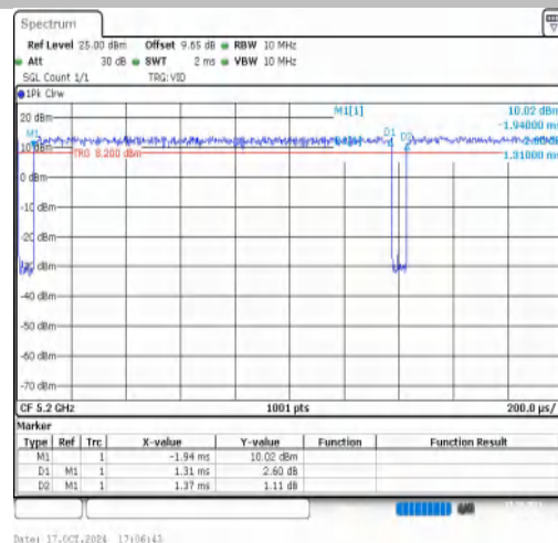
NTVN-11AC20MIMO-Ant2-5200
