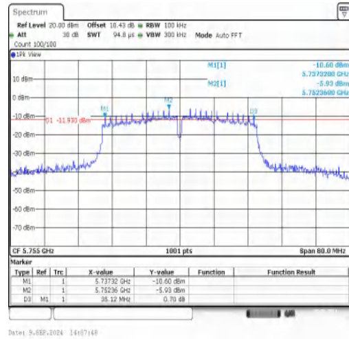
11N40MIMO-Ant2-5755-PASS
