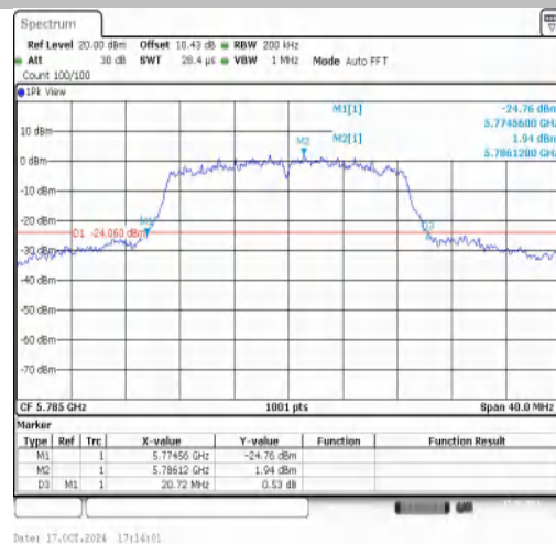
11AC20MIMO-Ant2-5785
