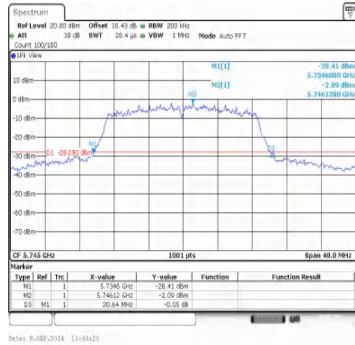
11N20MIMO-Ant2-5745
