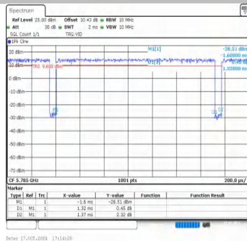
NTNV-11AC20MIMO-Ant2-5785
