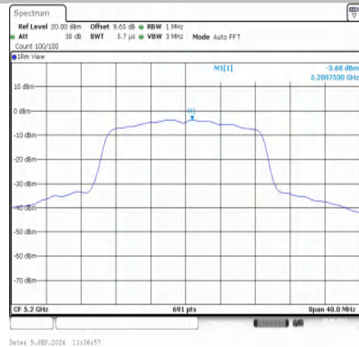
11N20MIMO-Ant2-5200-PASS
