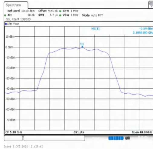
11A-CDD-Ant2-5180-PASS
