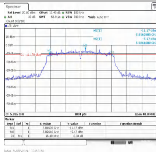
11N20MIMO-Ant2-5825-PASS
