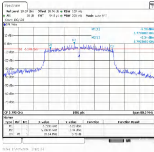
11AC40MIMO-Ant1-5795-PASS
