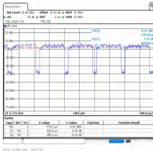
NTNV-11AC80MIMO-Ant2-5775
