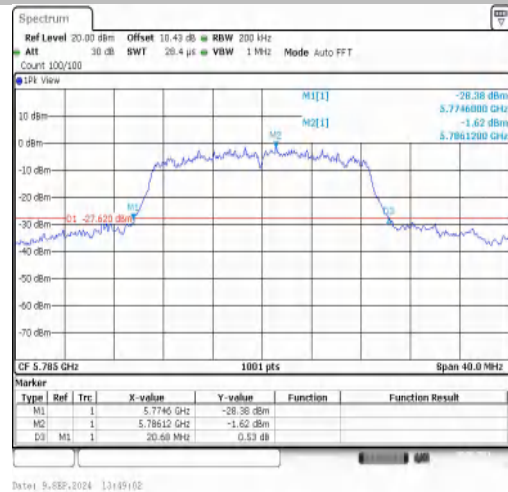
11N20MIMO-Ant2-5785
