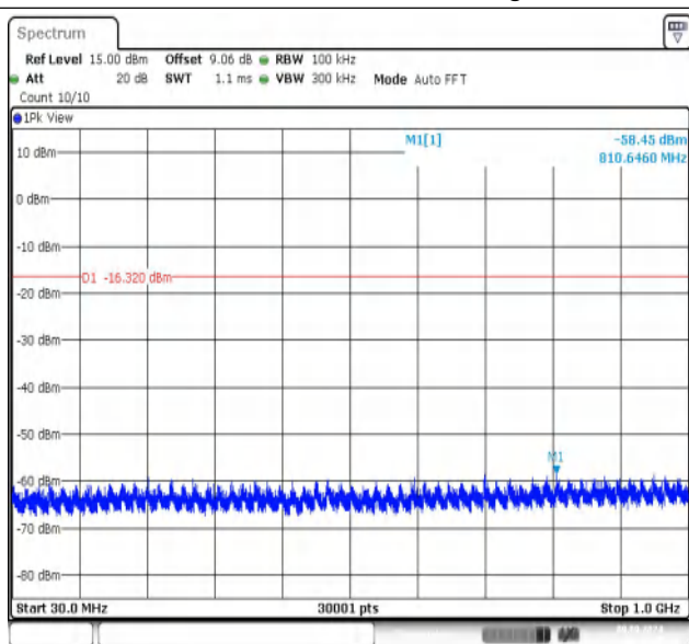
11G-CDD-Ant1-2462-30~1000-PASS
