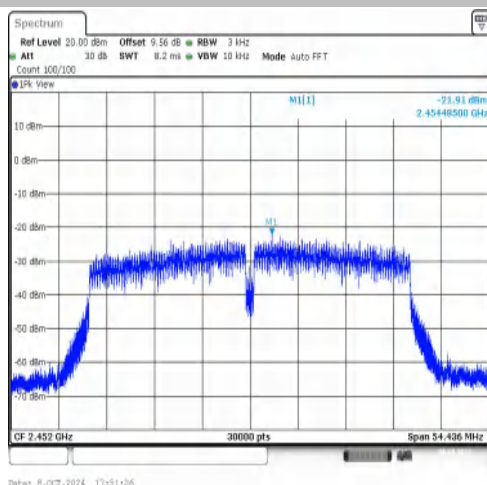
11N40MIMO-Ant1-2452-PASS
