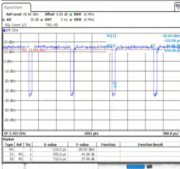
NTNV-11N40MIMO-Ant1-2422
