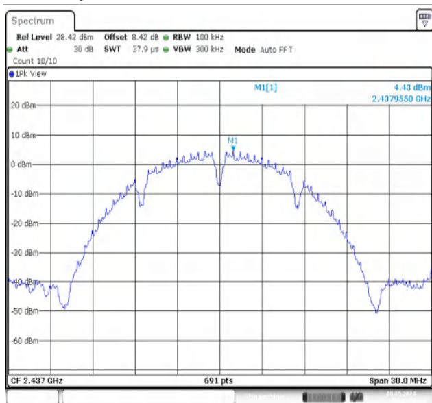
11B-CDD-Ant2-2437-0~Reference-PASS
