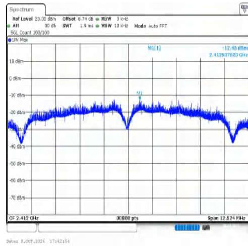
11B-CDD-Ant2-2412-PASS
