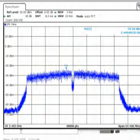
11N40MIMO-Ant2-2452-PASS
