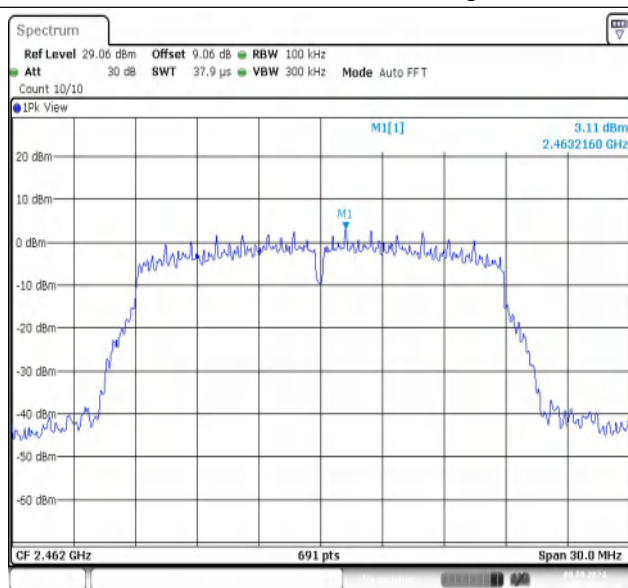
11N20MIMO-Ant1-2462-0~Reference-PASS
