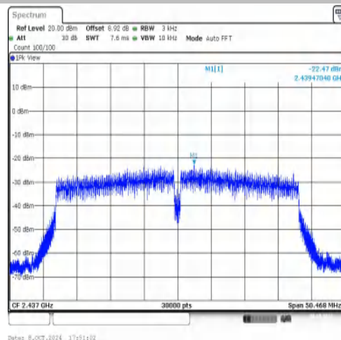
11N40MIMO-Ant2-2437-PASS
