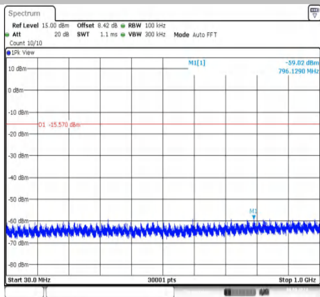
11B-CDD-Ant2-2437-0~Reference-PASS
