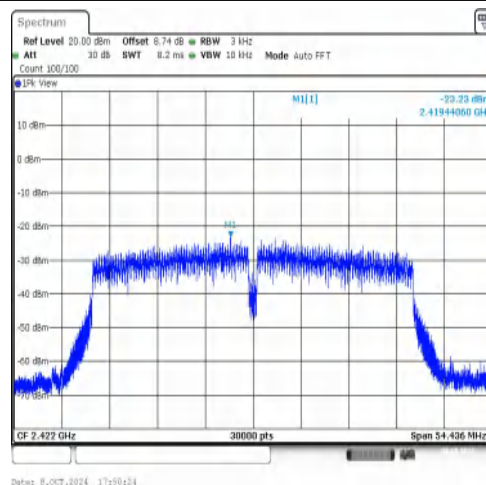
11N40MIMO-Ant2-2422-PASS
