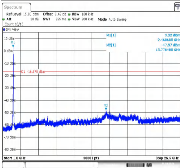
11G-CDD-Ant2-2462-1000~26500-PASS
