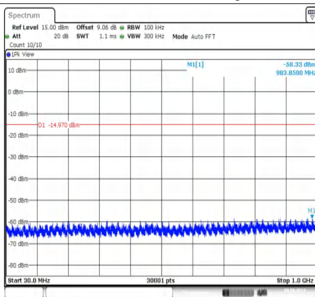
11B-CDD-Ant1-2437-30~1000-PASS
