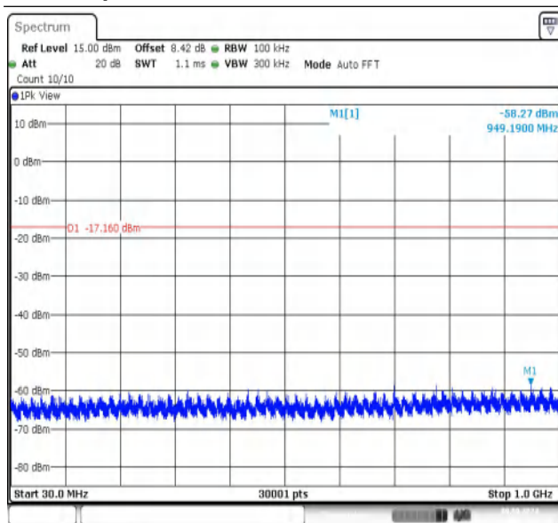
11G-CDD-Ant2-2437-30~1000-PASS
