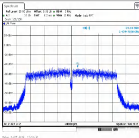
11N40MIMO-Ant1-2437-PASS
