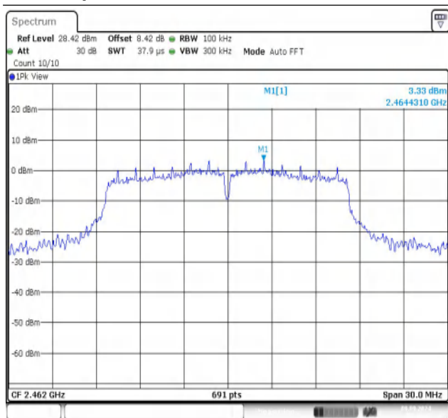
11G-CDD-Ant2-2462-0~Reference-PASS
