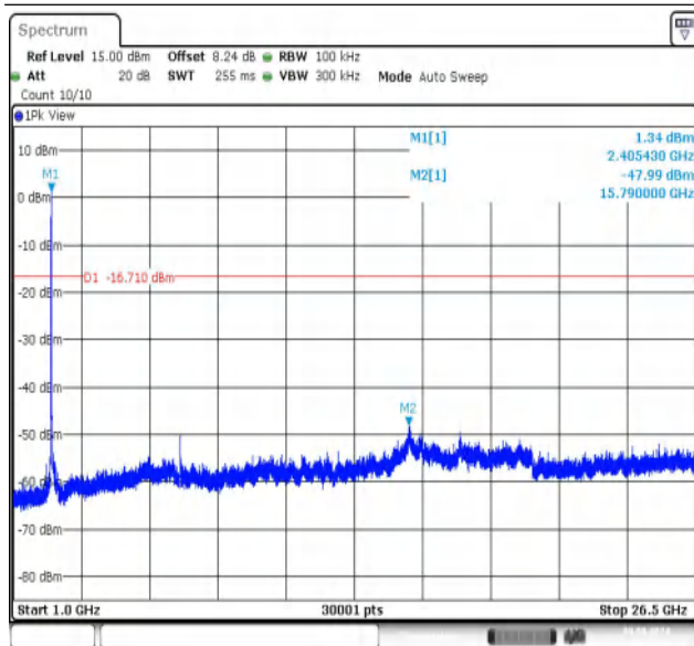
11G-CDD-Ant2-2412-1000~26500-PASS
