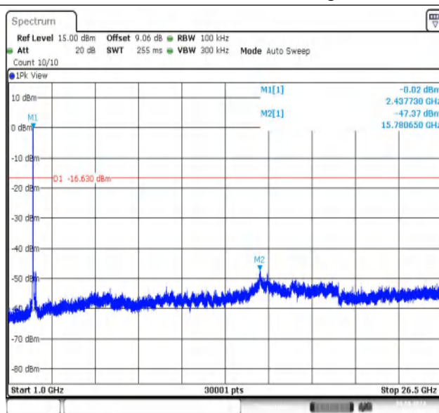
11G-CDD-Ant1-2437-1000~26500-PASS
