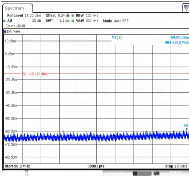
11B-CDD-Ant2-2412-30~1000-PASS
