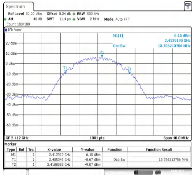
11B-CDD-Ant2-2412
