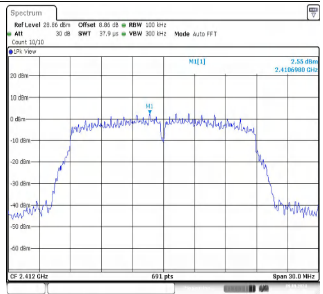
11N20MIMO-Ant1-2412-0~Reference-PASS
