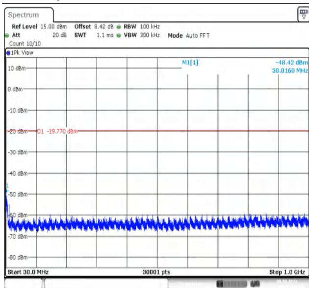
11N40MIMO-Ant2-2437-30~1000-PASS
