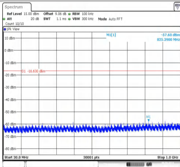
11G-CDD-Ant1-2437-0~Reference-PASS
