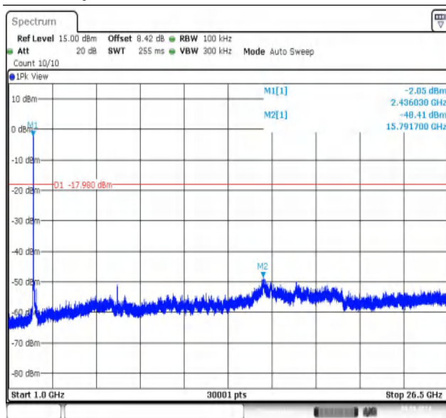
11N20MIMO-Ant2-2437-1000~26500-PASS
