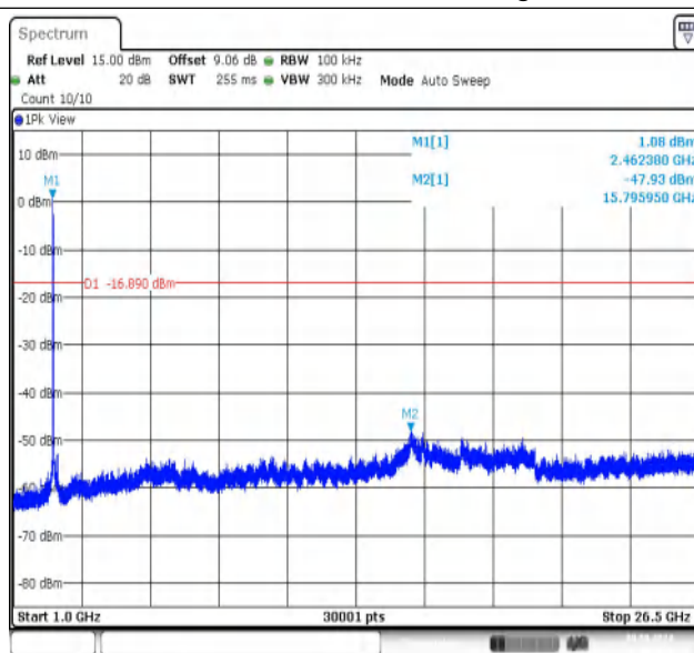
11N20MIMO-Ant1-2462-1000~26500-PASS
