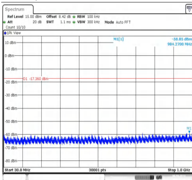
11N20MIMO-Ant2-2462-30~1000-PASS
