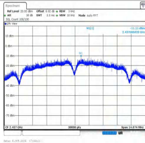
11B-CDD-Ant2-2437-PASS
