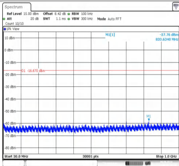
11G-CDD-Ant2-2462-0~Reference-PASS
