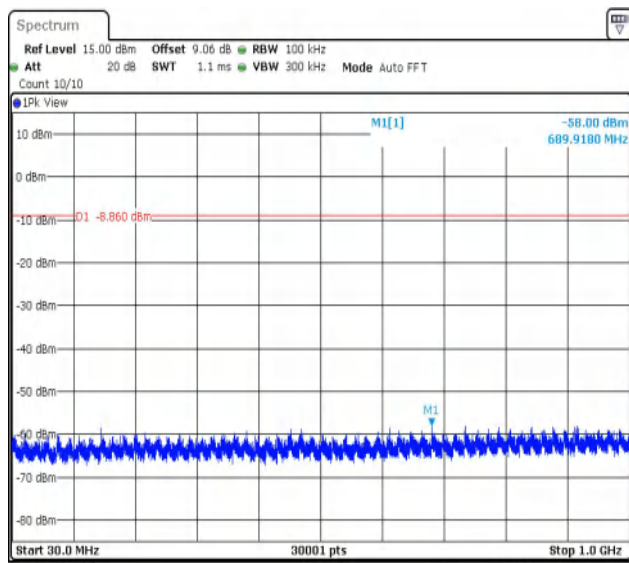
DH5-Ant1-2441-30~1000-PASS
