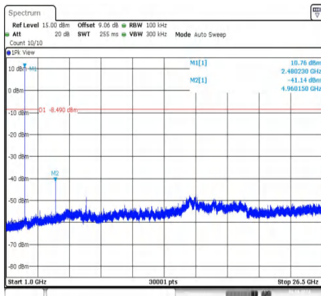
2DH5-Ant1-2480-1000~26500-PASS
