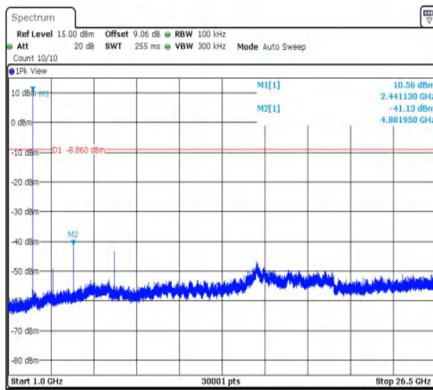
DH5-Ant1-2441-1000~26500-PASS
