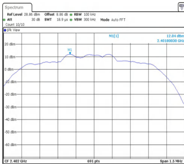
2DH5-Ant1-2402-0~Reference-PASS
