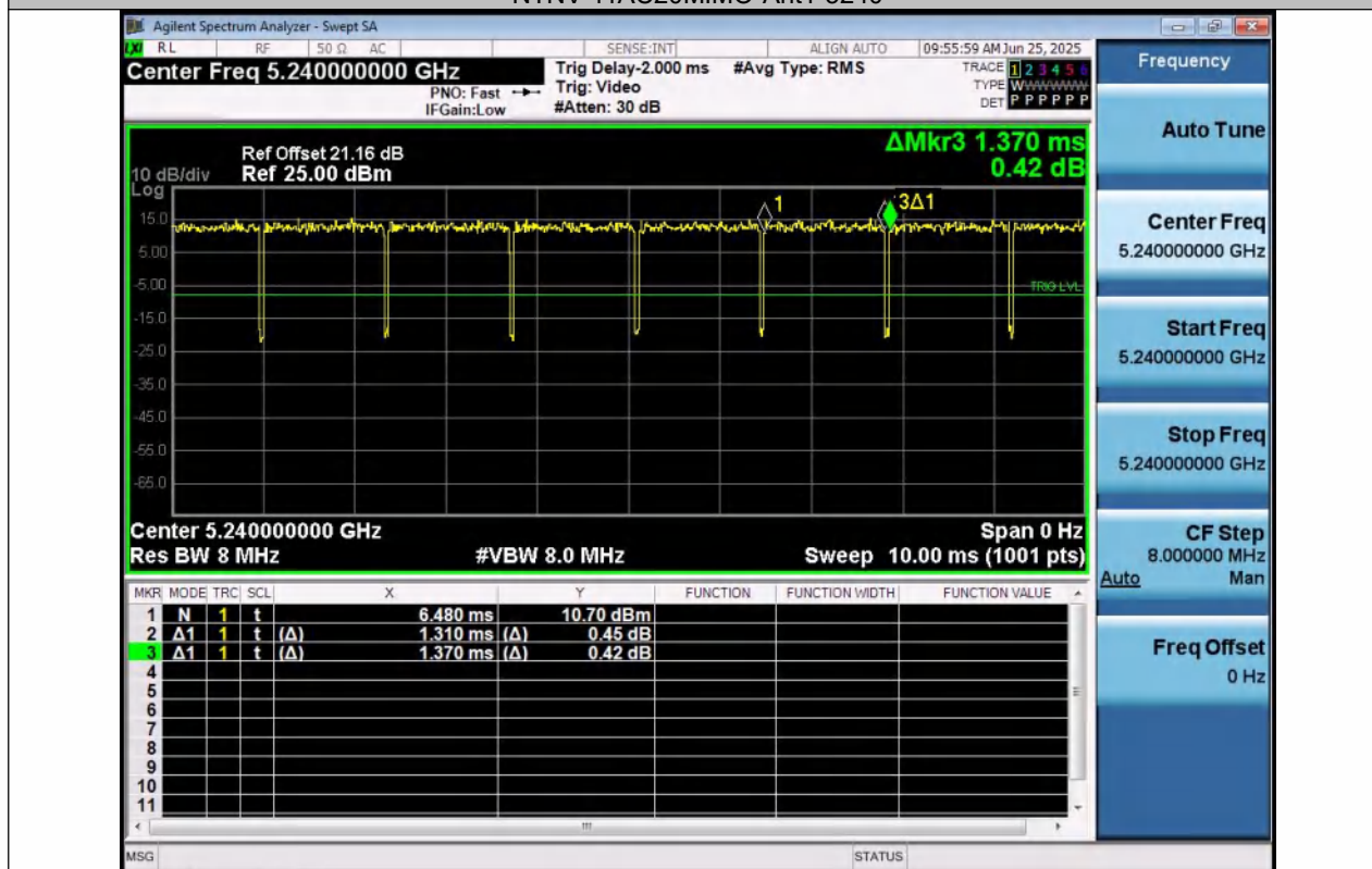
NTNV-11AC20MIMO-Ant2-5240
