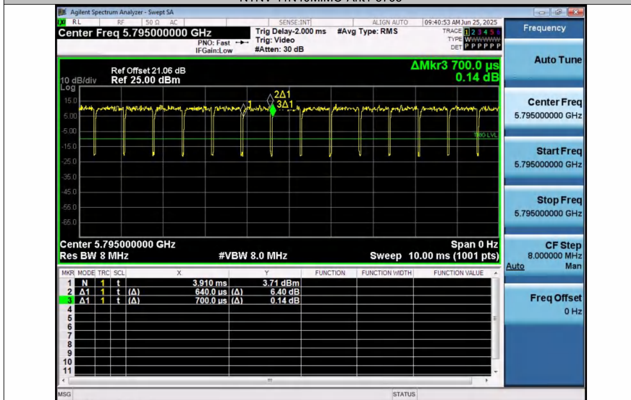
NTNV-11N40MIMO-Ant2-5795
