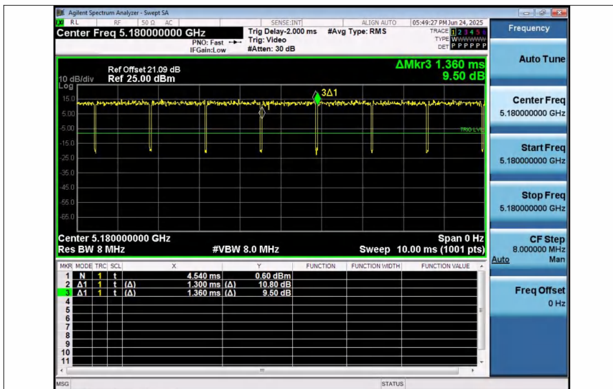
NTNV-11N20MIMO-Ant1-5180
