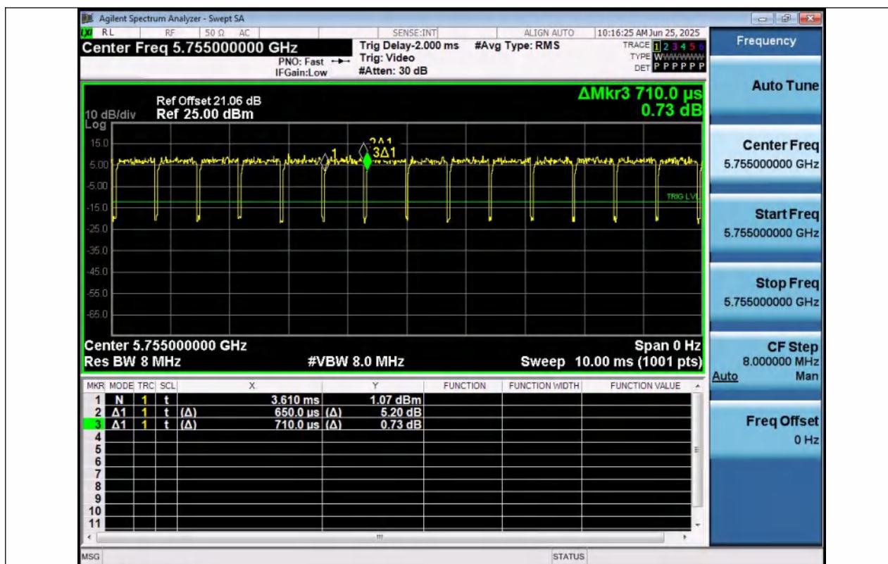
NTNV-11AC40MIMO-Ant1-5755
