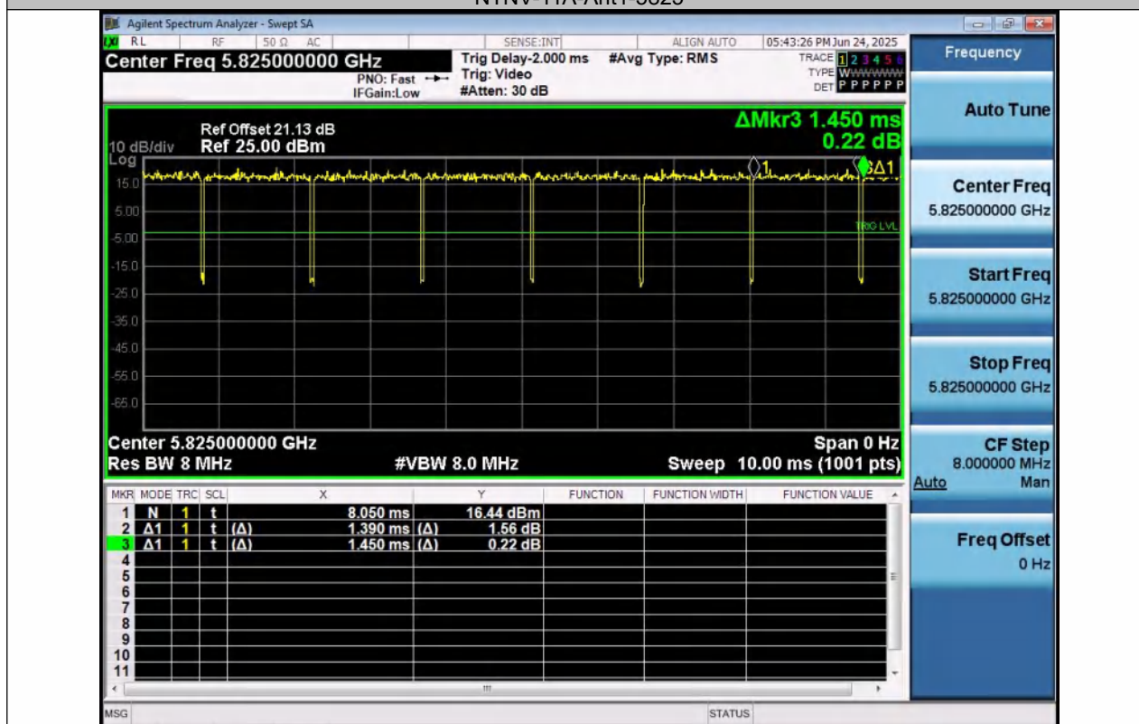
NTNV-11A-Ant2-5825
