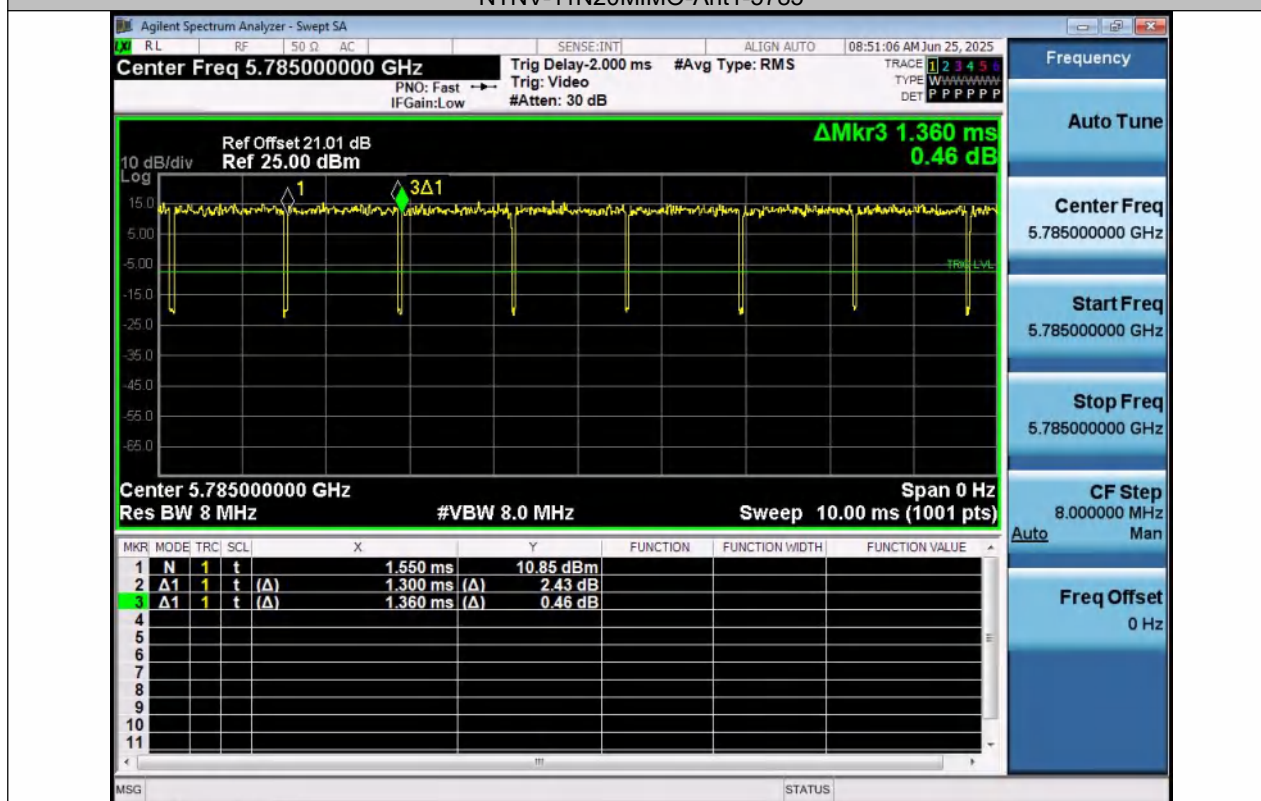
NTNV-11N20MIMO-Ant2-5785
