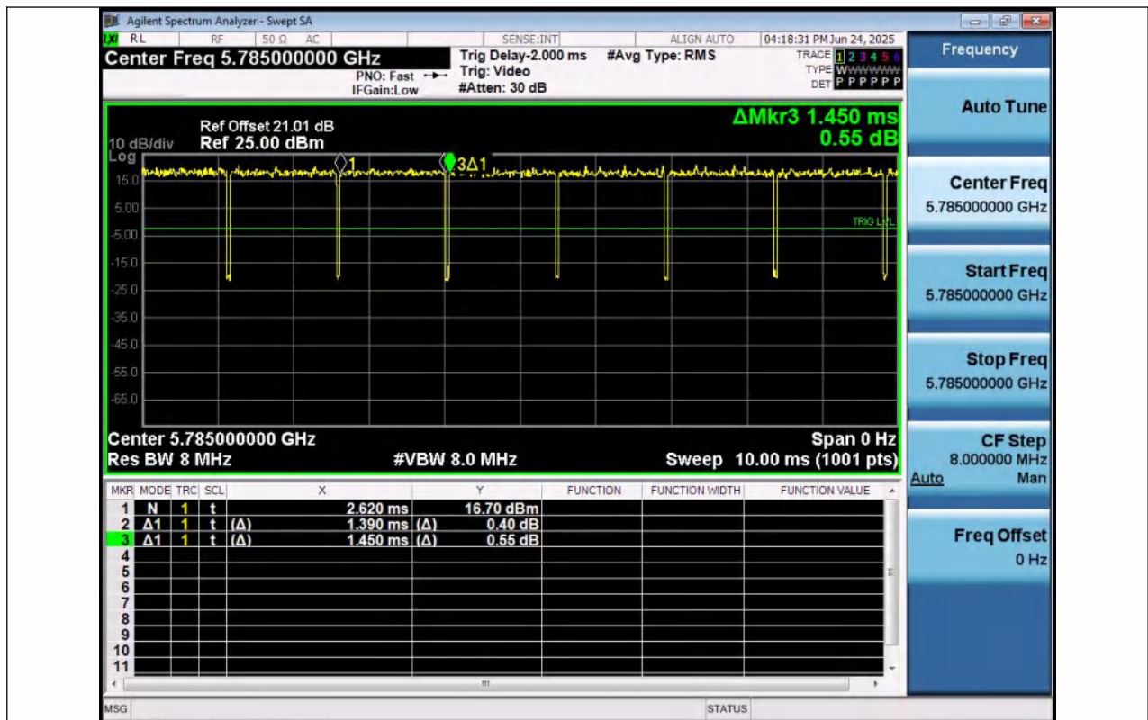
NTNV-11A-Ant1-5785
