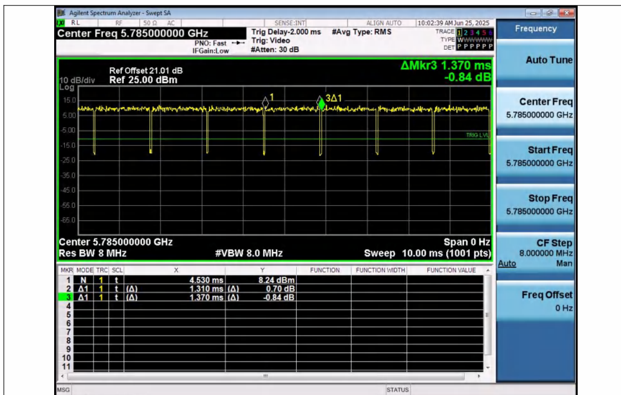
NTNV-11AC20MIMO-Ant1-5785
