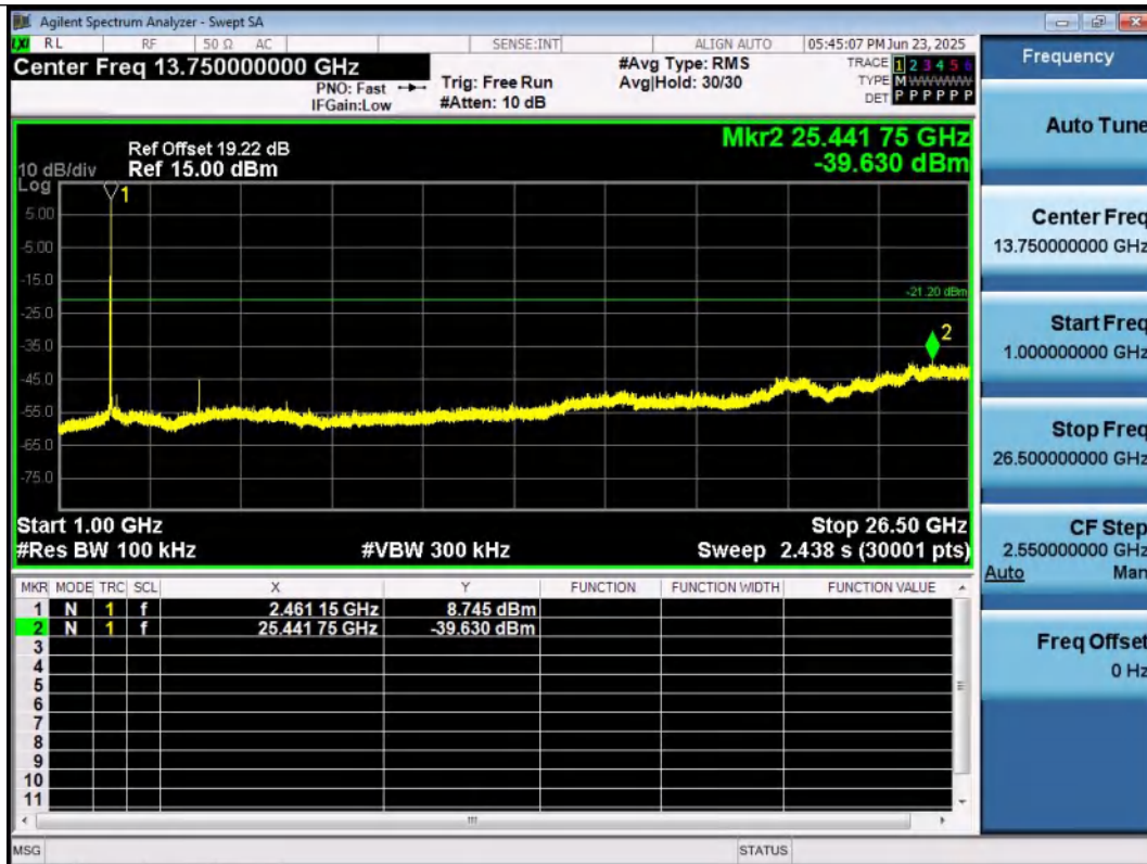
11B-Ant1-2462-1000~26500-PASS
