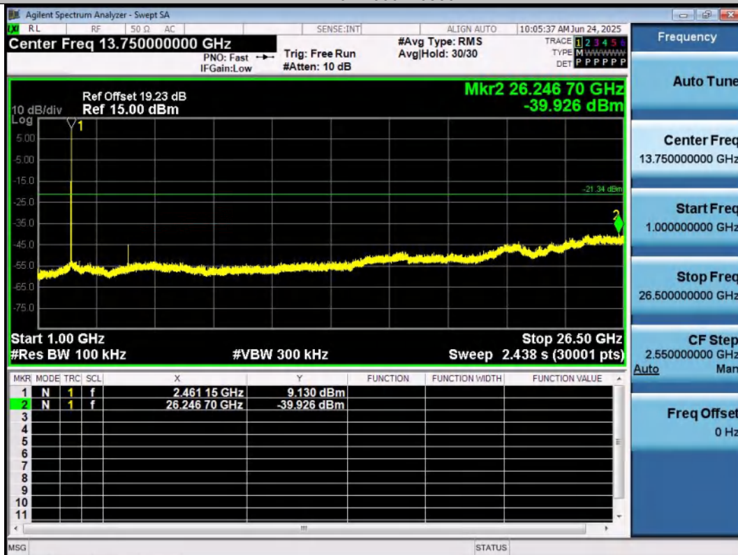
11B-Ant2-2462-1000~26500-PASS
