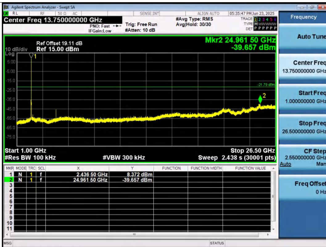
11B-Ant1-2437-1000~26500-PASS
