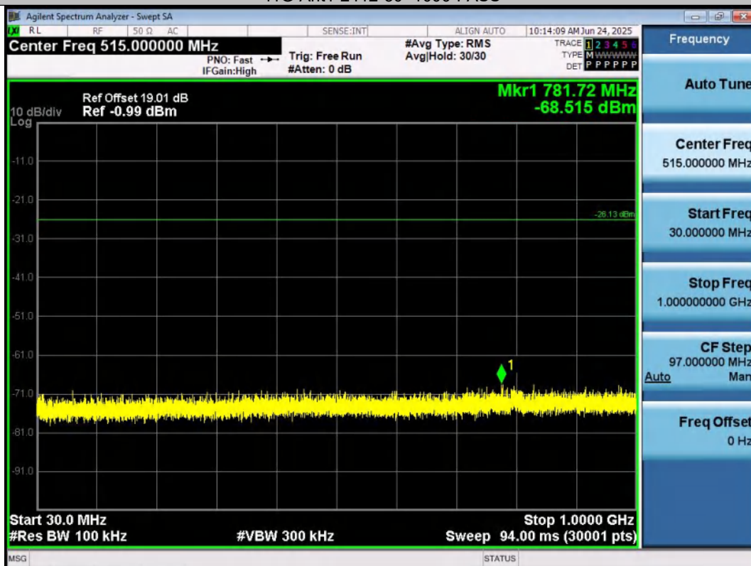
11G-Ant2-2412-30~1000-PASS
