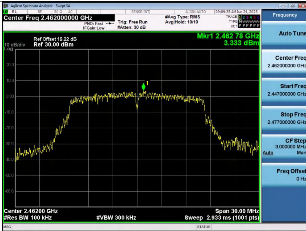
11G-Ant1-2462-0~Reference-PASS
