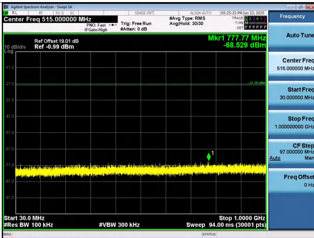
11B-Ant1-2412-30~1000-PASS
