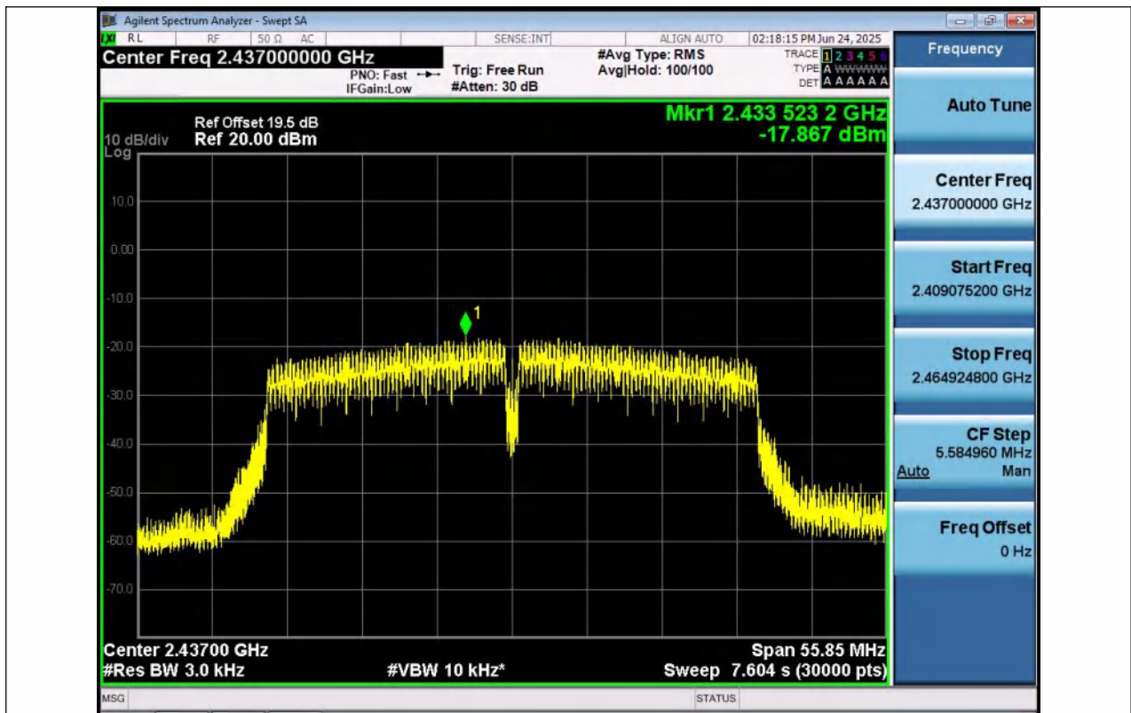
11N40MIMO-Ant1-2437-PASS
