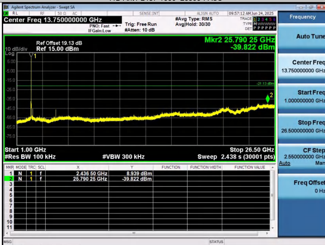
11B-Ant2-2437-1000~26500-PASS
