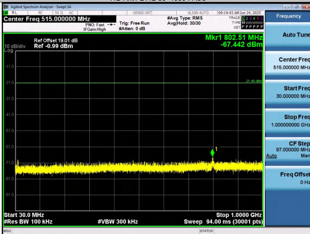
11B-Ant2-2412-30~1000-PASS
