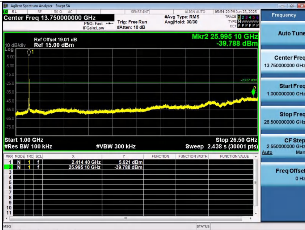
11G-Ant1-2412-1000~26500-PASS
