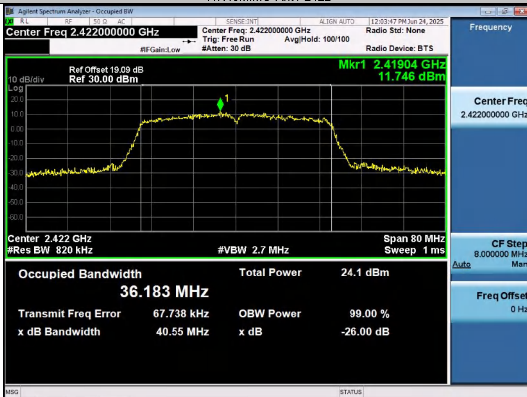
11N40MIMO-Ant2-2422
