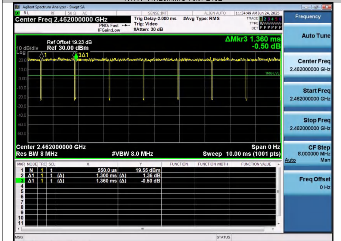
NTNV-11N20MIMO-Ant2-2462
