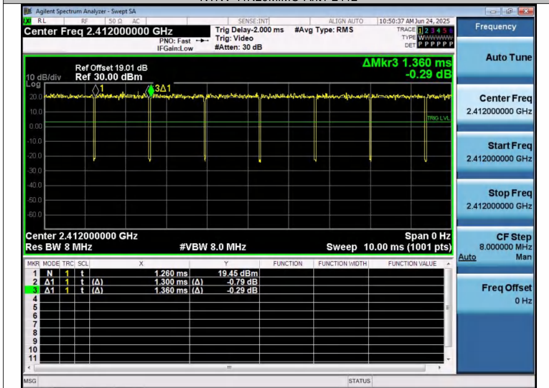
NTNV-11N20MIMO-Ant2-2412
