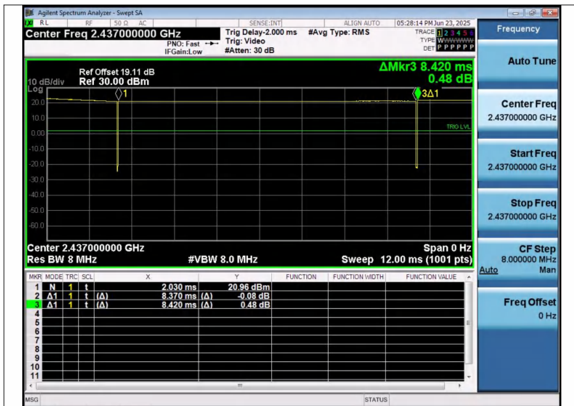
NTNV-11B-Ant1-2437
