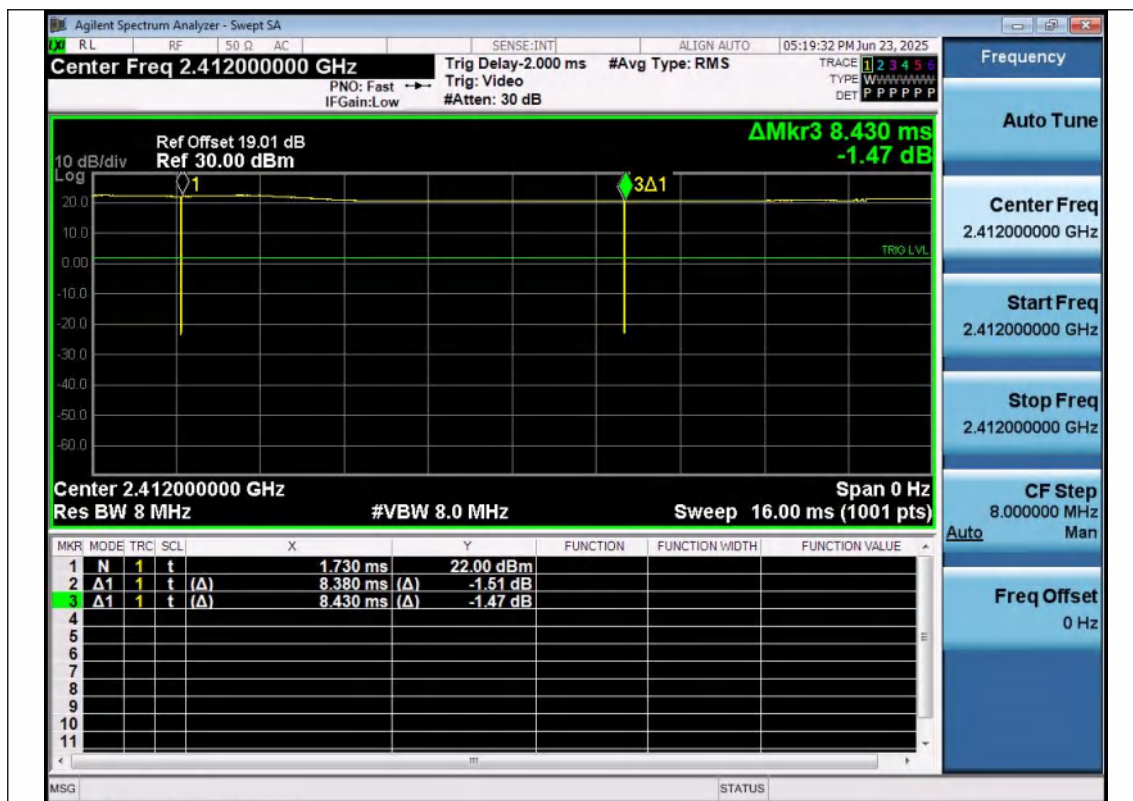
NTNV-11B-Ant1-2412
