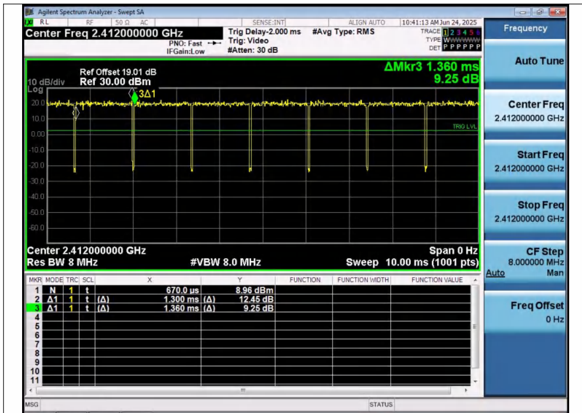
NTNV-11N20MIMO-Ant1-2412
