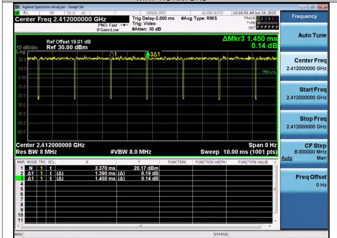
NTNV-11G-Ant2-2412
