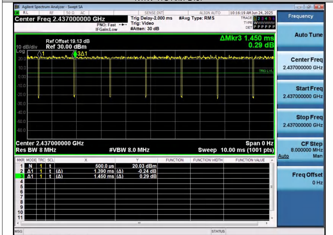
NTVN-11G-Ant2-2437
