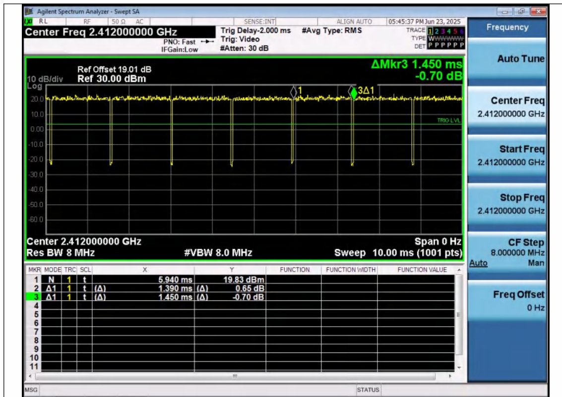
NTNV-11G-Ant1-2412
