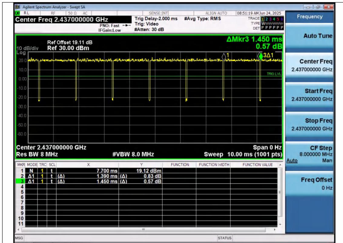
NTVN-11G-Ant1-2437
