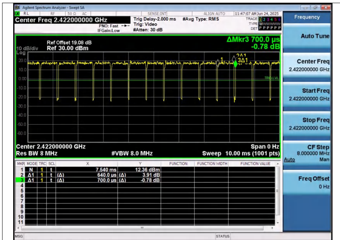
NTNV-11N40MIMO-Ant1-2422
