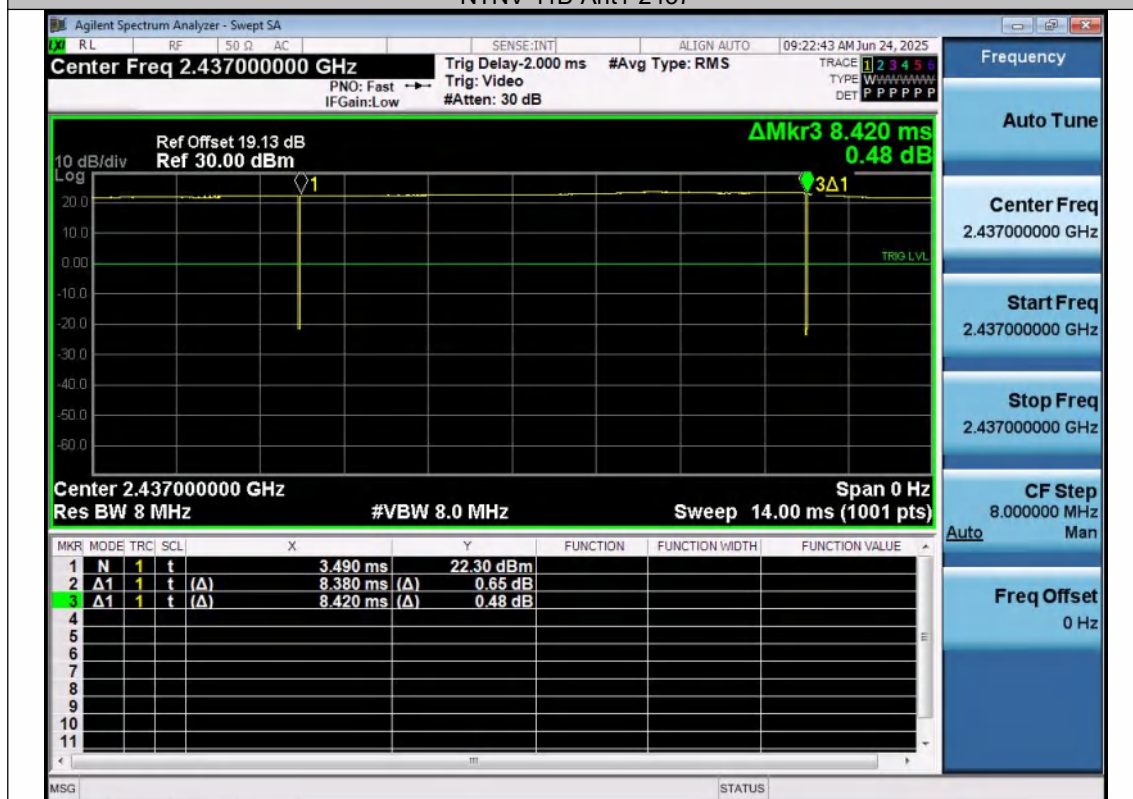
NTNV-11B-Ant2-2437
