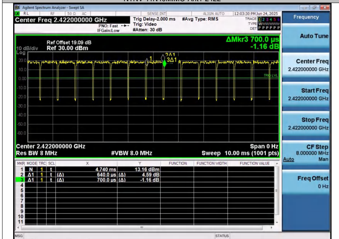
NTNV-11N40MIMO-Ant2-2422
