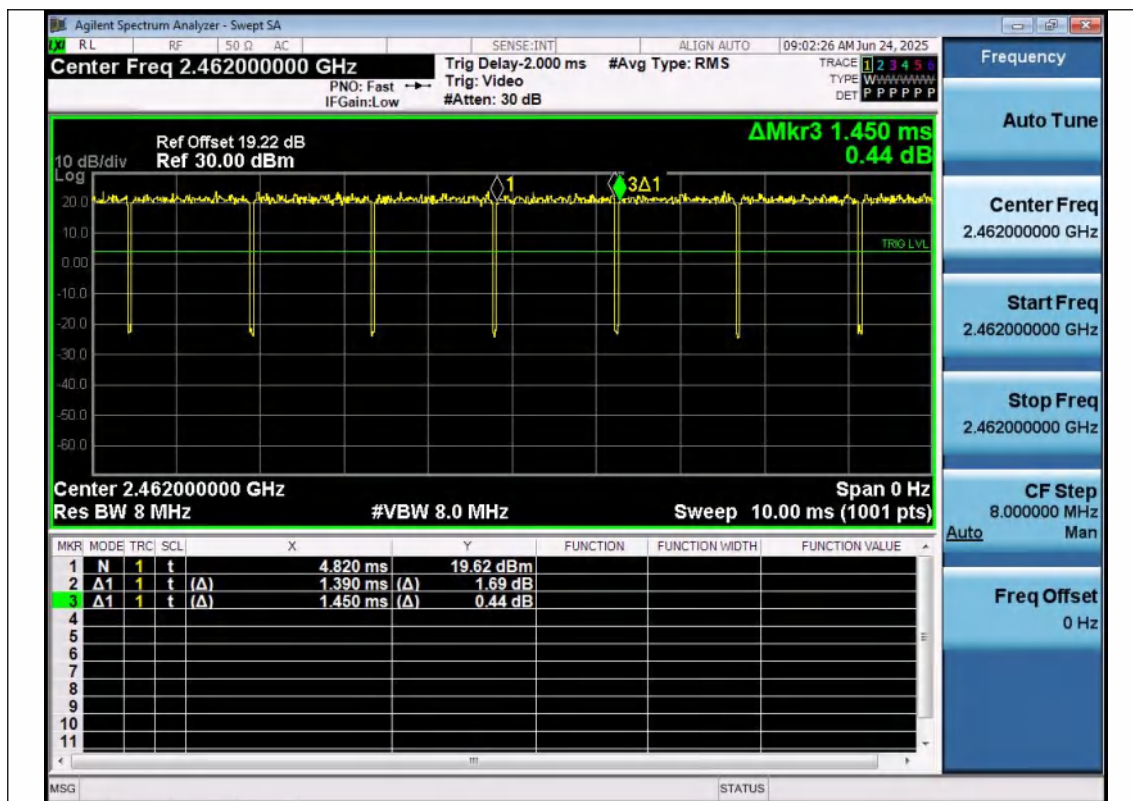
NTNV-11G-Ant1-2462
