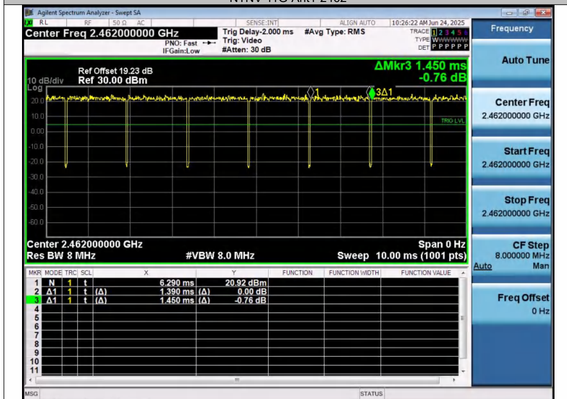
NTNV-11G-Ant2-2462
