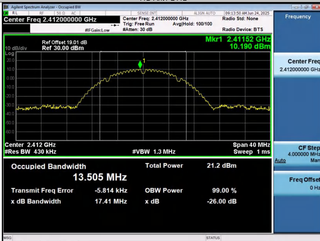
11B-Ant2-2412
