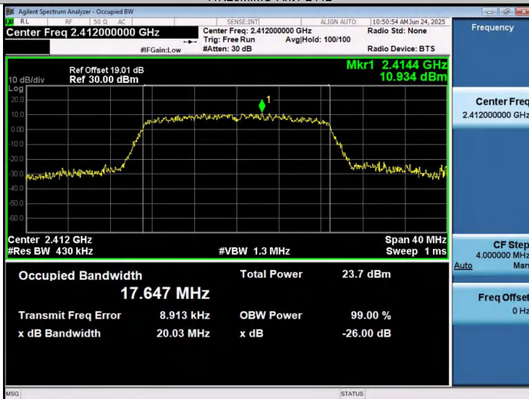
11N20MIMO-Ant2-2412
