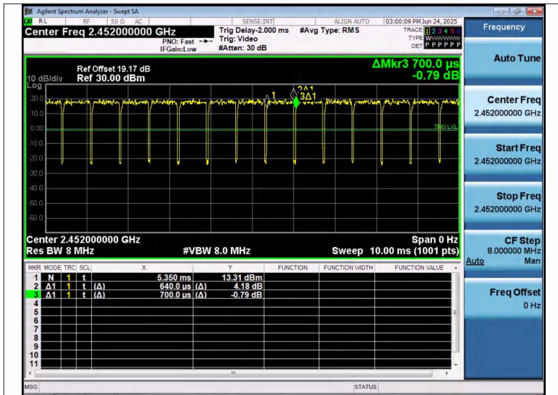
NTNV-11N40MIMO-Ant1-2452
