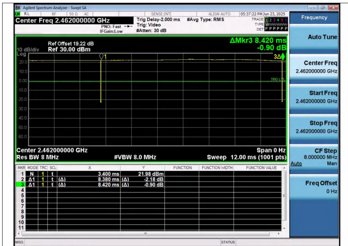
NTNV-11B-Ant1-2462
