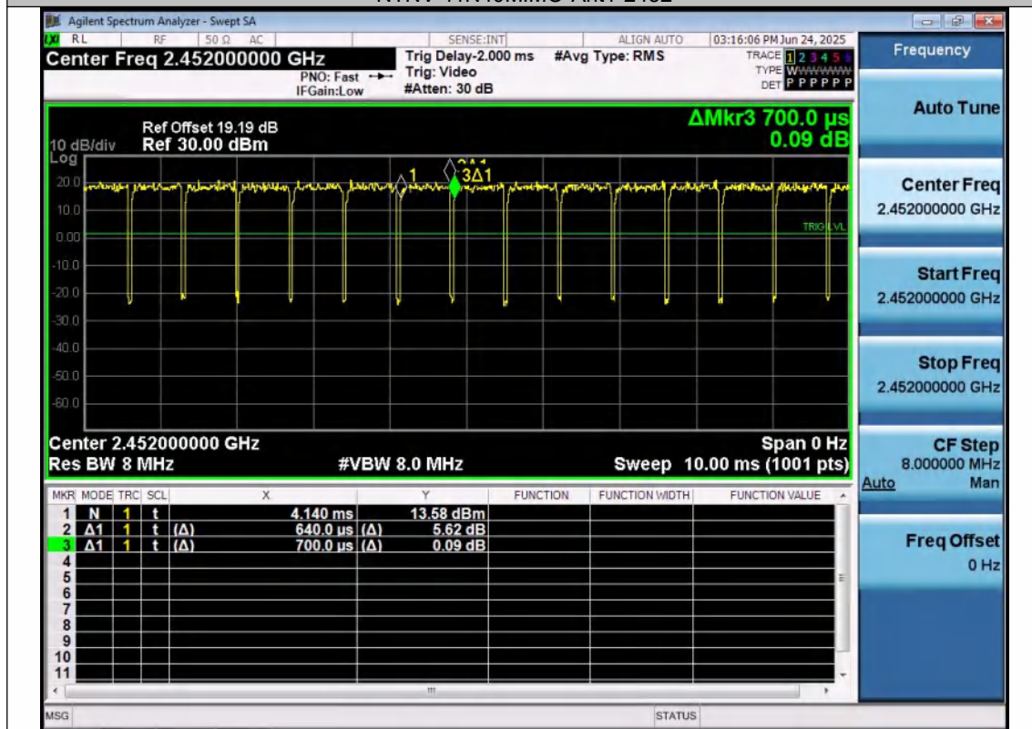
NTNV-11N40MIMO-Ant2-2452
