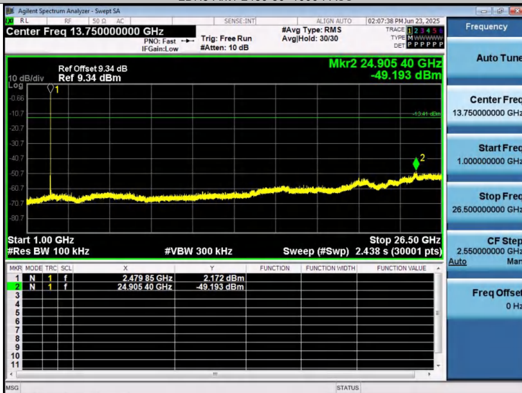
2DH5-Ant1-2480-1000~26500-PASS
