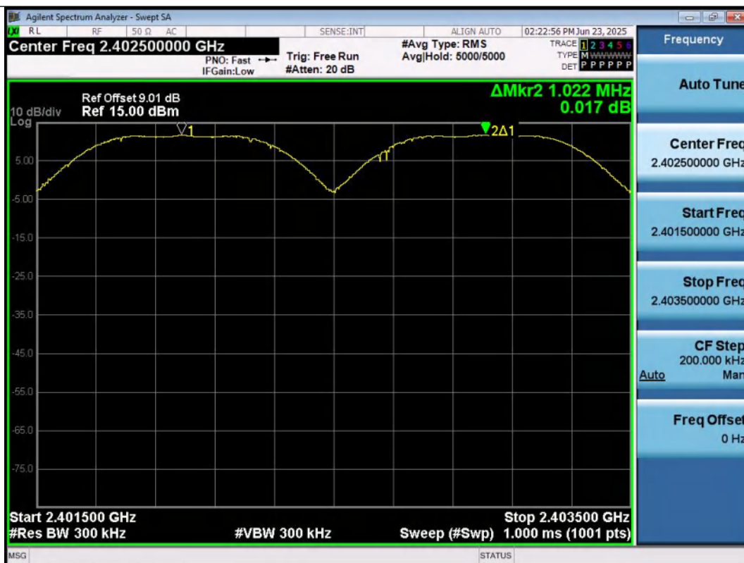
DH5-Ant1-Hop_2402-PASS
