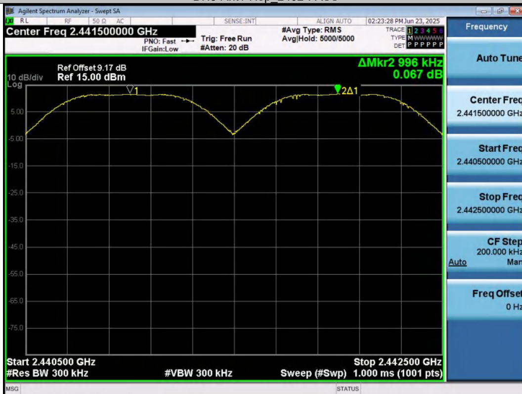
DH5-Ant1-Hop_2441-PASS
