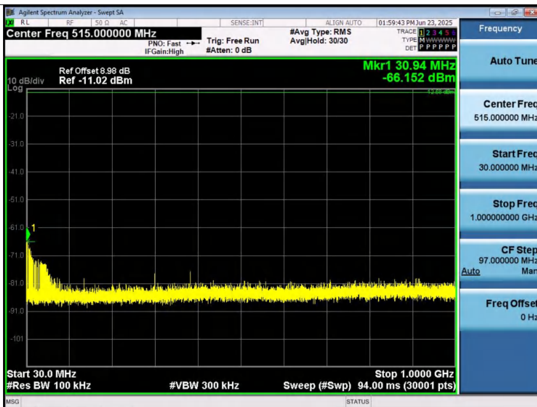
2DH5-Ant1-2402-30~1000-PASS
