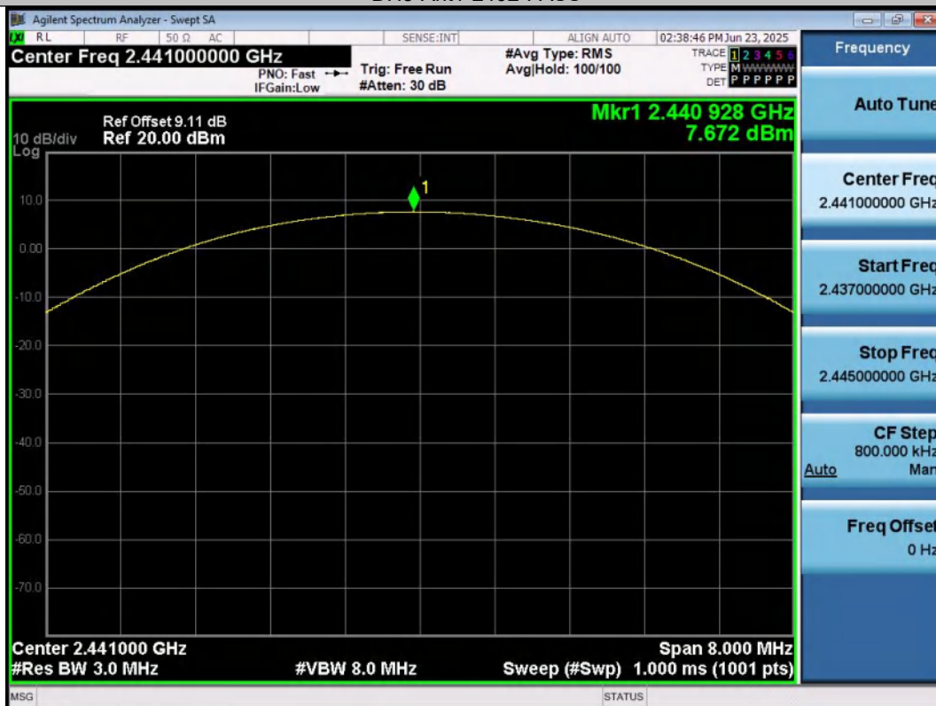
DH5-Ant1-2441-PASS
