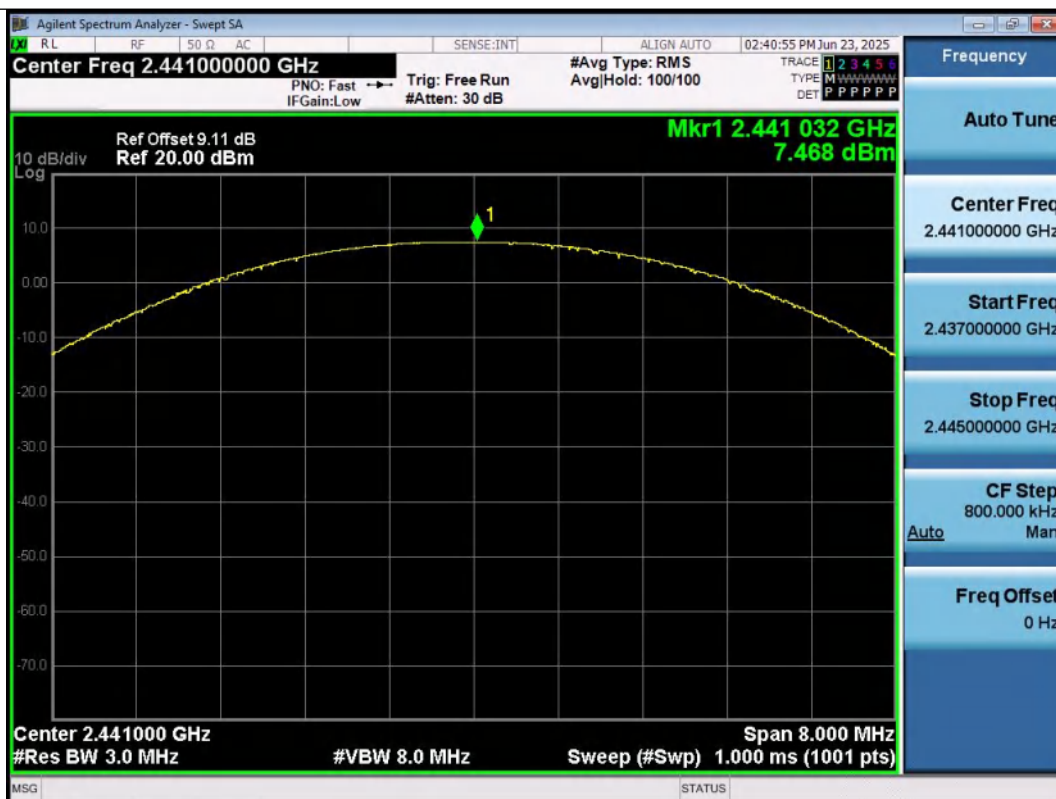
2DH5-Ant1-2441-PASS
