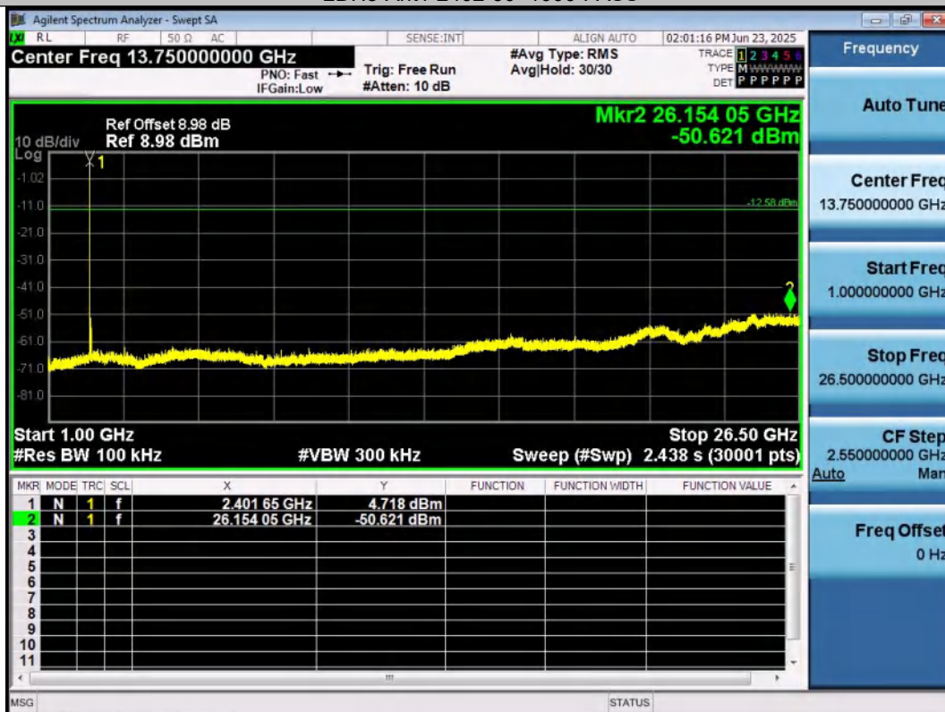
2DH5-Ant1-2402-1000~26500-PASS
