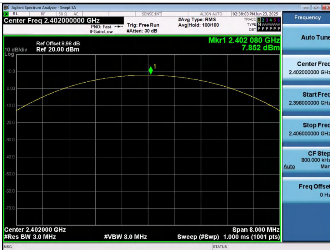
DH5-Ant1-2402-PASS
