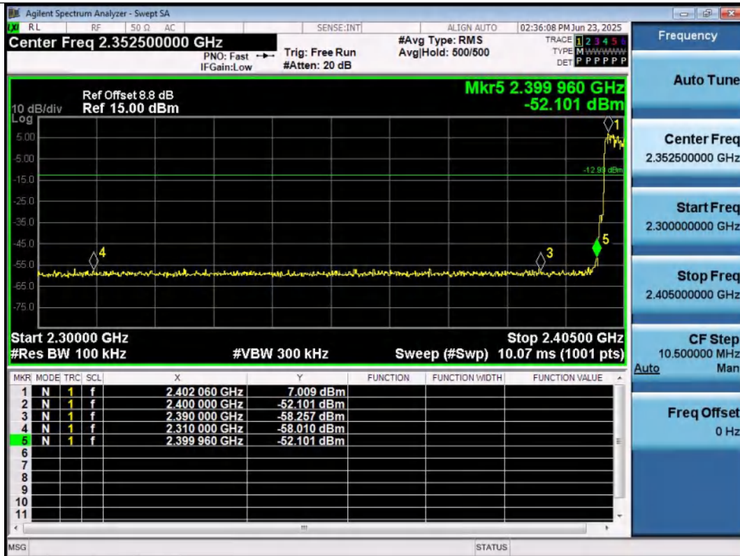
3DH5-Ant1-Hop_2402-PASS
