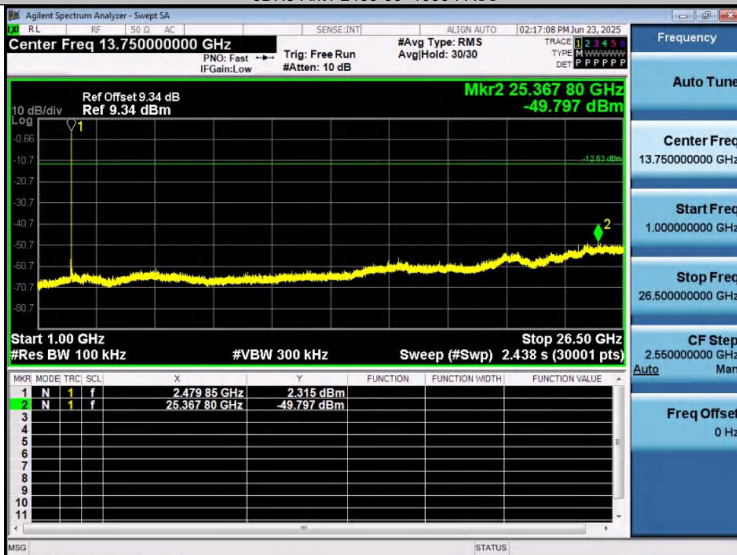
3DH5-Ant1-2480-1000~26500-PASS
