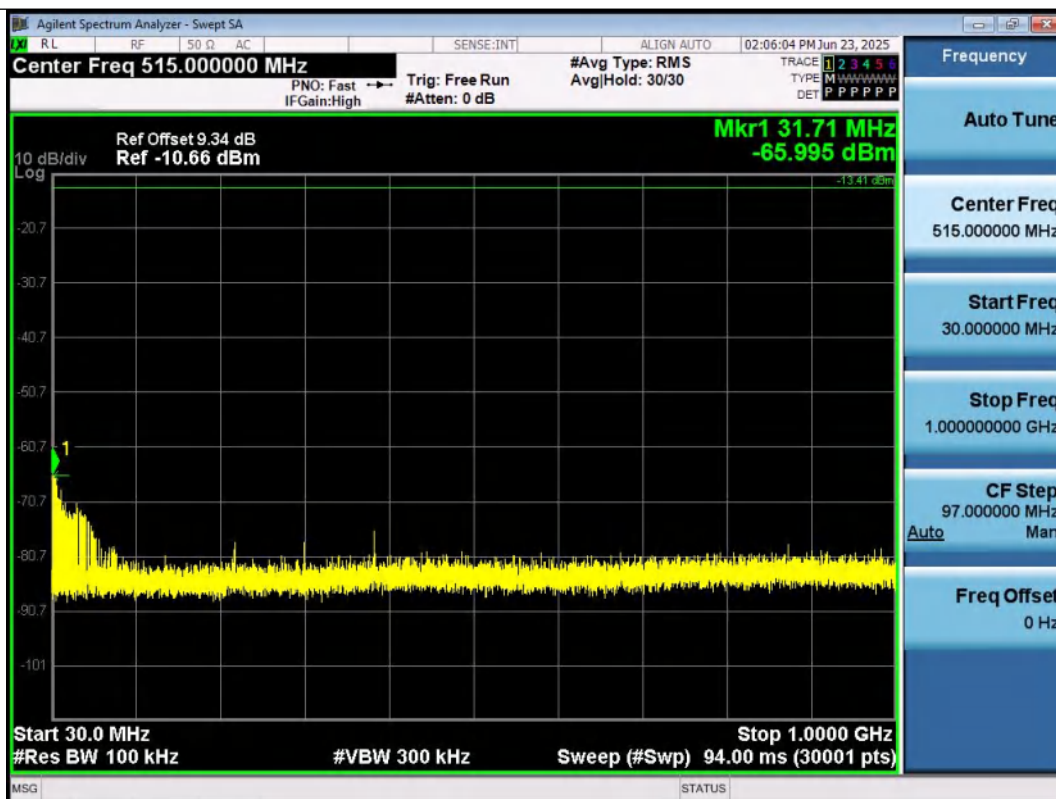
2DH5-Ant1-2480-30~1000-PASS
