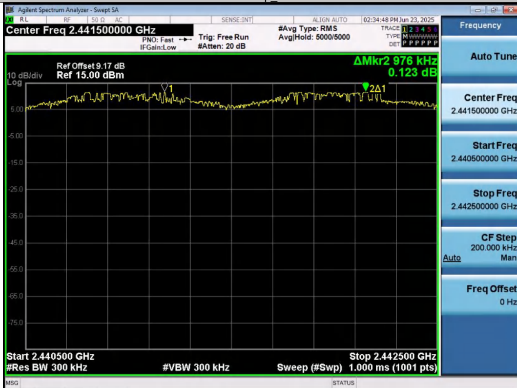
3DH5-Ant1-Hop_2441-PASS
