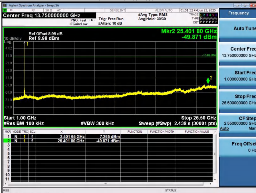
DH5-Ant1-2402-1000~26500-PASS
