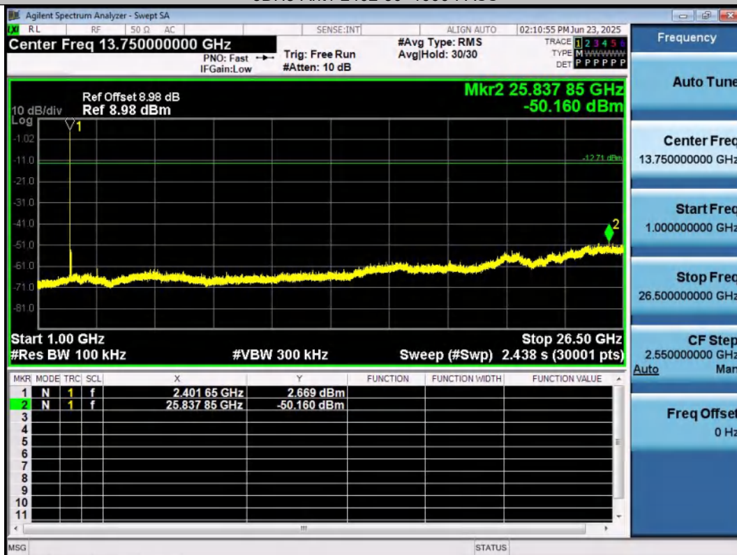
3DH5-Ant1-2402-1000~26500-PASS
