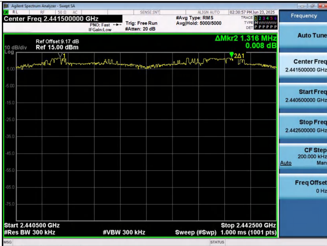
2DH5-Ant1-Hop_2441-PASS
