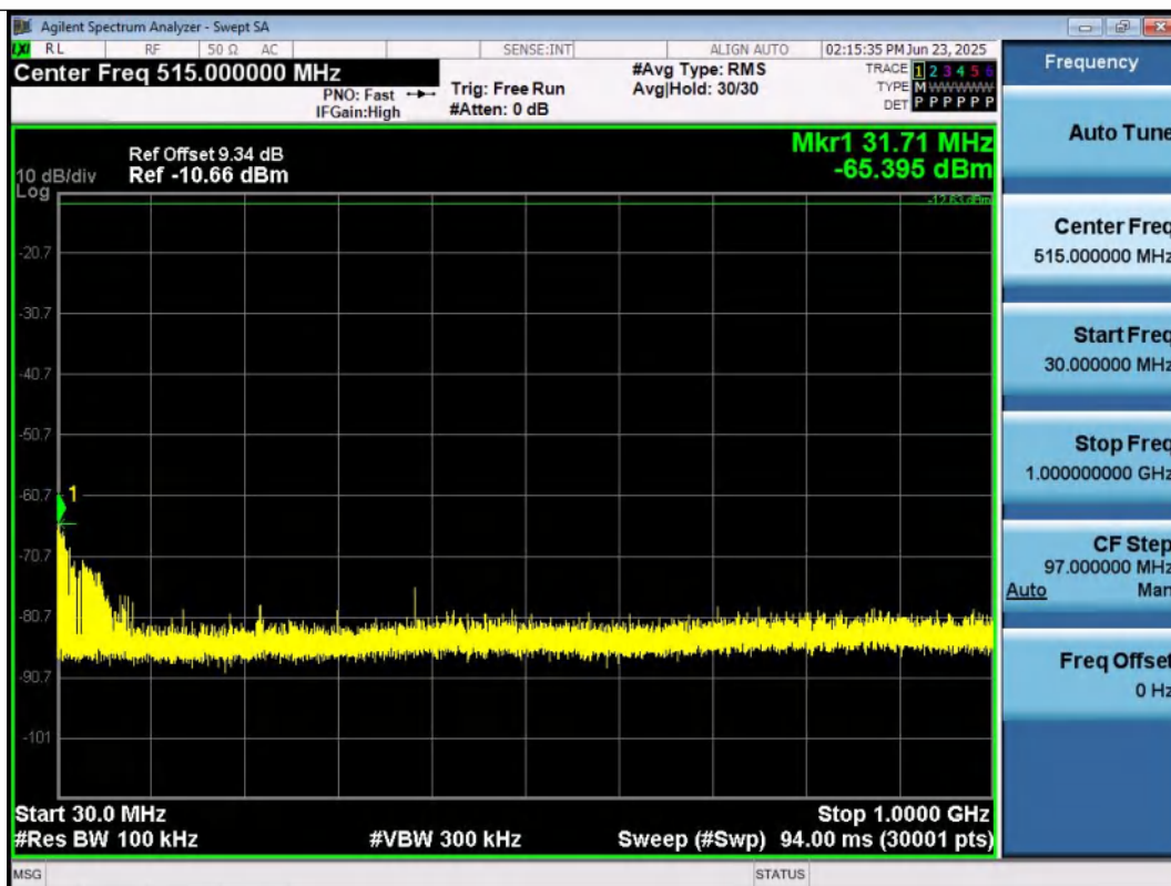
3DH5-Ant1-2480-30~1000-PASS
