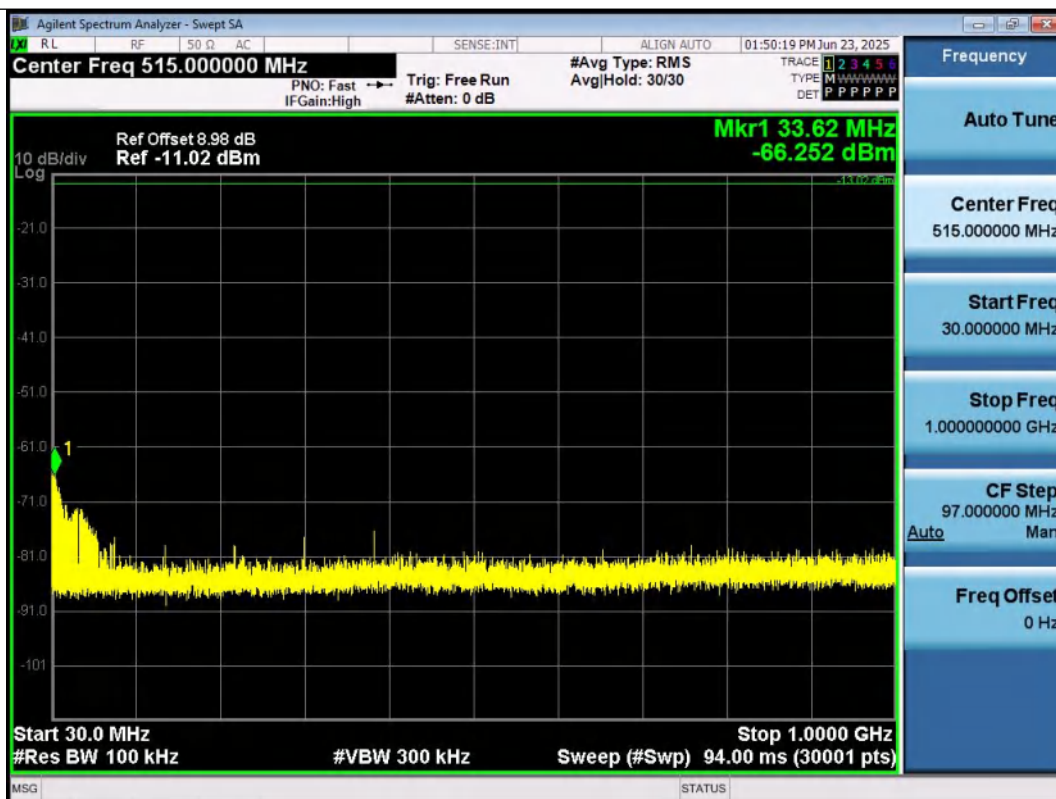
DH5-Ant1-2402-30~1000-PASS
