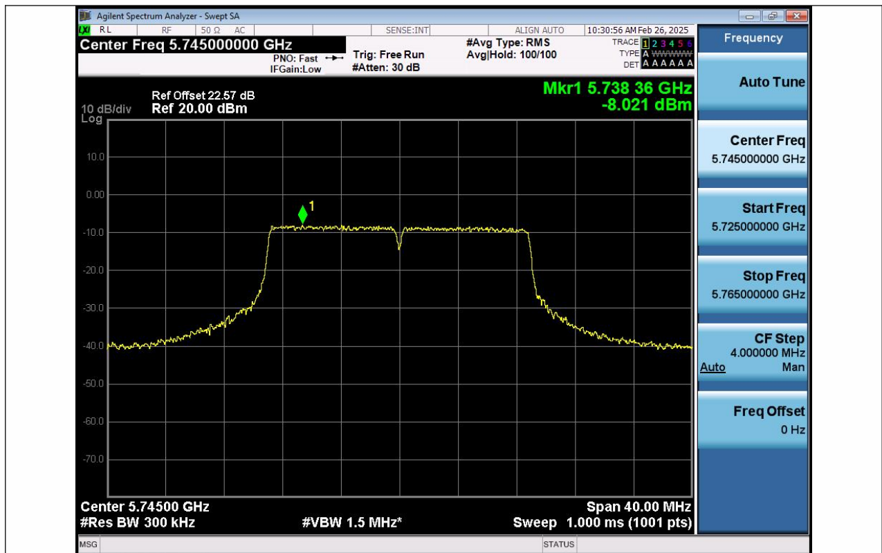
11AC20SISO-Ant1-5745-PASS
