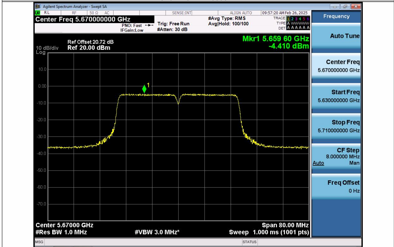
11AC40SISO-Ant1-5670-PASS
