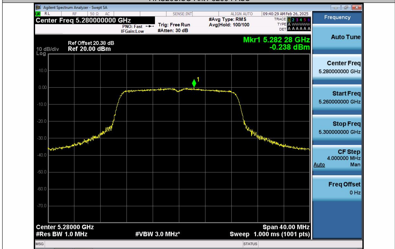
11AC20SISO-Ant1-5280-PASS
