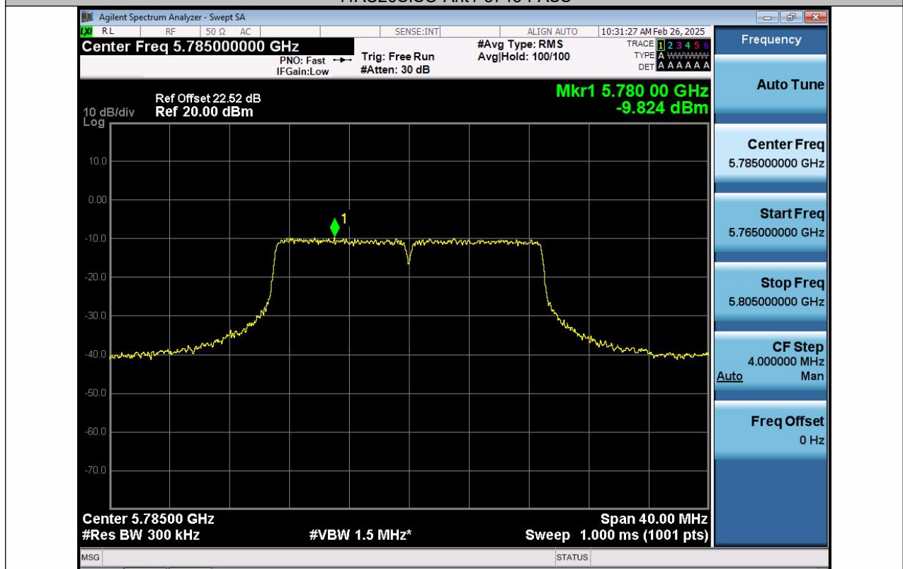
11AC20SISO-Ant1-5785-PASS
