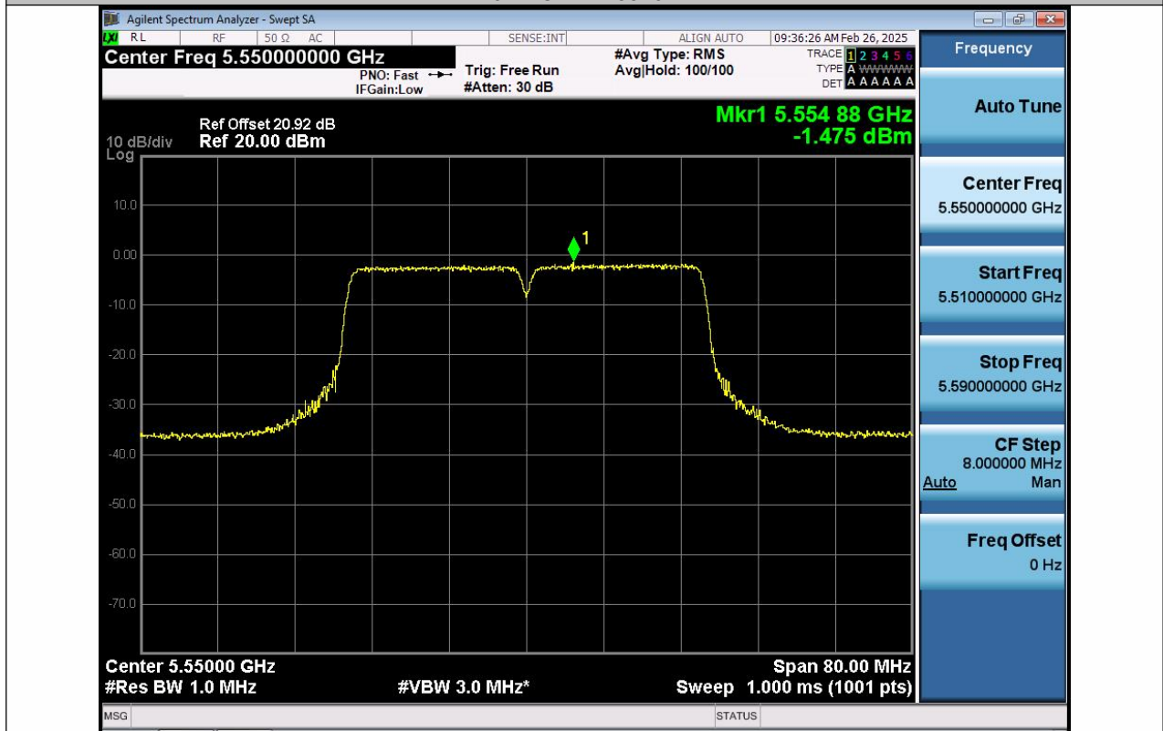
11N40SISO-Ant1-5550-PASS
