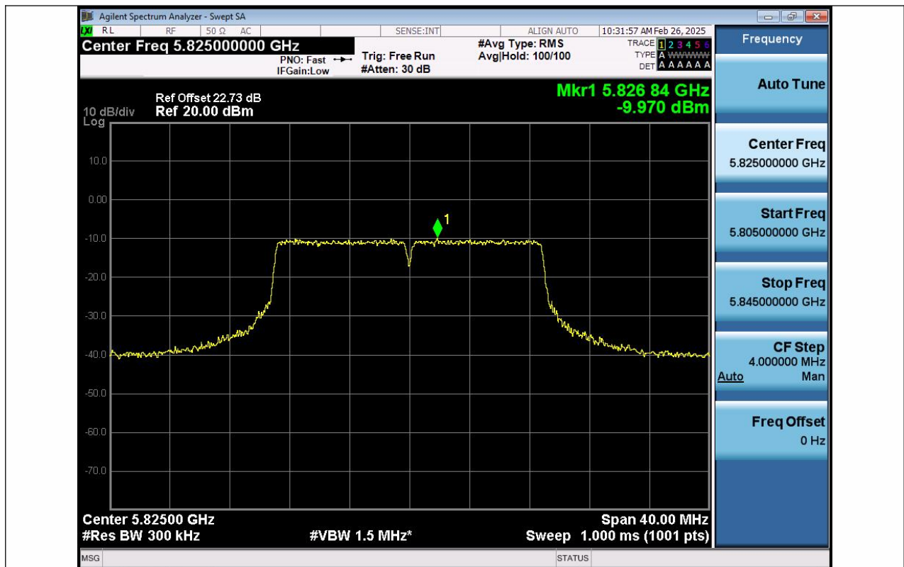
11AC20SISO-Ant1-5825-PASS
