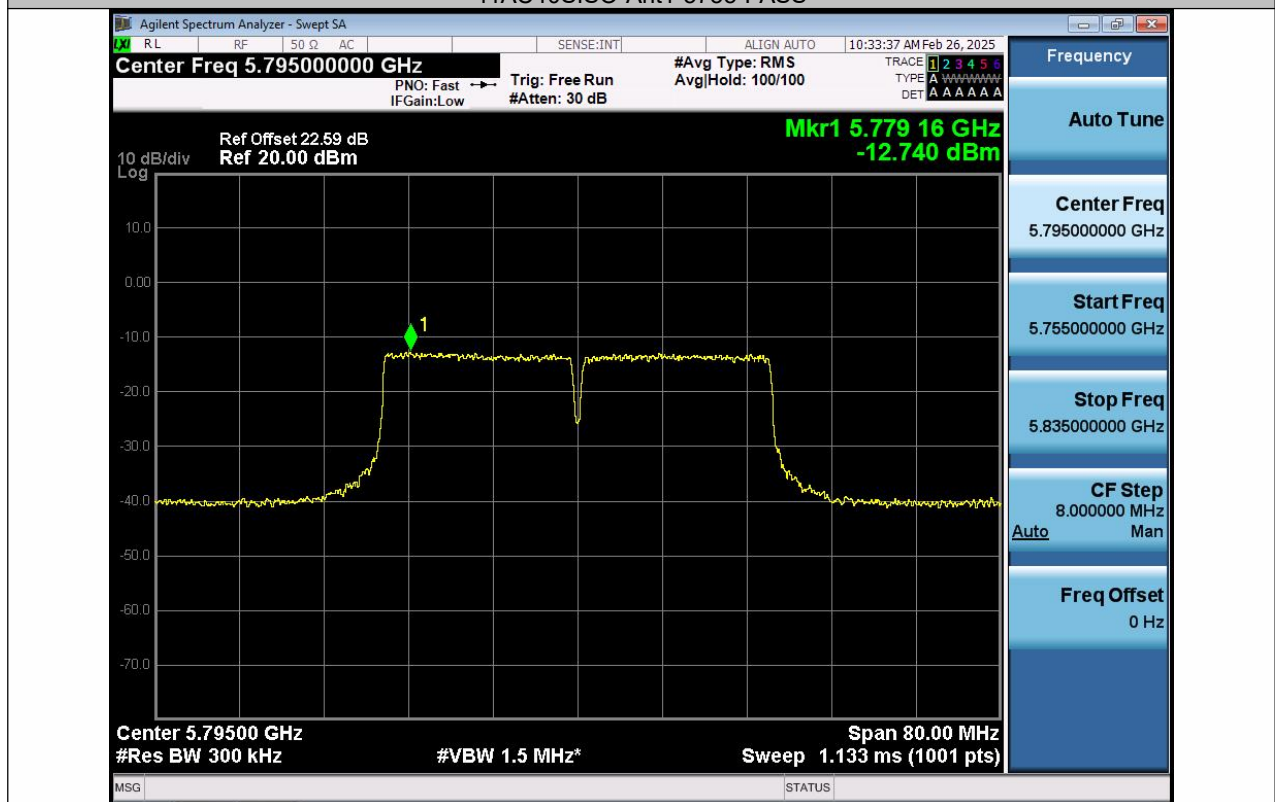
11AC40SISO-Ant1-5795-PASS
