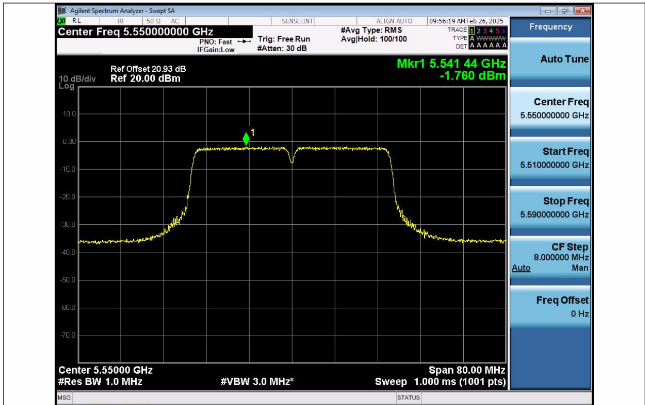
11AC40SISO-Ant1-5550-PASS
