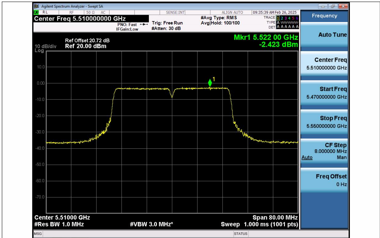
11N40SISO-Ant1-5510-PASS
