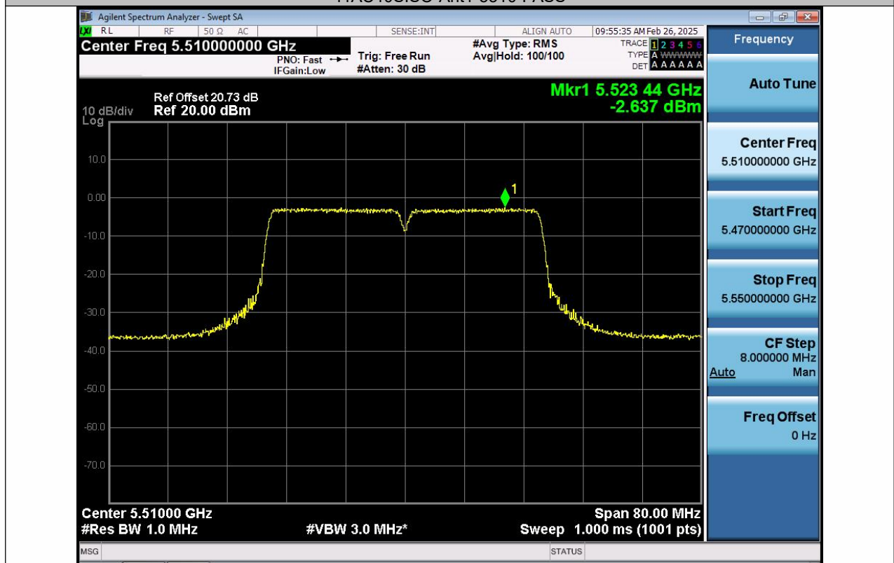
11AC40SISO-Ant1-5510-PASS
