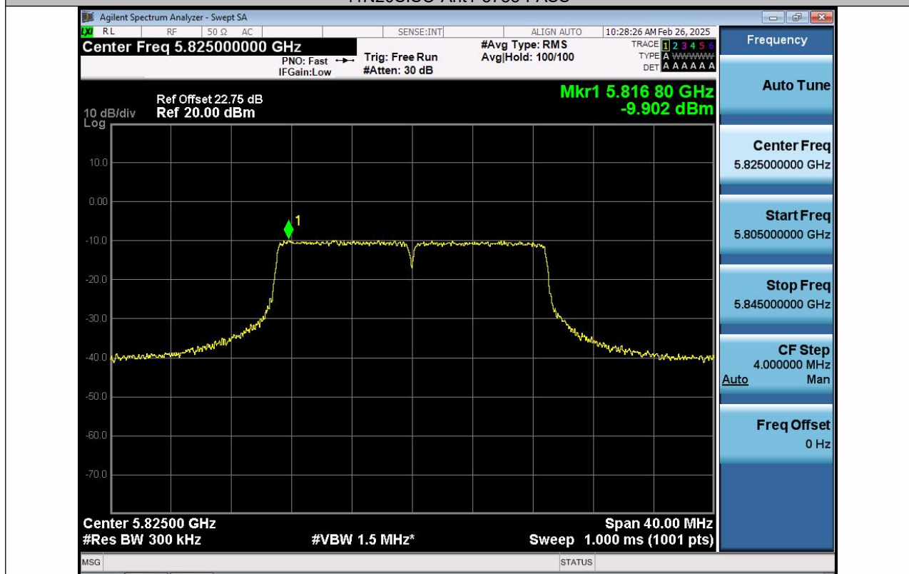
11N20SISO-Ant1-5825-PASS
