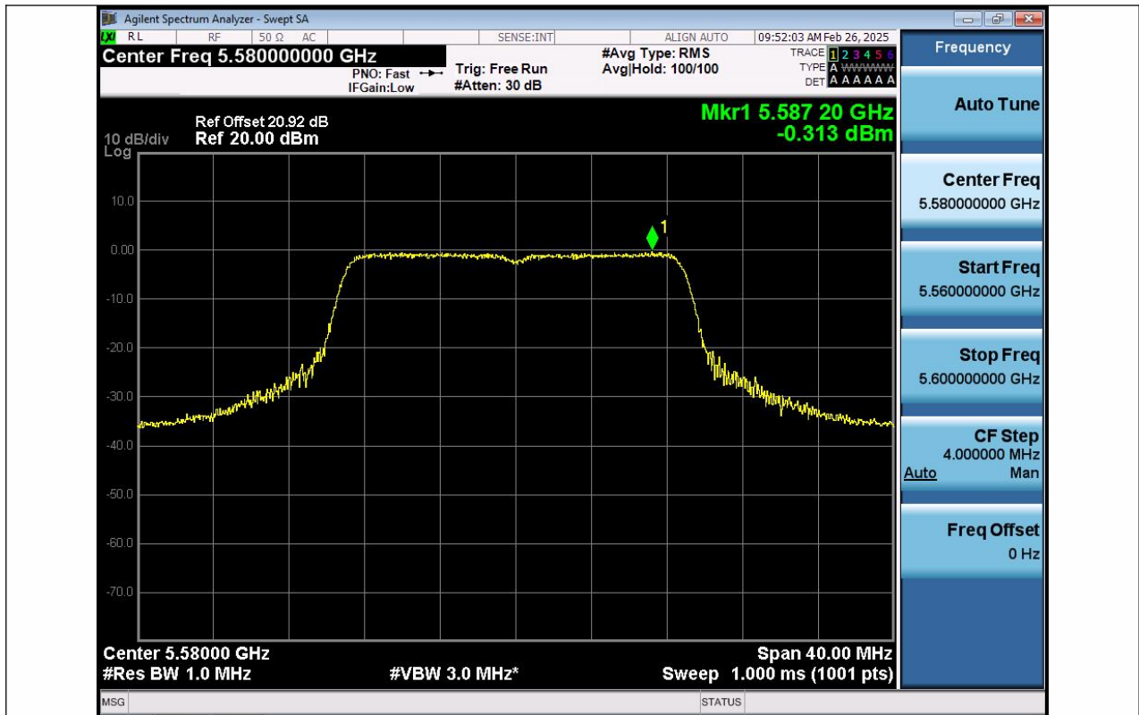
11AC20SISO-Ant1-5580-PASS
