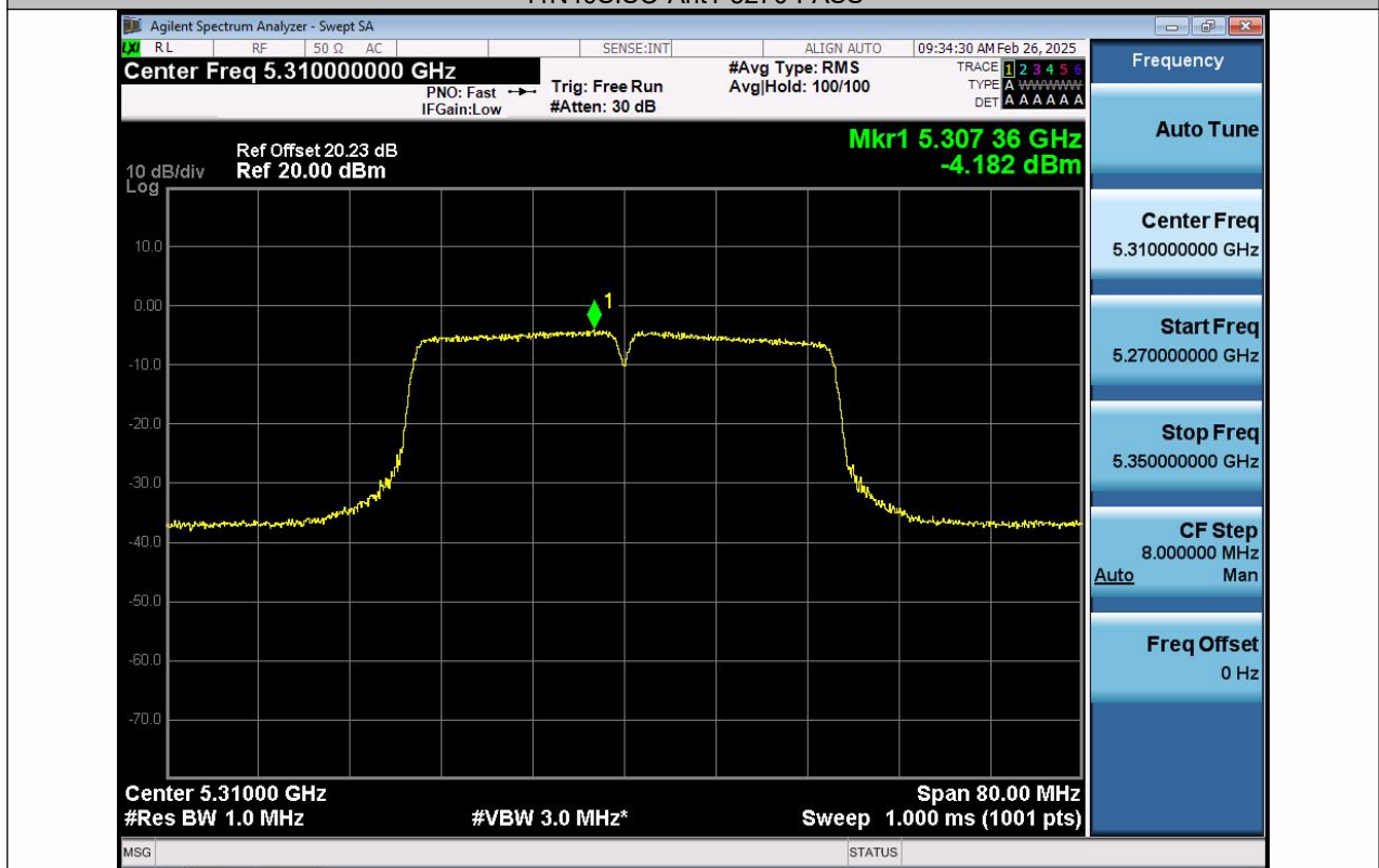
11N40SISO-Ant1-5310-PASS
