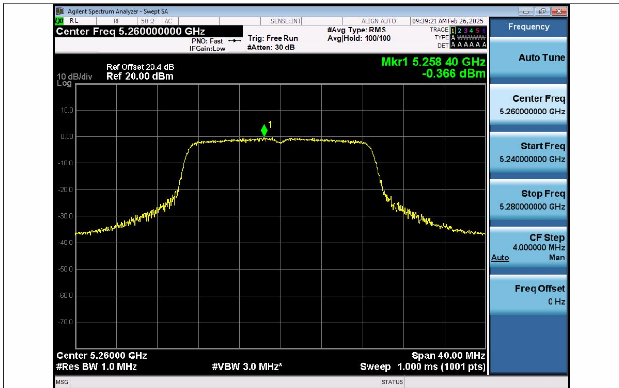
11AC20SISO-Ant1-5260-PASS
