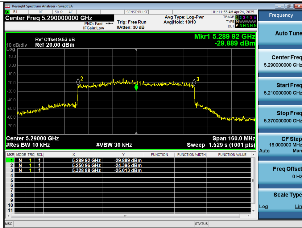
Freq. Stability 0C 12V ax80 5290MHz Ant1 0 Minutes
