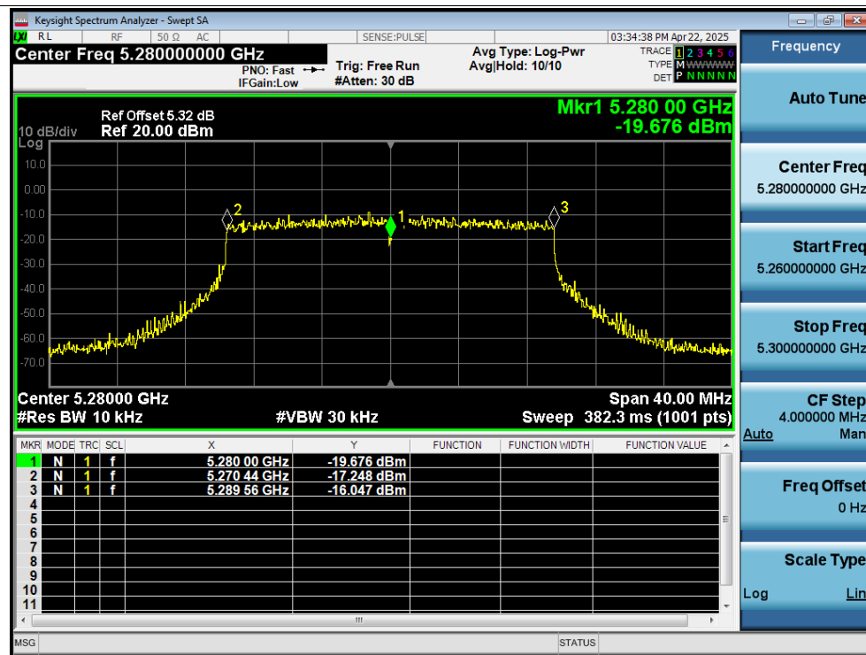
Freq. Stability -10C 12V ax20 5280MHz Ant2 0 Minutes
