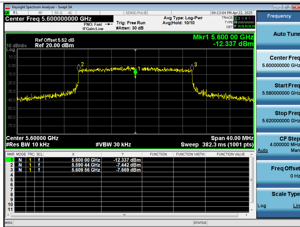
Freq. Stability -10C 12V ax20 5600MHz Ant2 0 Minutes
