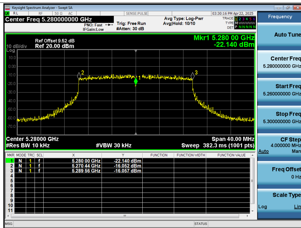
Freq. Stability -10C 12V ax20 5280MHz Ant1 0 Minutes
