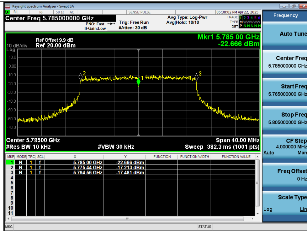
Freq. Stability -10C 12V ax20 5785MHz Ant1 0 Minutes
