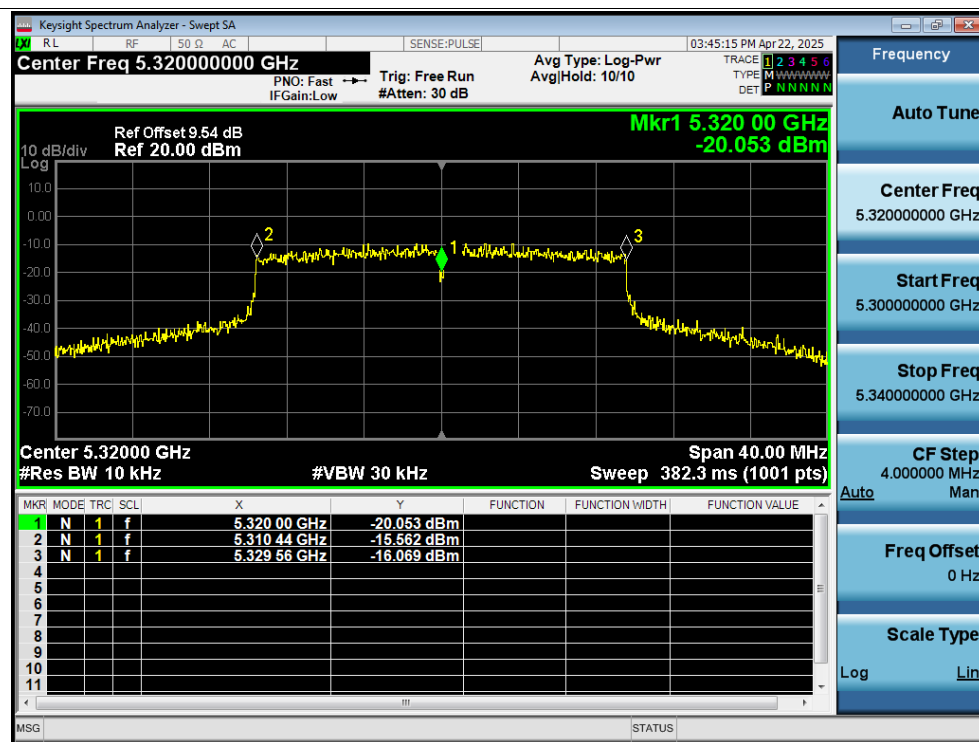
Freq. Stability 40C 12V ax20 5320MHz Ant1 0 Minutes
