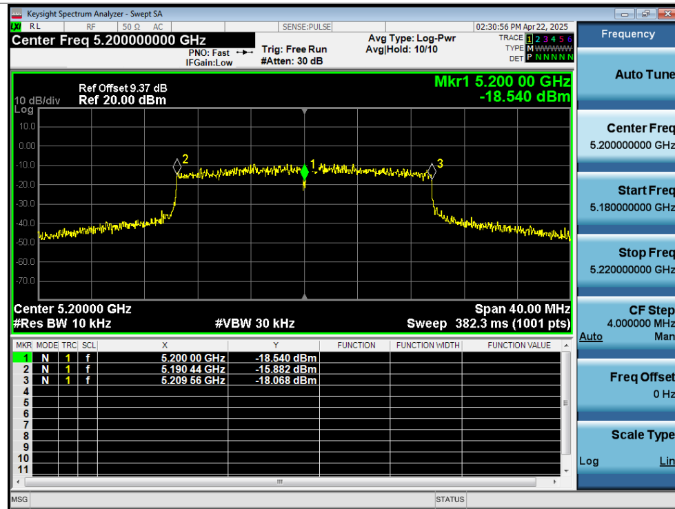
Freq. Stability -10C 12V ax20 5200MHz Ant1 0 Minutes
