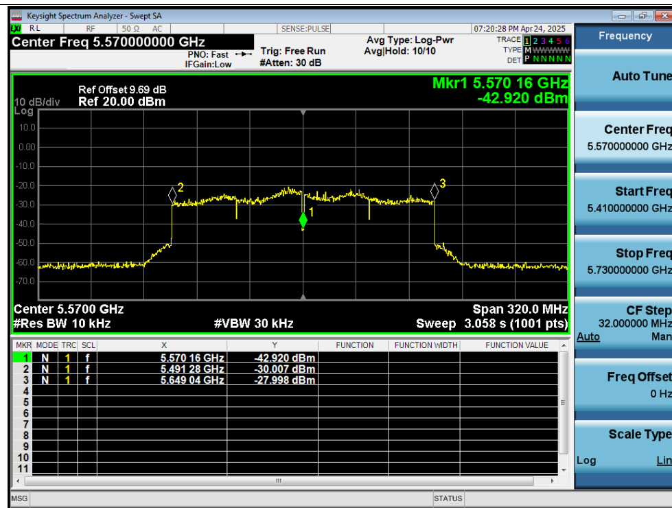
Freq. Stability 10C 12V ax160 5570MHz Ant1 0 Minutes
