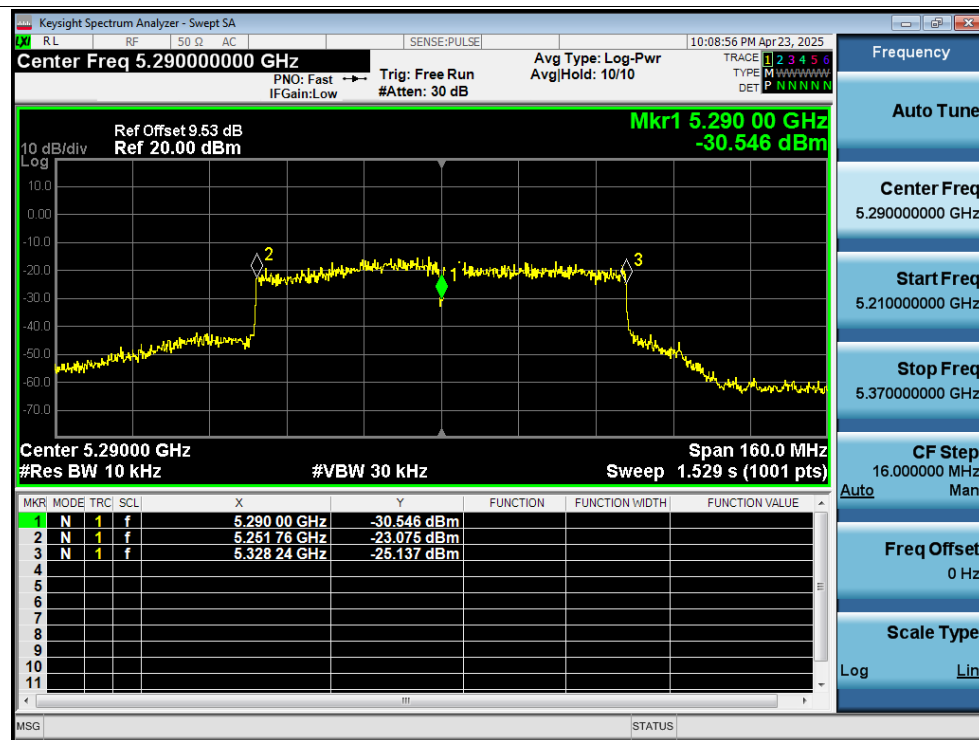
Freq. Stability -10C 12V ac80 5290MHz Ant1 0 Minutes
