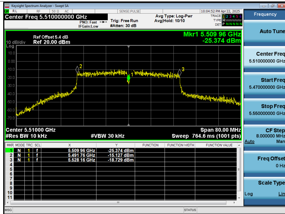
Freq. Stability -10C 12V ac40 5510MHz Ant3 0 Minutes
