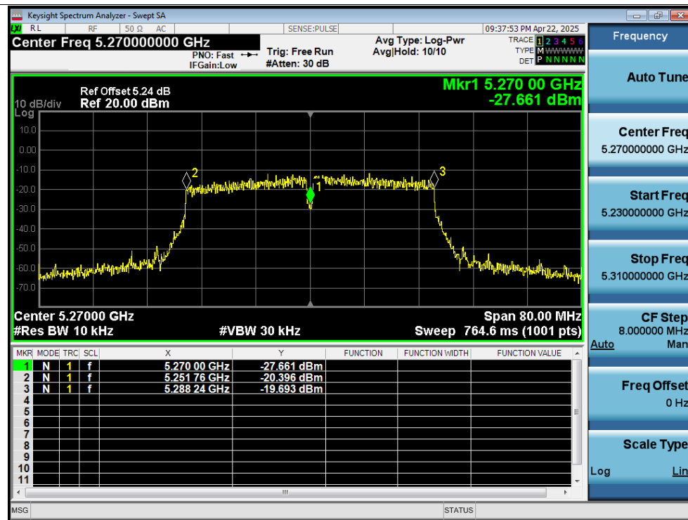
Freq. Stability 40C 12V ac40 5270MHz Ant3 0 Minutes
