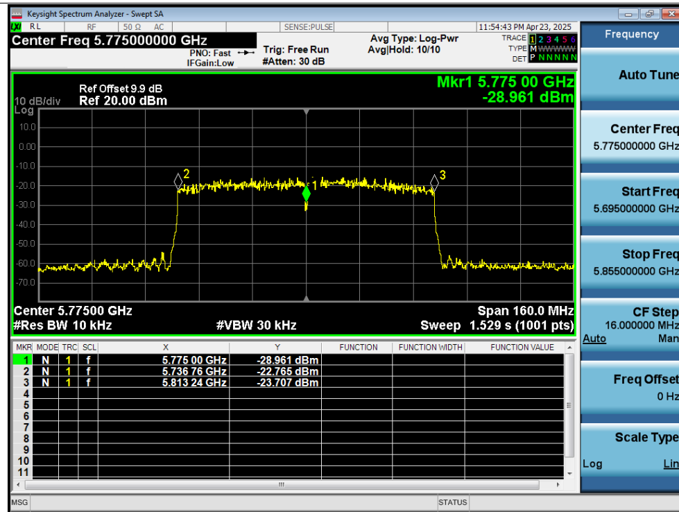
Freq. Stability -10C 12V ac80 5775MHz Ant1 0 Minutes
