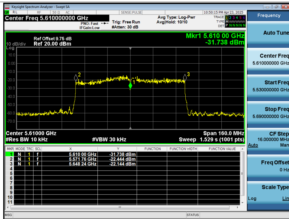
Freq. Stability -10C 12V ac80 5610MHz Ant1 0 Minutes
