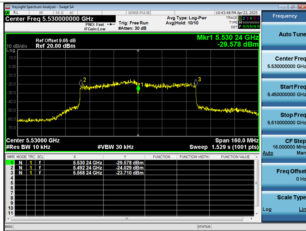
Freq. Stability -10C 12V ac80 5530MHz Ant1 0 Minutes
