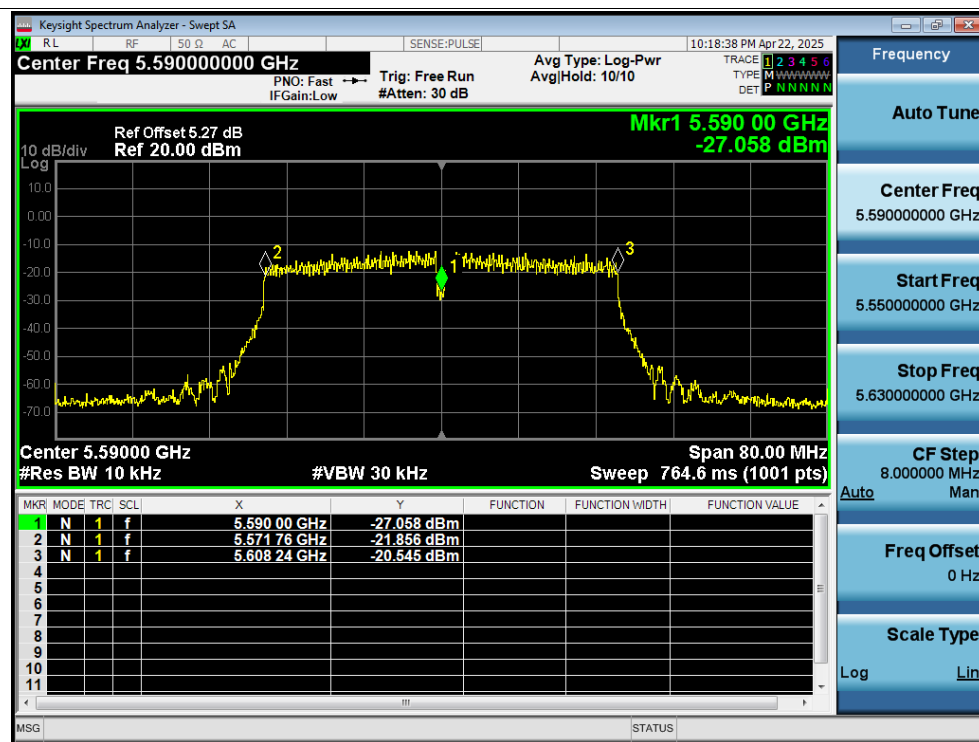
Freq. Stability 20C 13.8V ac40 5590MHz Ant3 0 Minutes
