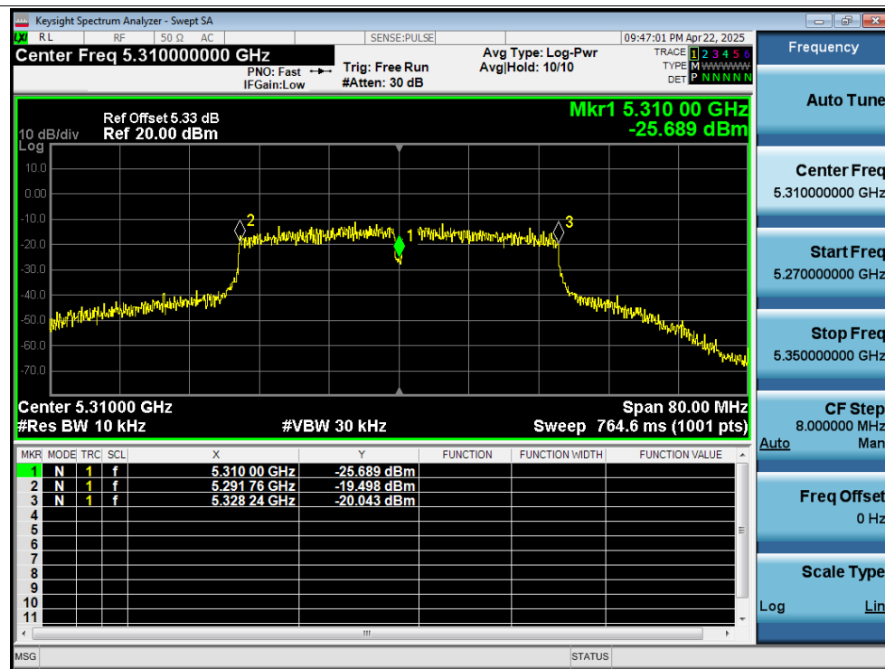
Freq. Stability -10C 12V ac40 5310MHz Ant2 0 Minutes
