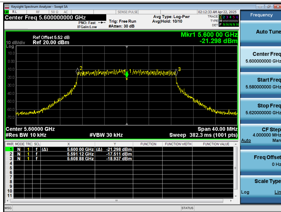
Freq. Stability -10C 12V ac20 5600MHz Ant2 0 Minutes
