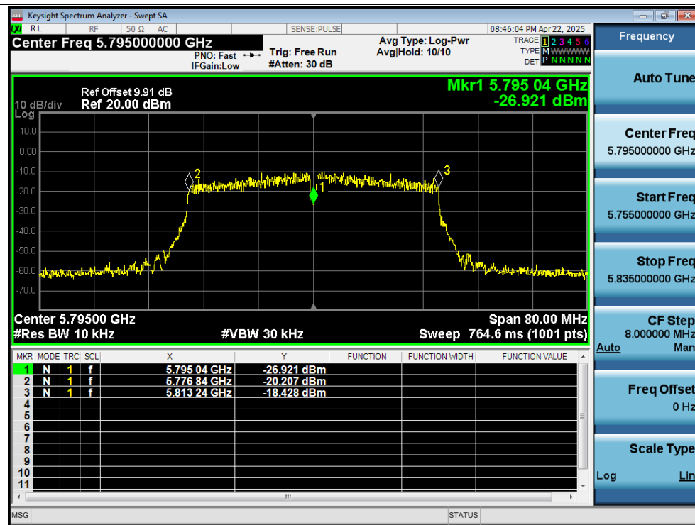
Freq. Stability 40C 12V n40 5795MHz Ant1 0 Minutes
