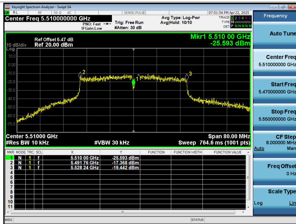
Freq. Stability 10C 12V n40 5510MHz Ant2 0 Minutes
