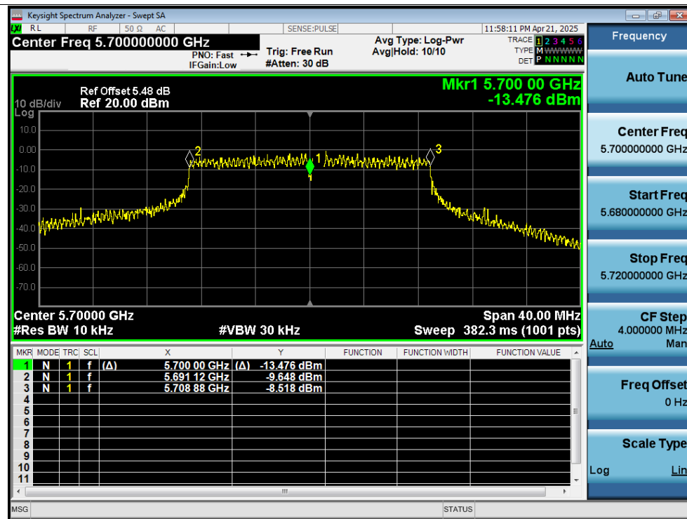
Freq. Stability 0C 12V n20 5700MHz Ant3 -18 Minutes
