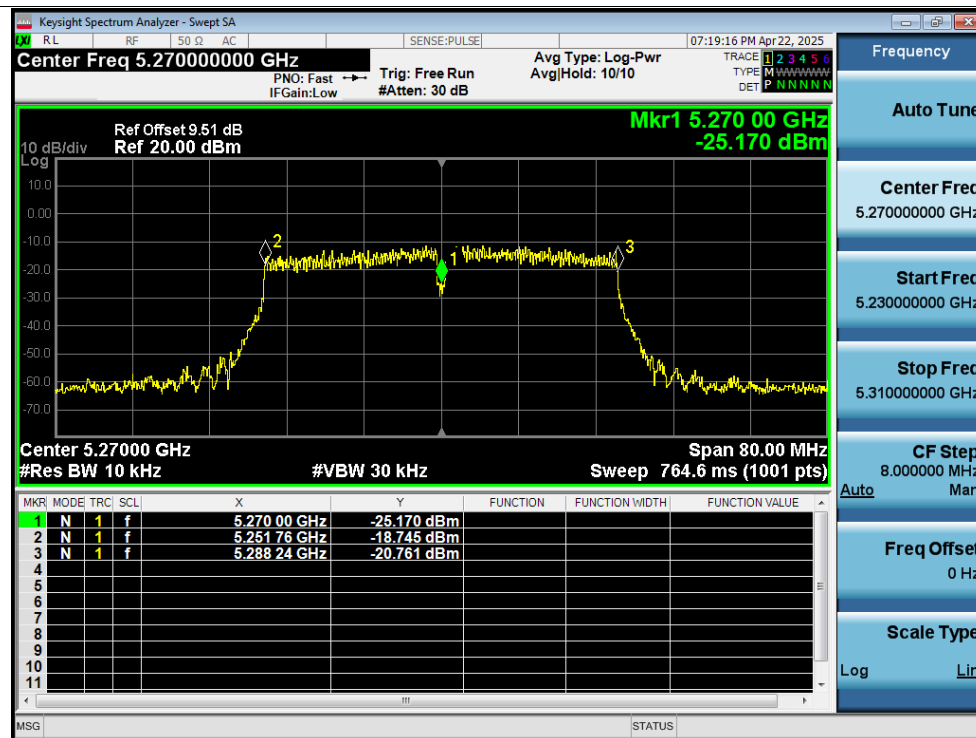
Freq. Stability 20C 13.8V n40 5270MHz Ant1 0 Minutes
