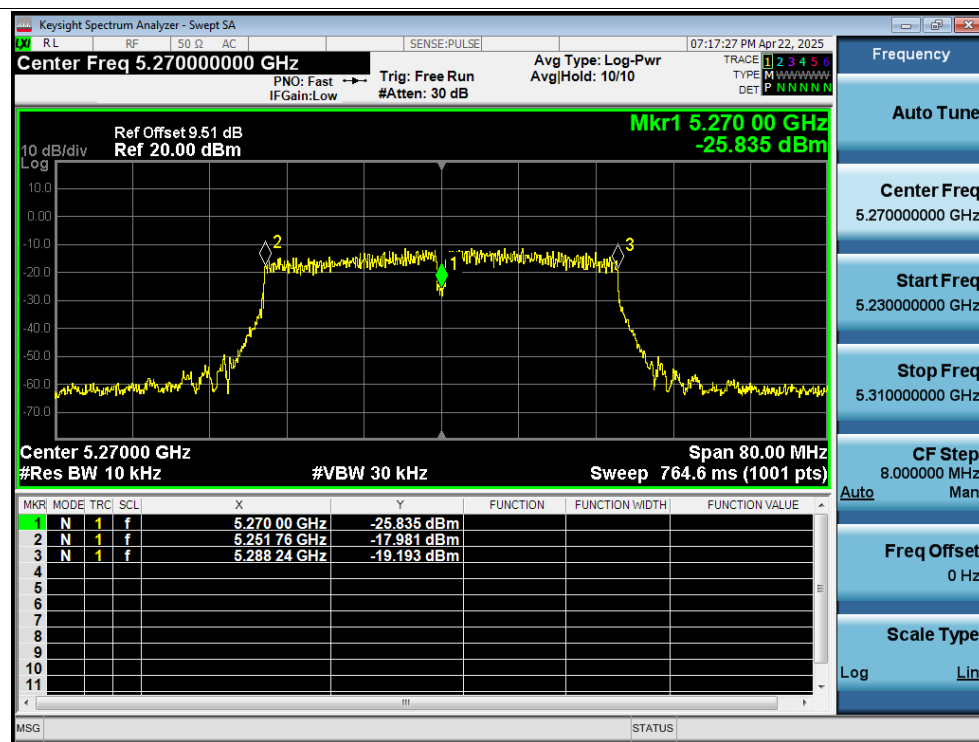
Freq. Stability 20C 10.2V n40 5270MHz Ant1 0 Minutes
