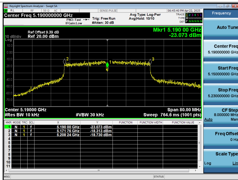
Freq. Stability 40C 12V n40 5190MHz Ant1 0 Minutes
