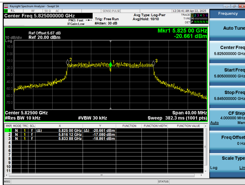
Freq. Stability 50C 12V n20 5825MHz Ant2 0 Minutes
