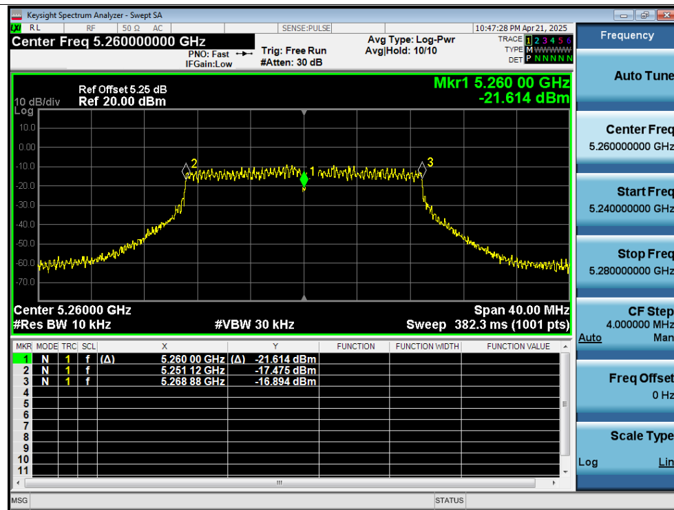
Freq. Stability 50C 12V n20 5260MHz Ant3 0 Minutes
