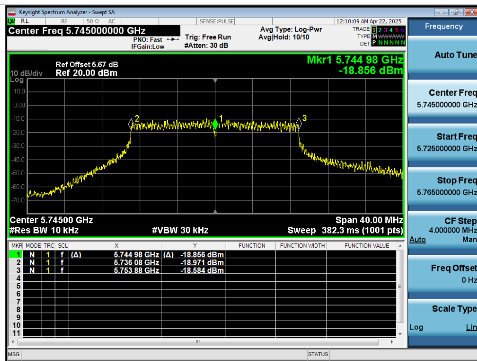
Freq. Stability 30C 12V n20 5745MHz Ant2 0 Minutes
