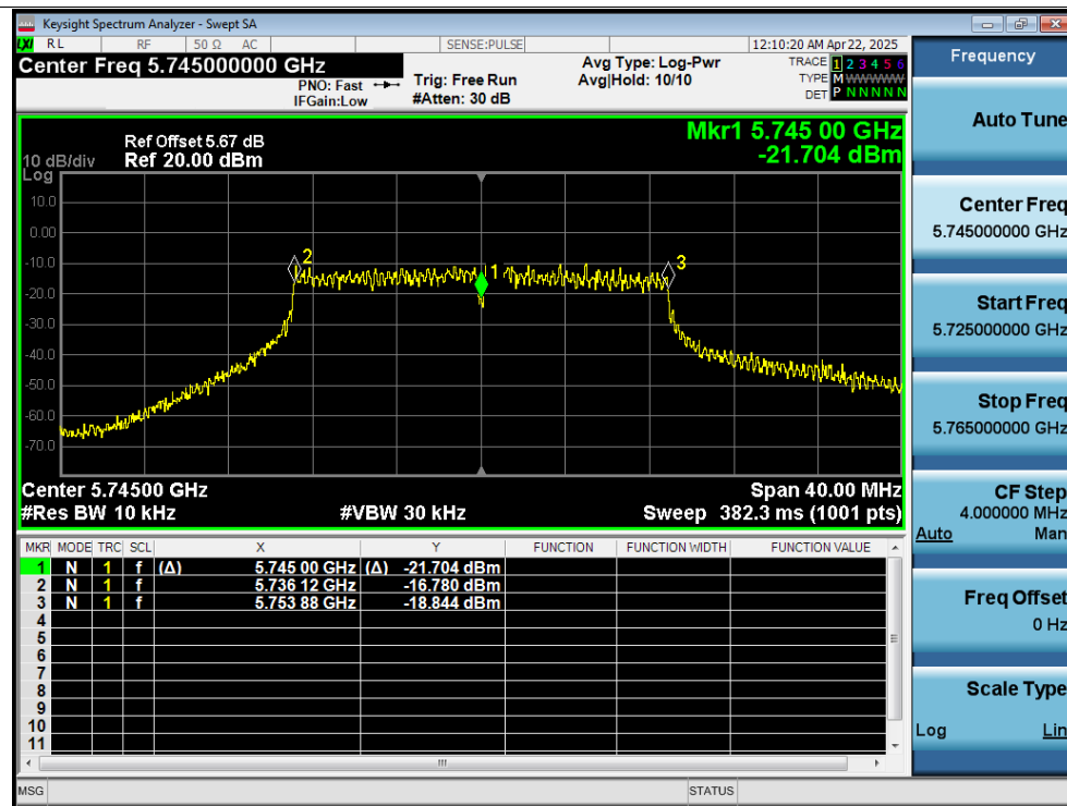
Freq. Stability 50C 12V n20 5745MHz Ant2 0 Minutes
