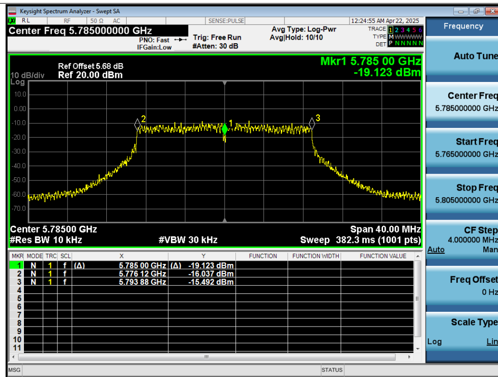
Freq. Stability 30C 12V n20 5785MHz Ant2 0 Minutes
