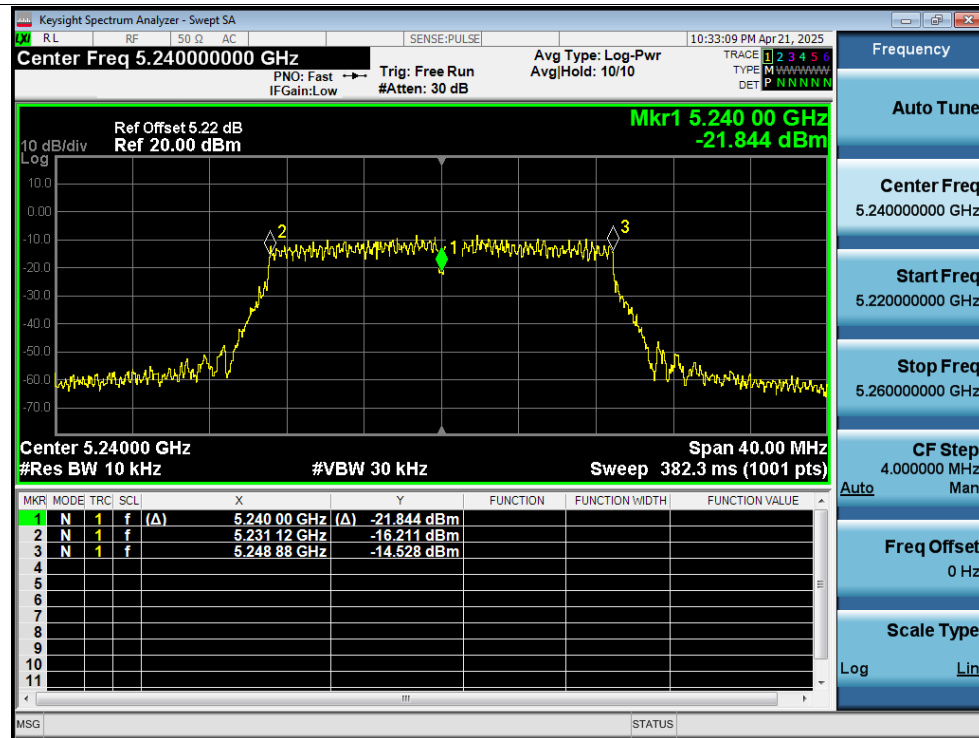
Freq. Stability 20C 12V n20 5240MHz Ant3 0 Minutes
