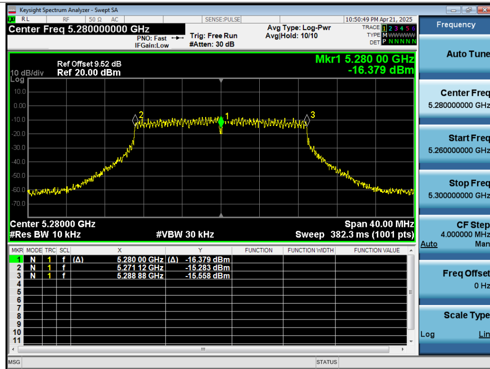
Freq. Stability 20C 12V n20 5280MHz Ant1 0 Minutes
