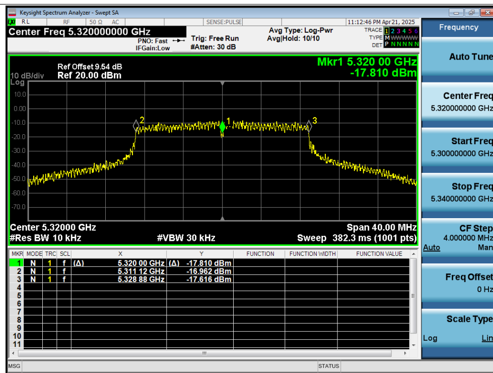
Freq. Stability 0C 12V n20 5320MHz Ant1 0 Minutes
