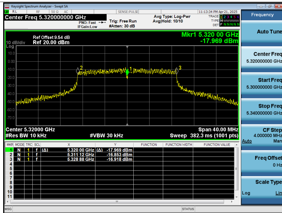
Freq. Stability 50C 12V n20 5320MHz Ant1 0 Minutes
