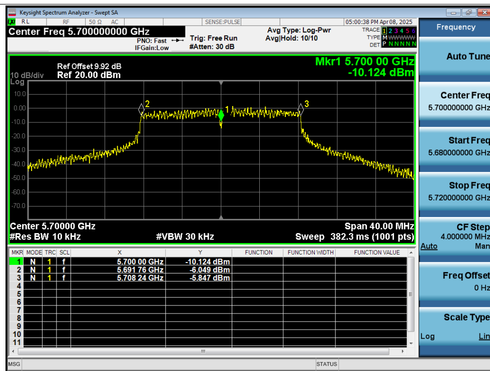
Freq. Stability 0C 12V a 5700MHz Ant1 0 Minutes
