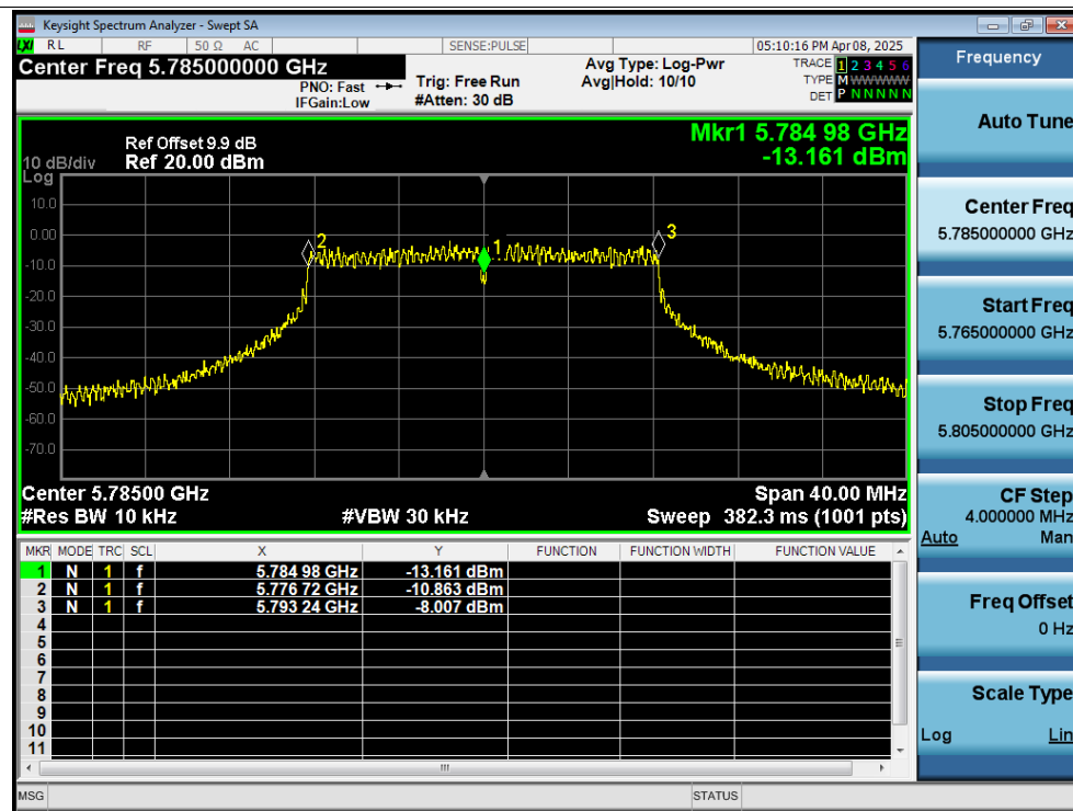
Freq. Stability 0C 12V a 5785MHz Ant1 0 Minutes
