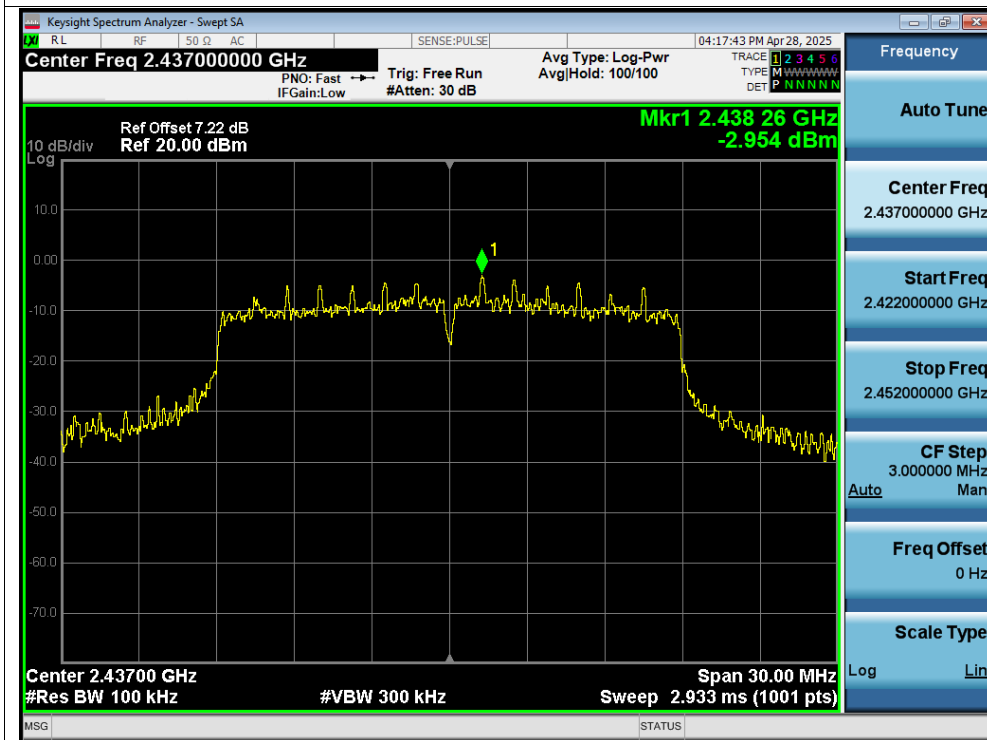
Tx. Spurious NVNT ac20 2437MHz Ant1 Emission
