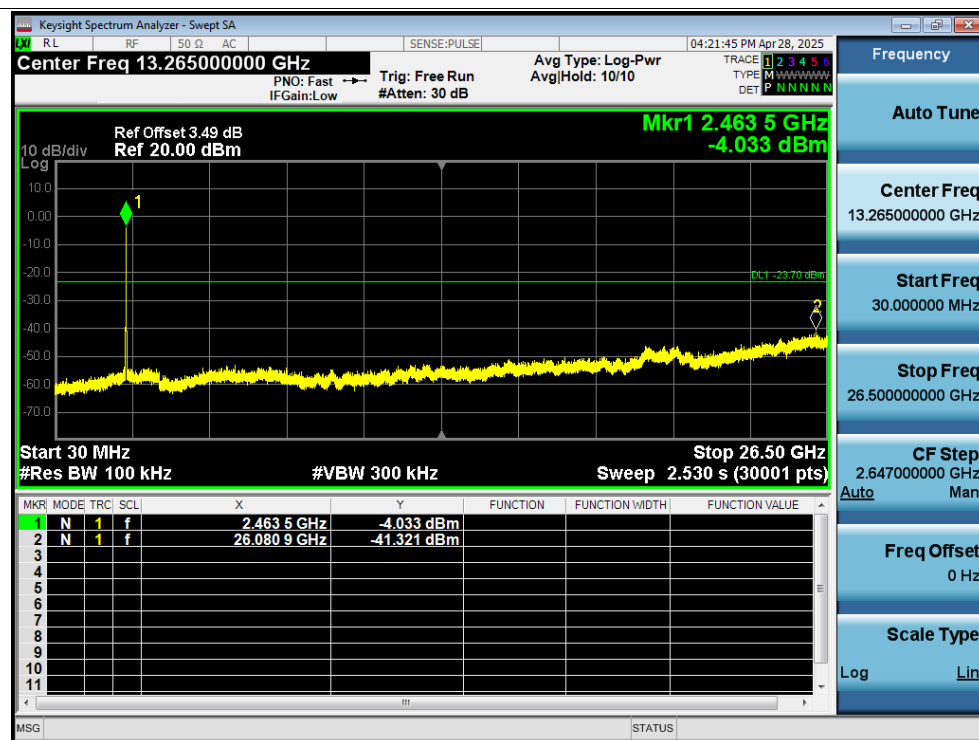
Tx. Spurious NVNT ac20 2462MHz Ant2 Emission
