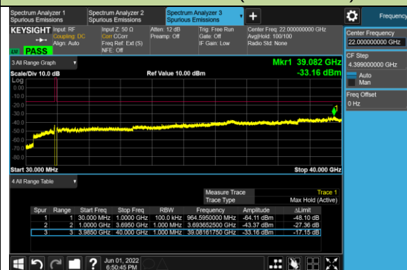
Channel 664332 (3964.98MHz)
