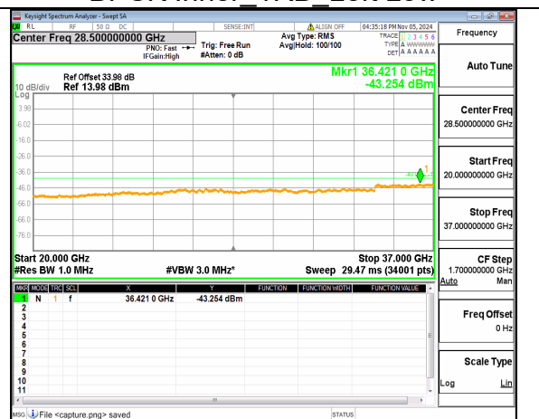
n48 (20GHz-37GHz) 10M DFT-s-OFDM BPSK Inner_1RB_Right Low
