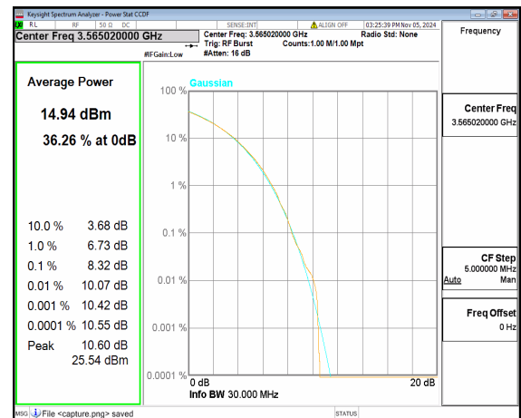
n48 30M CP-OFDM 256QAM Outer_Full Low
