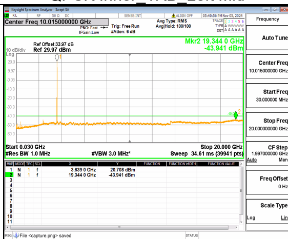
n48 (30MHz-20GHz) 30M DFT-s-OFDM QPSK Inner 1RB Right Mid
