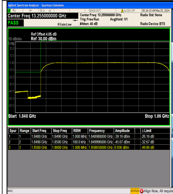
Band25_10MHz_16QAM_26090_50RB#0
