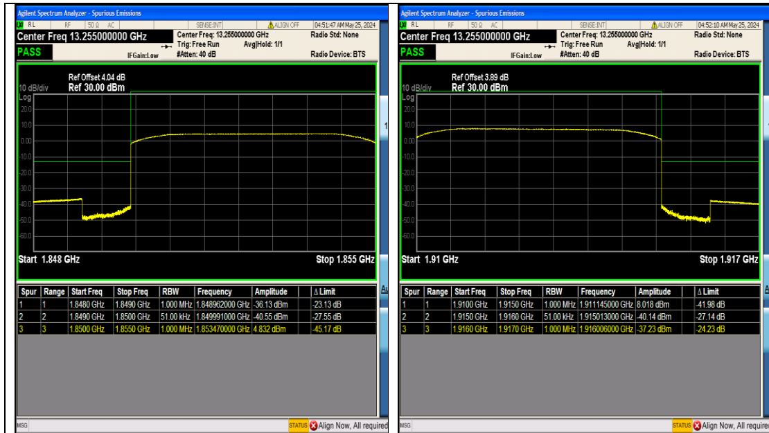
Band25_5MHz_QPSK_26065_25RB#0
