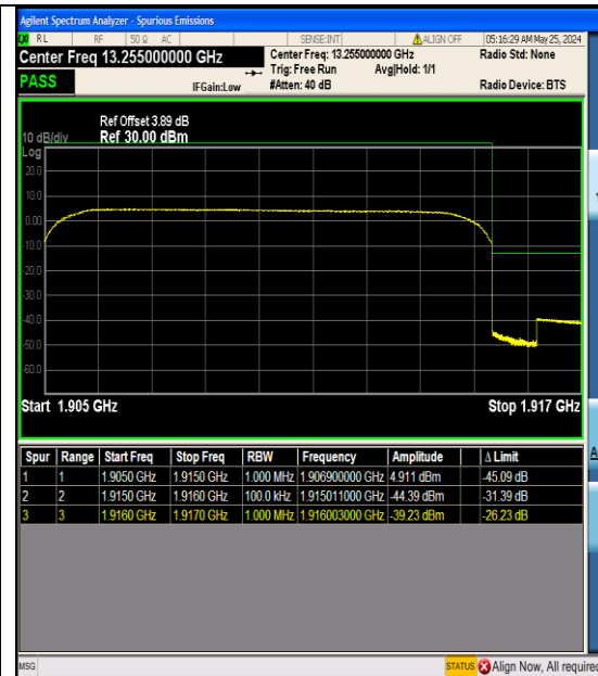
Band25_10MHz_QPSK_26640_50RB#0
