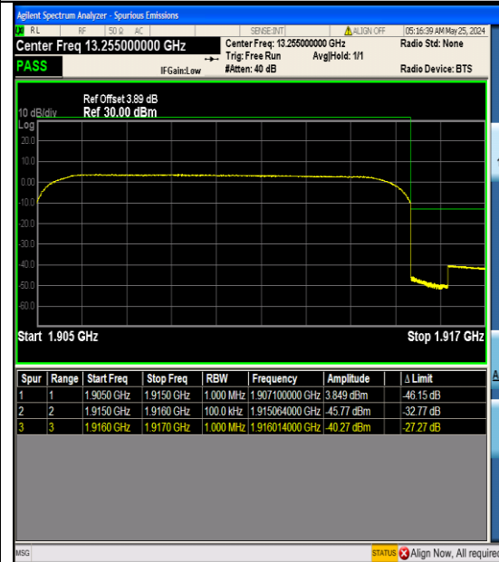
Band25_10MHz_16QAM_26640_50RB#0
