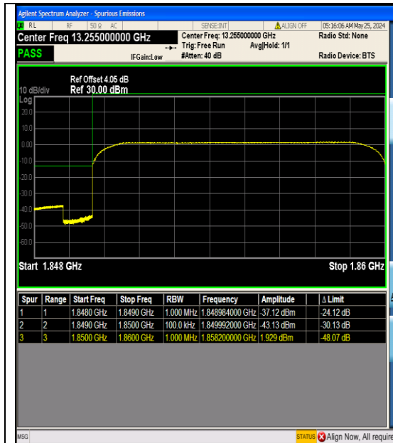
Band25_10MHz_QPSK_26090_50RB#0
