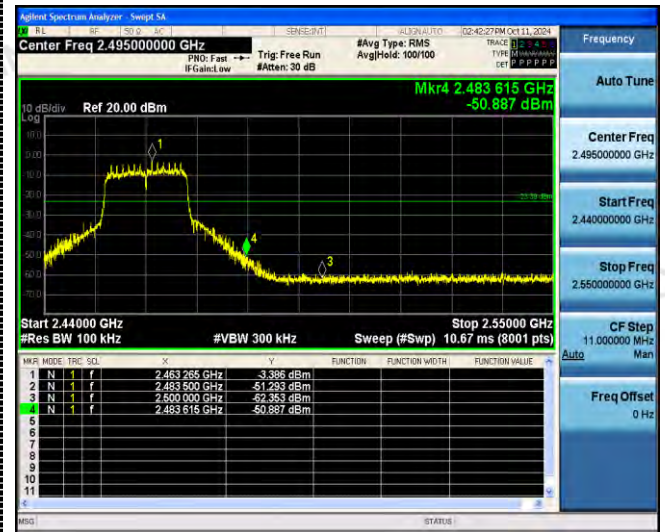
Left bandedge
