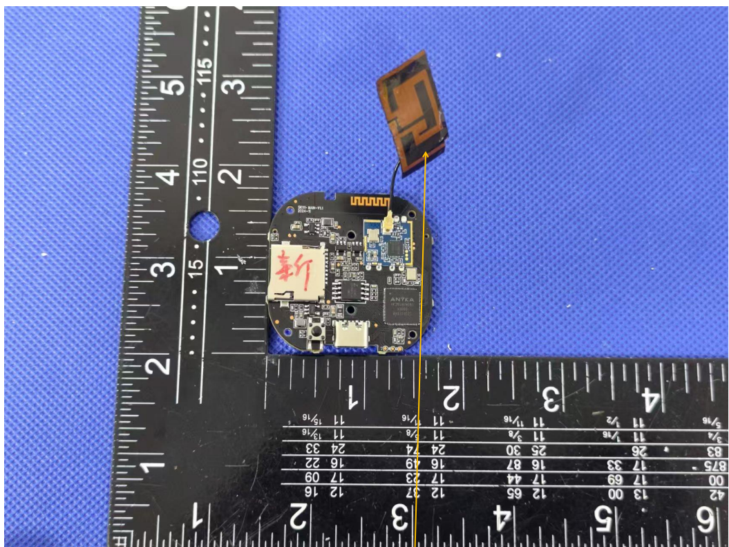
Internal antenna
