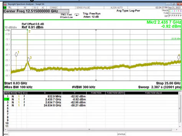
802.11g Middle CH, 2437MHz
