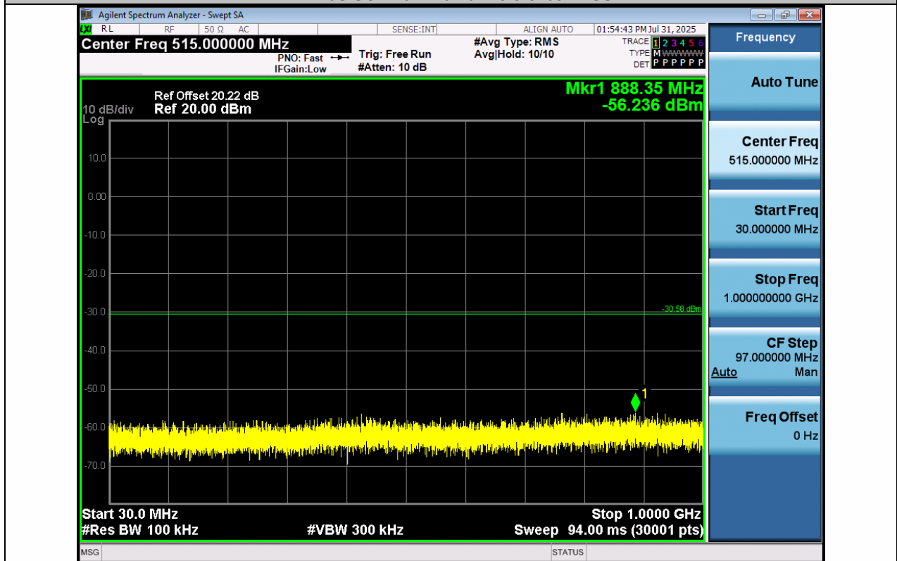
11N20SISO-Ant1-2462-30~1000-PASS
