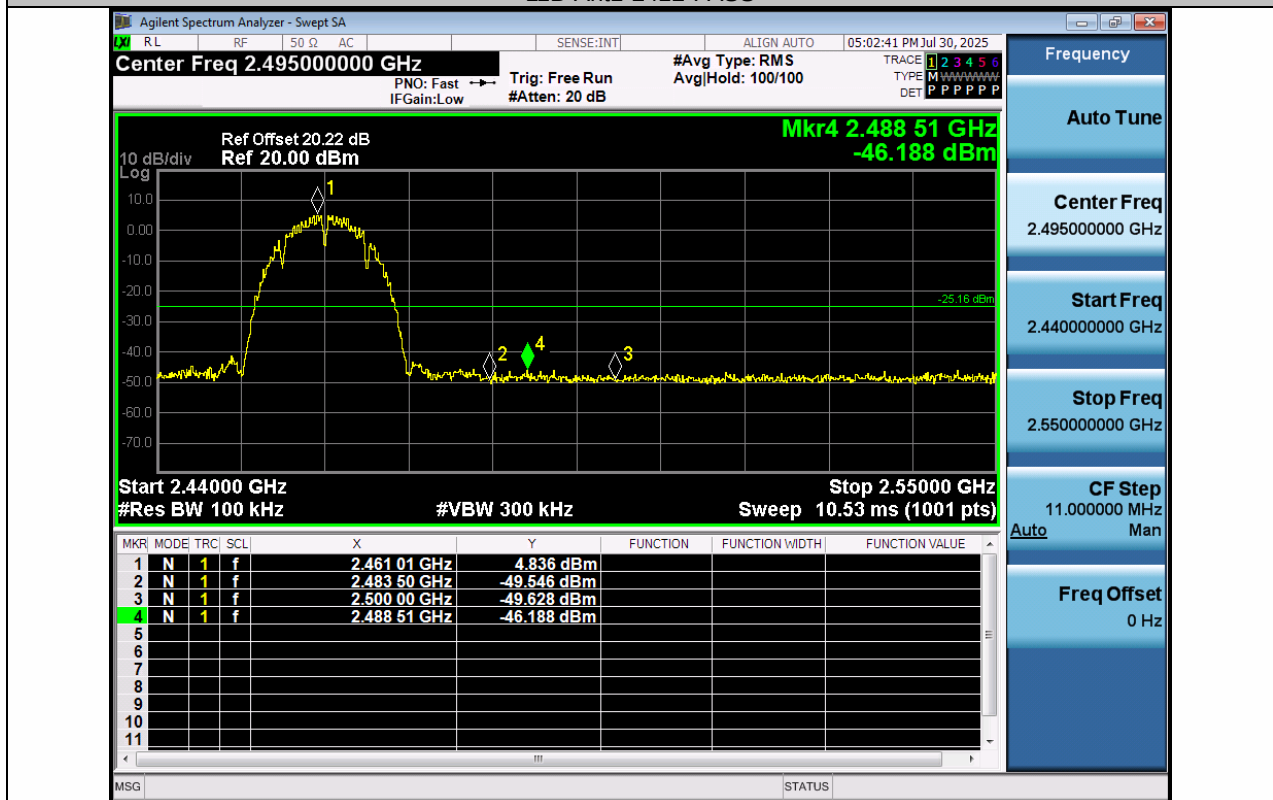
11B-Ant1-2462-PASS
