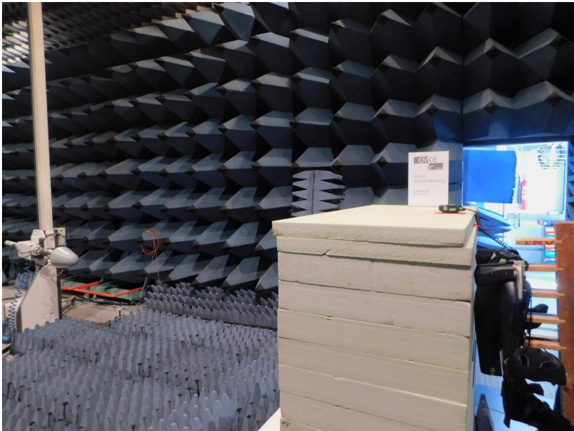
Radiated emission - SAC @3m
