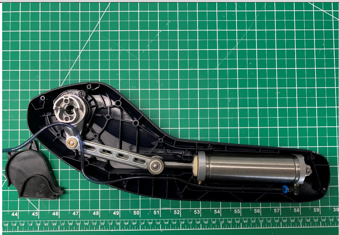
Arm actuator without cover
