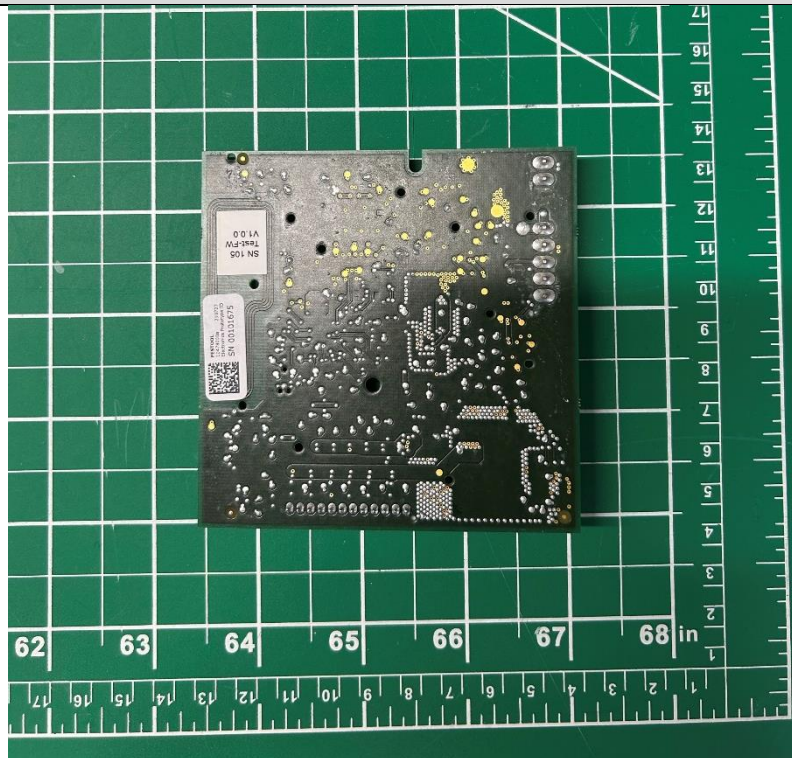
Main electronic – front side (Sample before the potting production step)
