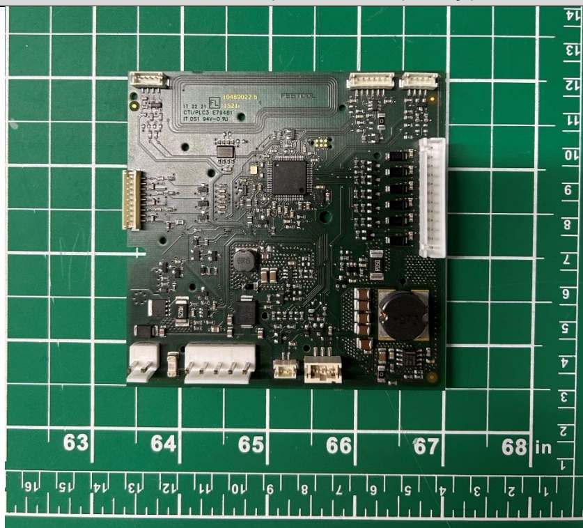
Main electronic – rear side (Sample before the potting production step)
