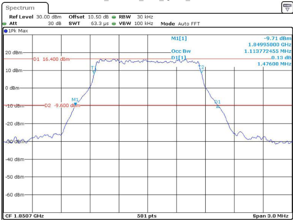
Band 2_1.4 MHz_Low_QPSK_RB6#0
