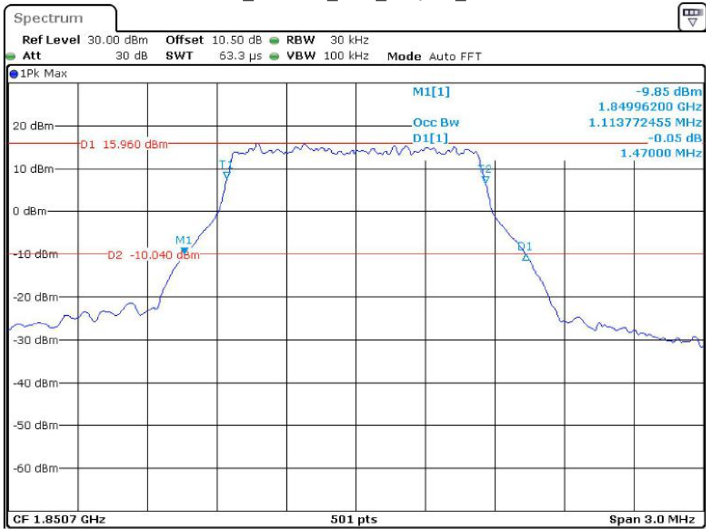
Band 2_1.4 MHz_Low_16QAM_RB6#0
