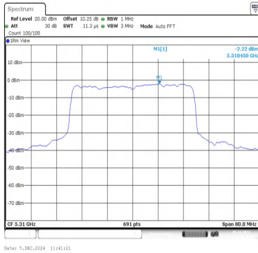
11AX40SISO-Ant1-5310-PASS
