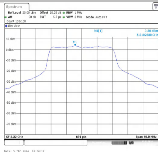
11A-Ant1-5320-PASS
