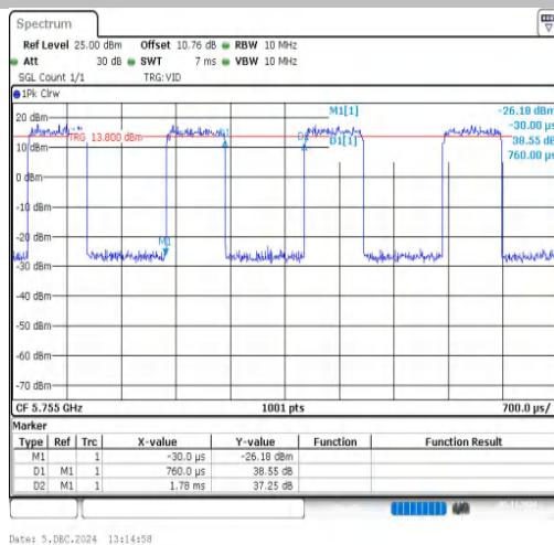
NTNV-11AX40SISO-Ant1-5755
