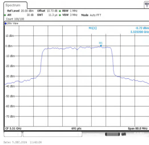
11AX40SISO-Ant1-5510-PASS
