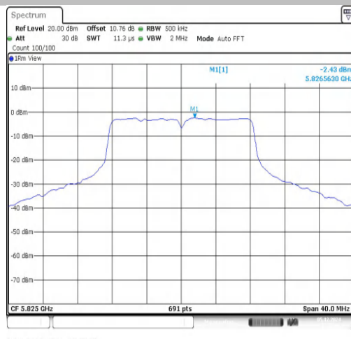
11A-Ant1-5825-PASS
