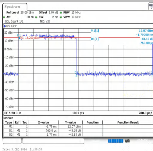
NTNV-11AX40SISO-Ant1-5230
