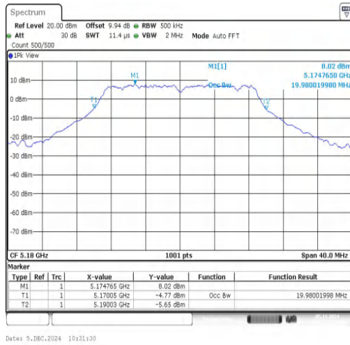
11AC20SISO-Ant1-5180
