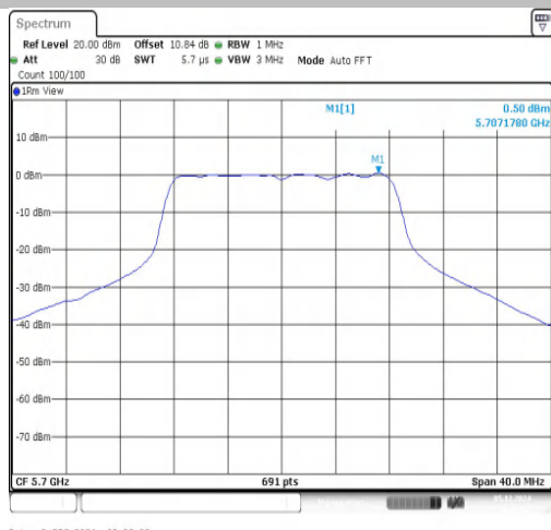
11A-Ant1-5700-PASS
