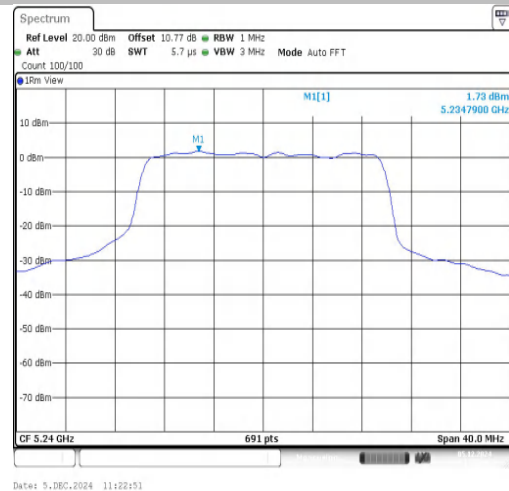
11AX20SISO-Ant1-5240-PASS
