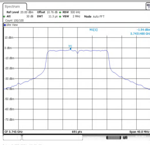
11A-Ant1-5745-PASS
