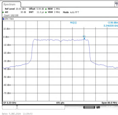
11AX40SISO-Ant1-5230-PASS
