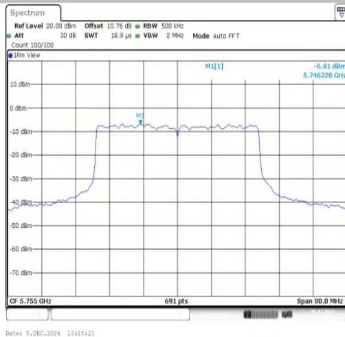
11AX40SISO-Ant1-5755-PASS
