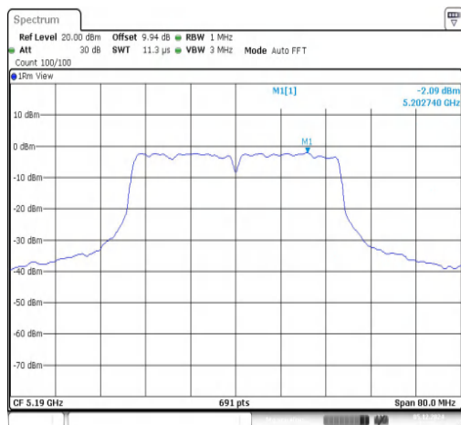
11AC40SISO-Ant1-5190-PASS
