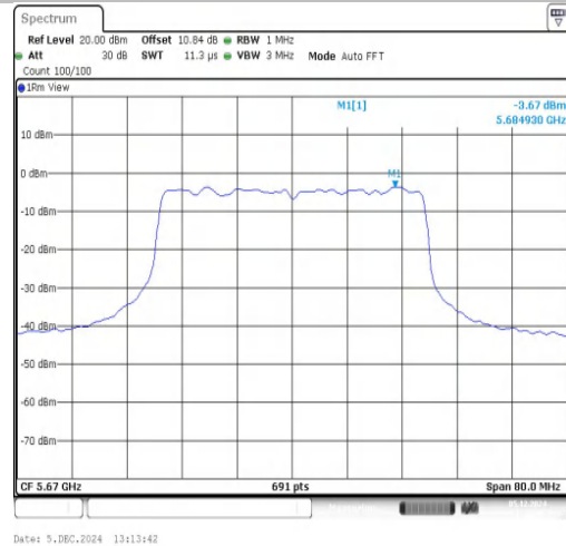
11AX40SISO-Ant1-5670-PASS
