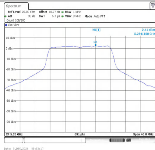
11A-Ant1-5260-PASS
