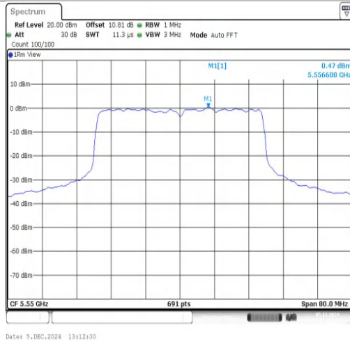
11AX40SISO-Ant1-5550-PASS
