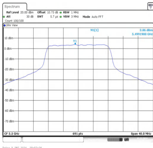
11A-Ant1-5500-PASS
