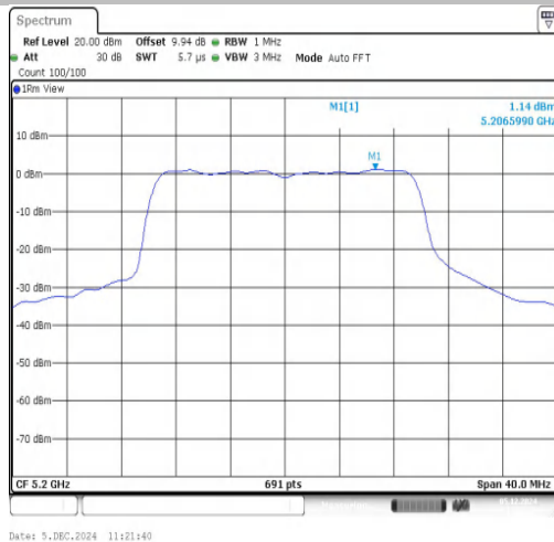
11AX20SISO-Ant1-5200-PASS
