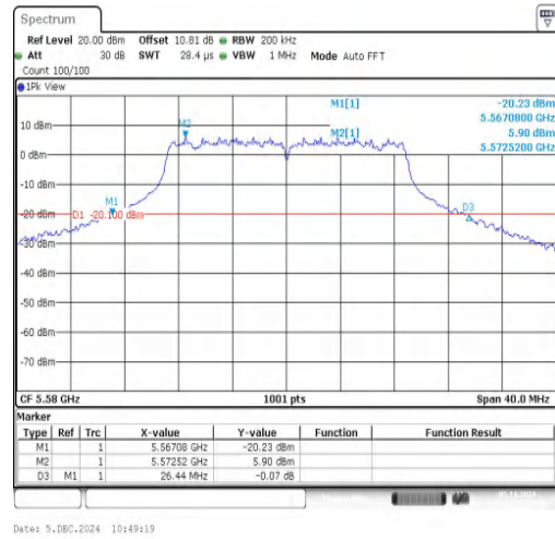
11AC20SISO-Ant1-5580
