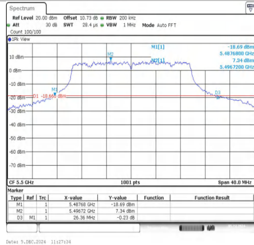
11AX20SISO-Ant1-5500
