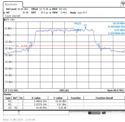
11AX40SISO-Ant1-5510
