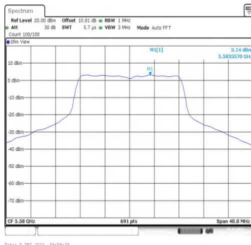
11A-Ant1-5580-PASS
