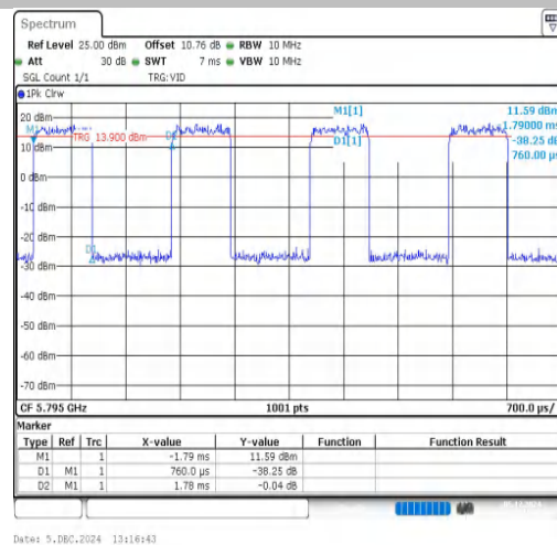
NTNV-11AX40SISO-Ant1-5795
