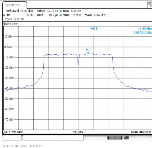
11AC40SISO-Ant1-5795-PASS
