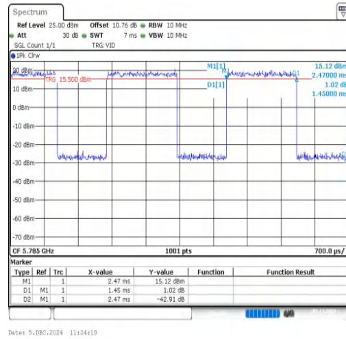
NTNV-11AX20SISO-Ant1-5785
