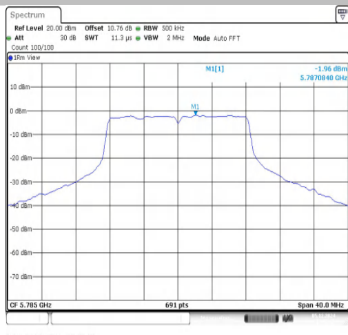
11A-Ant1-5785-PASS
