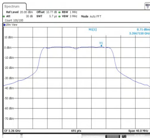
11AX20SISO-Ant1-5260-PASS
