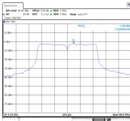
11AC40SISO-Ant1-5230-PASS
