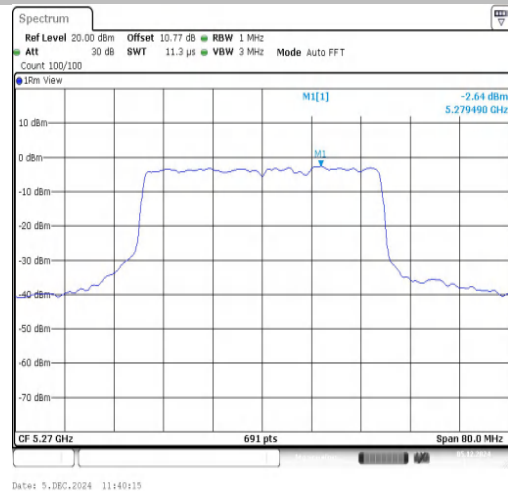
11AX40SISO-Ant1-5270-PASS
