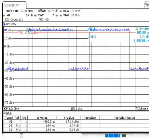
NTNV-11AC20SISO-Ant1-5500
