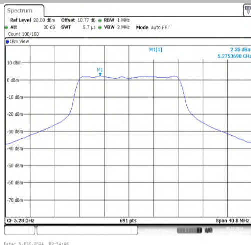
11A-Ant1-5280-PASS
