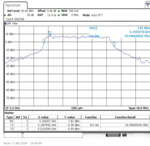
11AC20SISO-Ant1-5200
