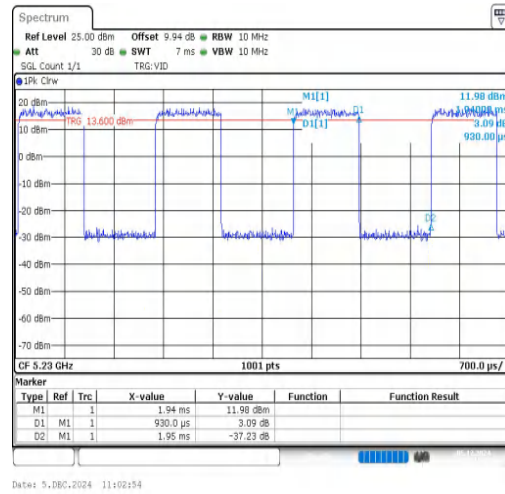
NTNV-11AC40SISO-Ant1-5230
