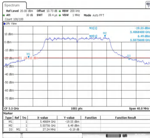
11AC20SISO-Ant1-5500
