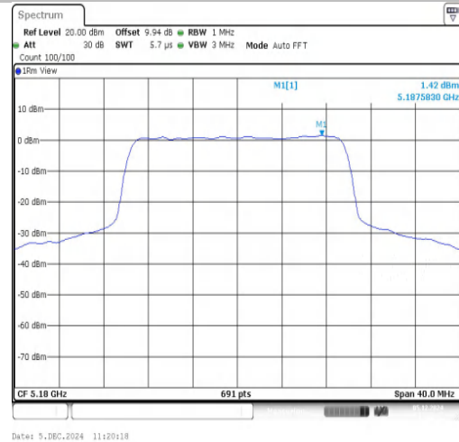
11AX20SISO-Ant1-5180-PASS
