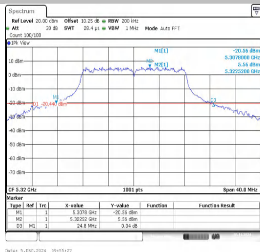
11A-Ant1-5320
