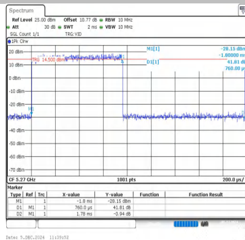
NTNV-11AX40SISO-Ant1-5270
