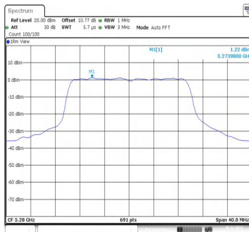
11AX20SISO-Ant1-5280-PASS
