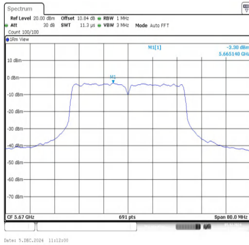
11AC40SISO-Ant1-5670-PASS
