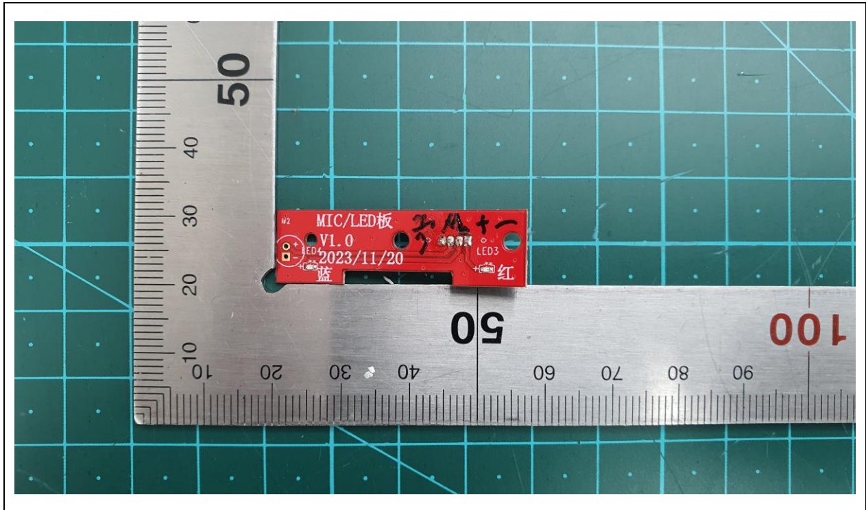
Mic PCB Front
