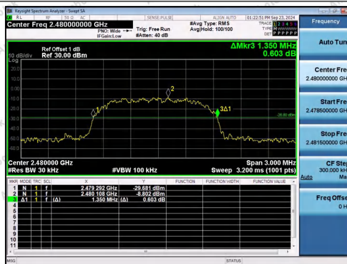
2DH5-Ant1-2480
