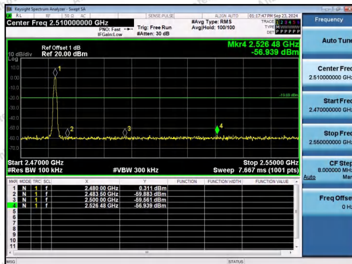
DH5-Ant1-2480-PASS
