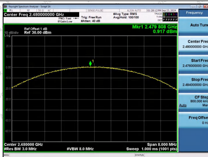
3DH5-Ant1-2480-PASS
