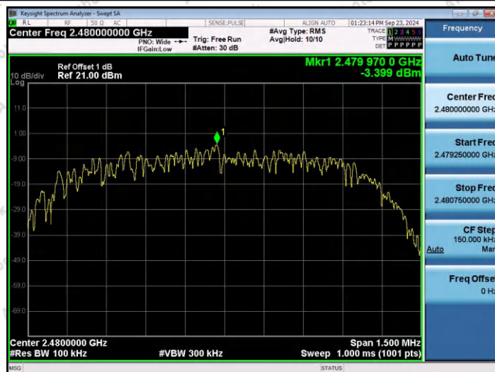
2DH5-Ant1-2480-0~Reference-PASS
