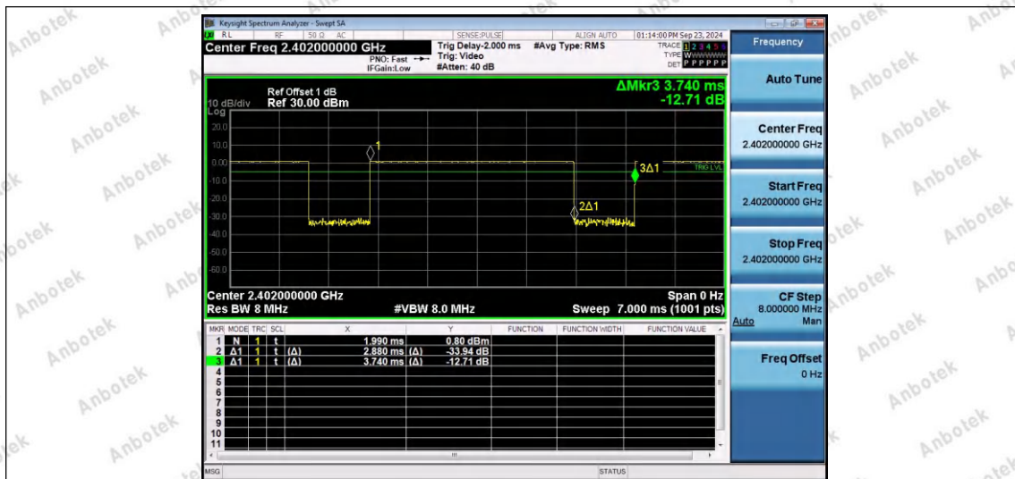
NTNV-DH5-Ant1-2402
