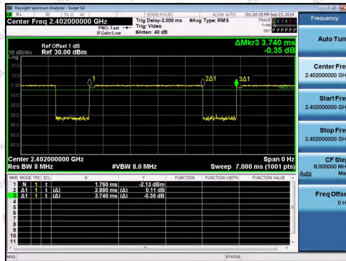
NTNV-3DH5-Ant1-2402
