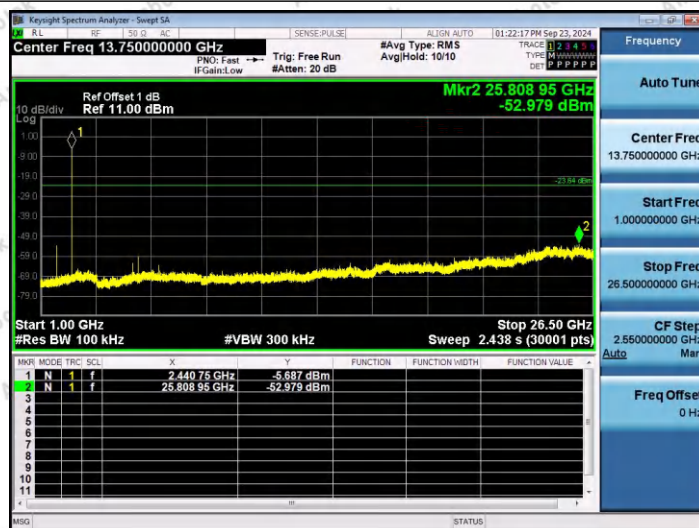
2DH5-Ant1-2441-1000~26500-PASS
