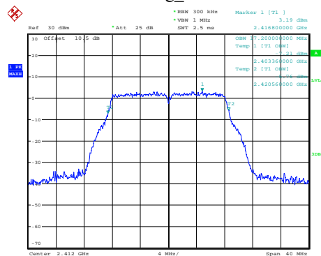
802.11g 2412MHz
