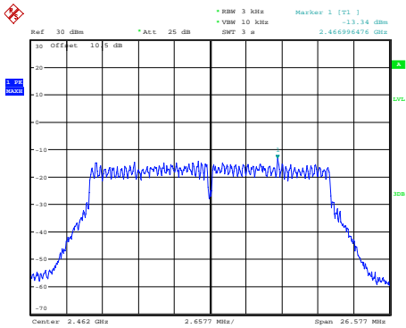
802.11n ht20_2462MHz
