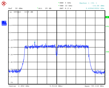
802.11n ht40_2452MHz
