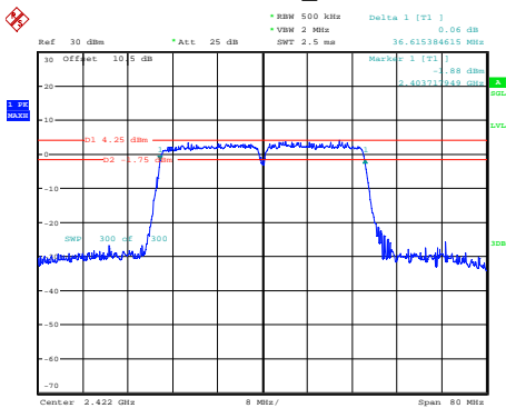
802.11n ht40_2422MHz
