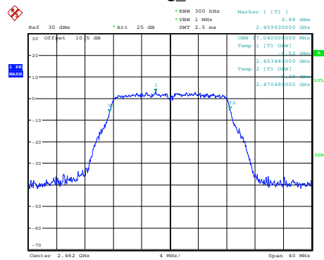
802.11g_2462MHz
