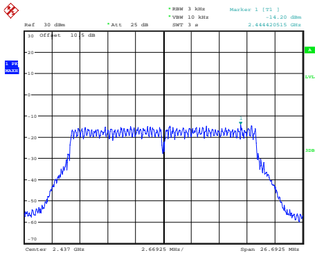
802.11n ht20_2437MHz
