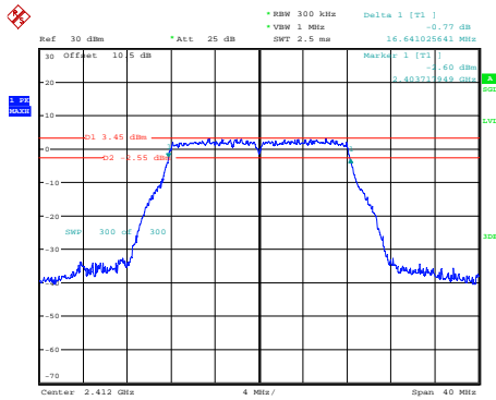
802.11g_2412MHz
