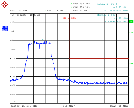
802.11g_2462MHz
