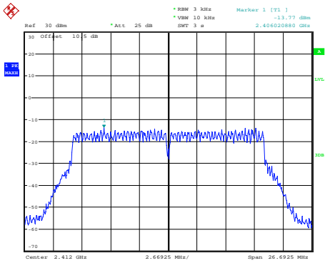
802.11n ht20_2412MHz
