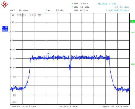
802.11n ht40_2437MHz
