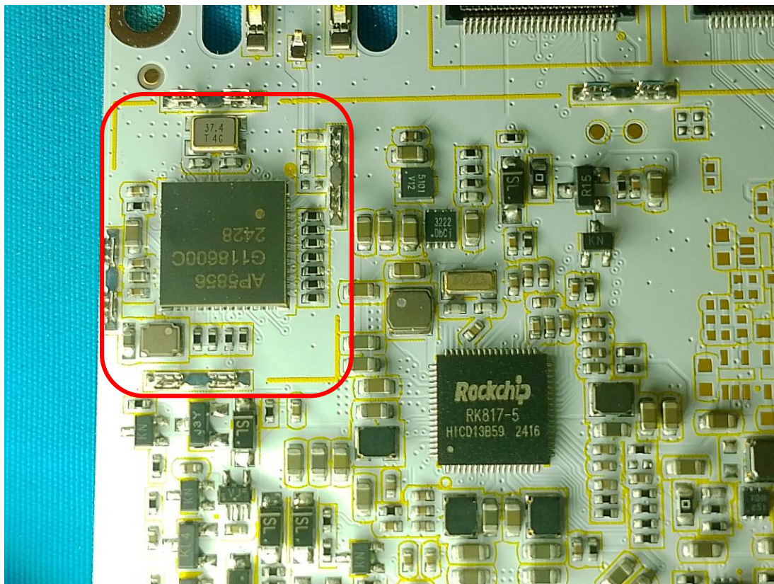
RF Chip
