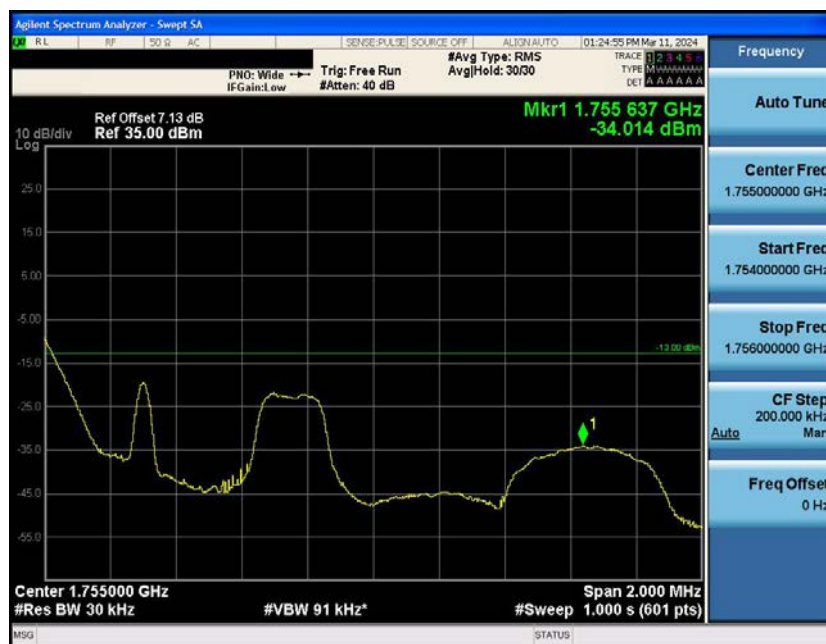
Band4-1.4MHz-16QAM-20393-1RB#5
