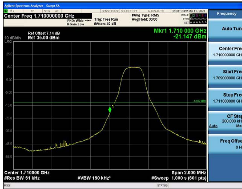
Band4-3MHz-16QAM-19965-1RB#14
