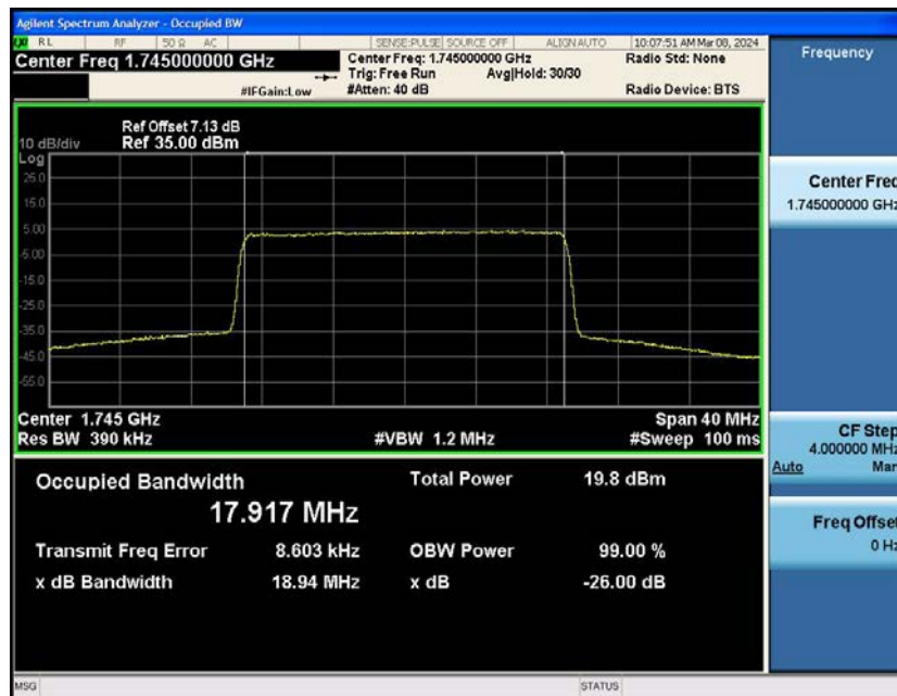
Band4-20MHz-16QAM-20300-100RB#0
