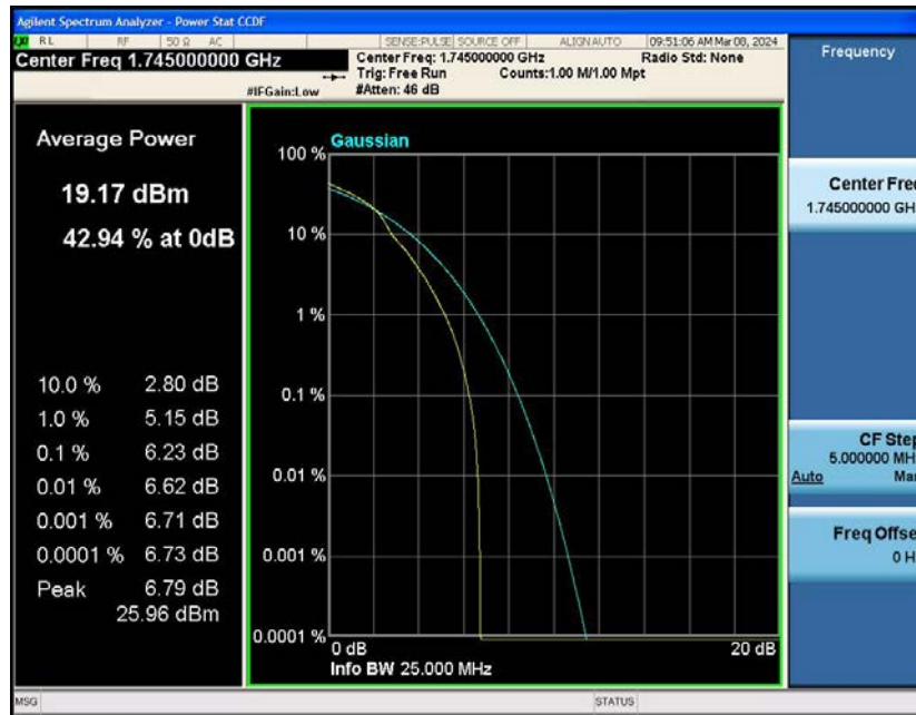
Band4-20MHz-16QAM-20300-100RB#0
