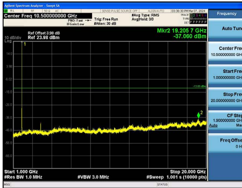
Band2-10MHz-16QAM-18650-1RB#0-Range1:1000~20000MHz
