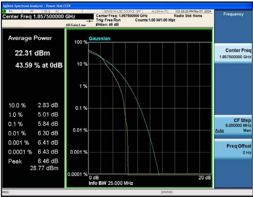
Band2-15MHz-16QAM-18675-75RB#0
