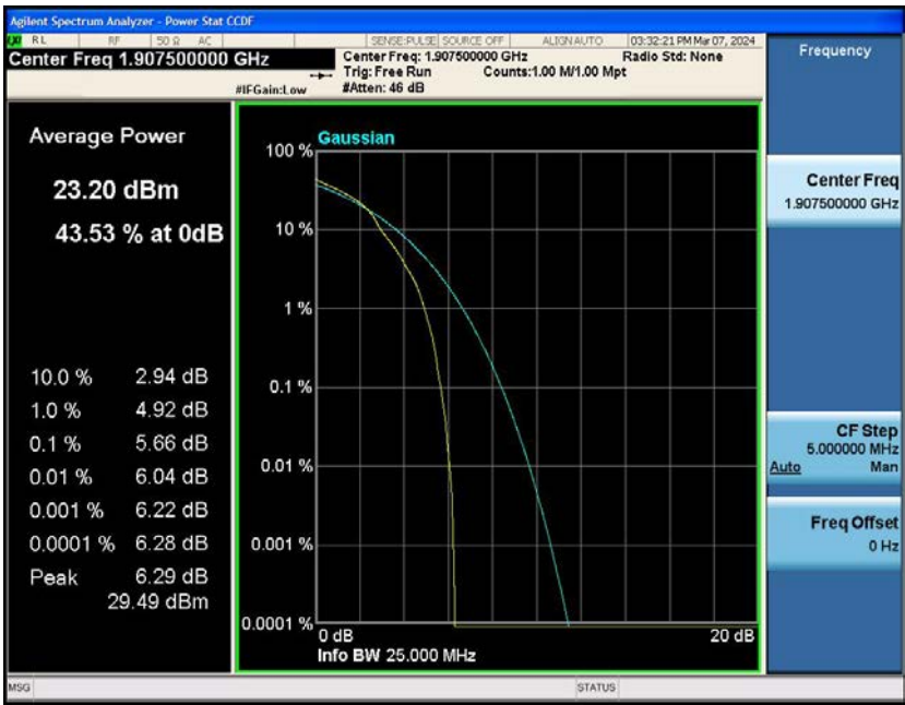
Band2-5MHz-16QAM-19175-25RB#0
