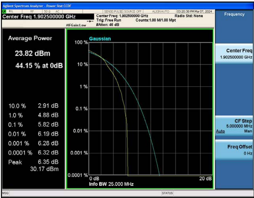
Band2-15MHz-16QAM-19125-75RB#0
