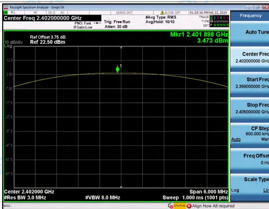
Peak_Output_Power_NVNT_ANT1_1Mbps_2402
