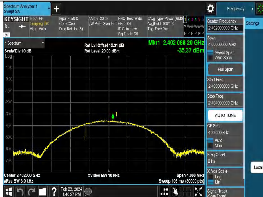
BLE_2M-Ant1-2402-PASS
