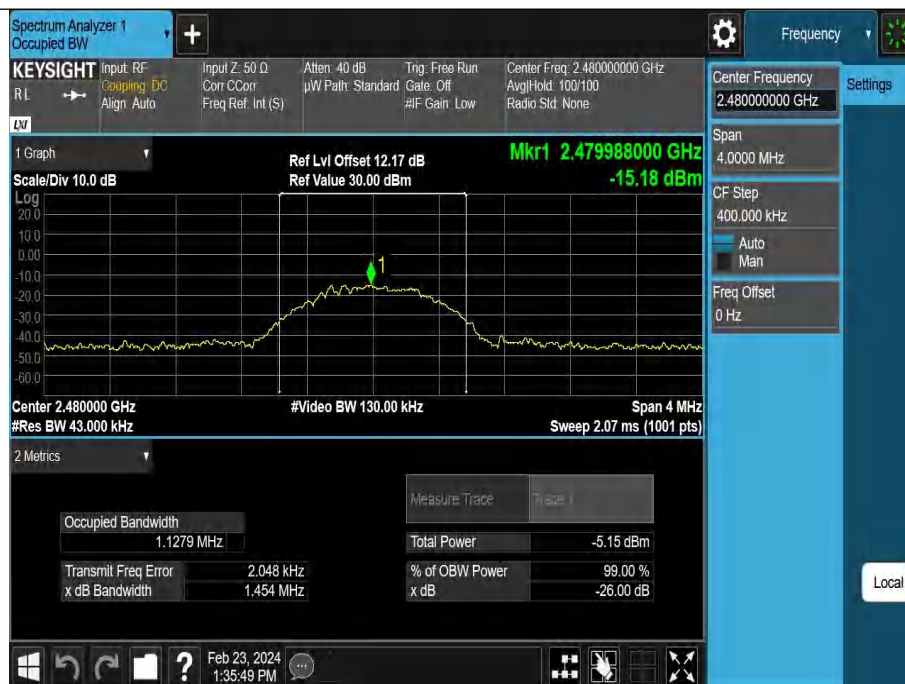
BLE_1M-Ant1-2480
