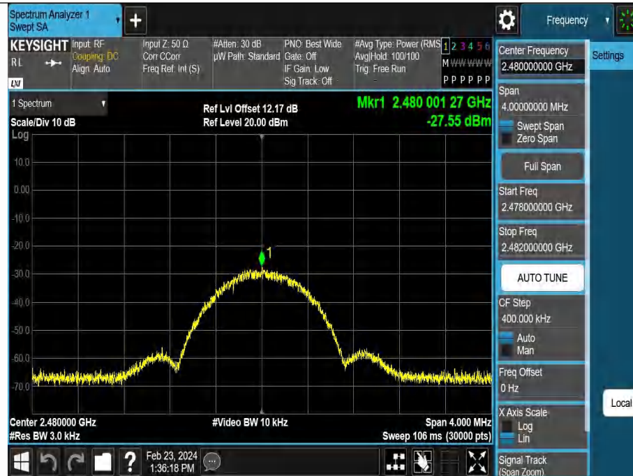
BLE_1M-Ant1-2480-PASS
