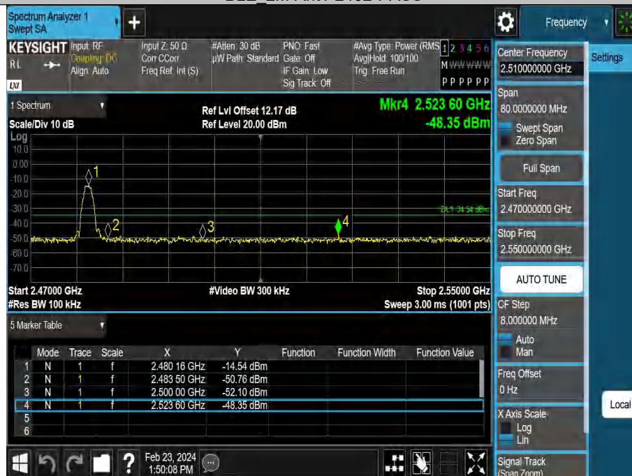
BLE_2M-Ant1-2480-PASS
