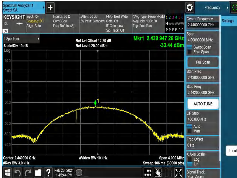
BLE_2M-Ant1-2440-PASS
