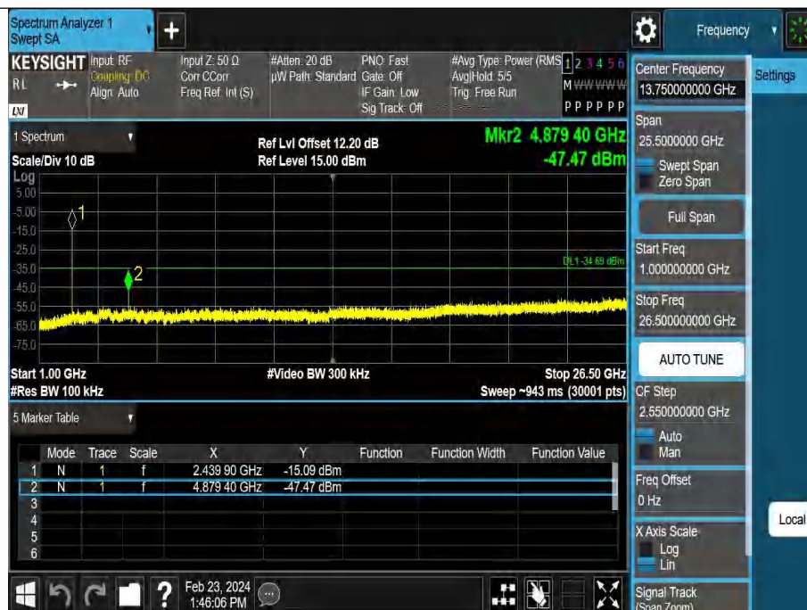
BLE_2M-Ant1-2440-1000~26500-PASS
