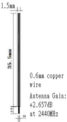
8-1 Antenna size
