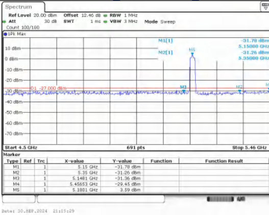
Out Of Band Emission IEEE 802.11ac Channel 36 20MHz
