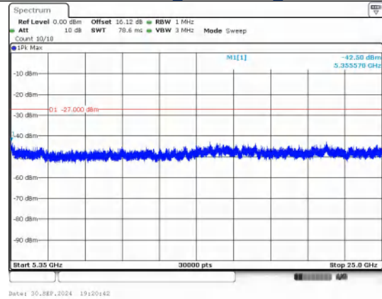
Spurious Emission:5350~25000.0 MHz IEEE 802.11ac_Channel 64_20MHz
