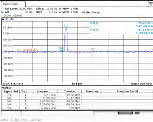
Out Of Band Emission IEEE 802.11ac_Channel 100_20MHz
