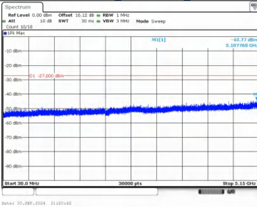
Spurious Emission:30.0~5150 MHz IEEE 802.11ac Channel 40 20MHz
