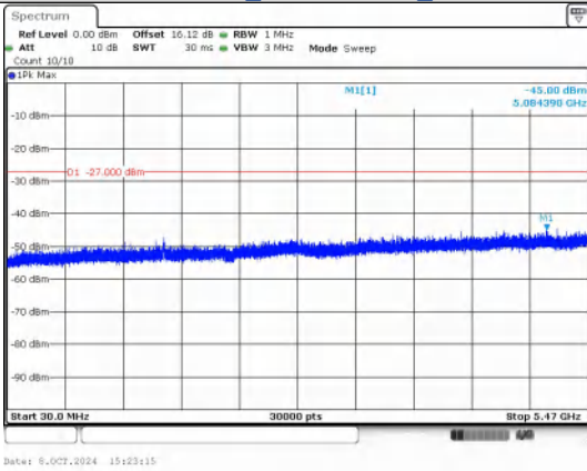
Spurious Emission: 30.0~5470 MHz IEEE 802.11n Channel 140 20MHz
