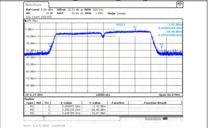
IEEE 802.11ac Channel 54_40MHz_Antenna 0
