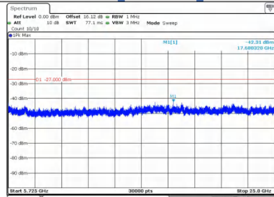
Out Of Band Emission IEEE 802.11a Channel 116 20MHz
