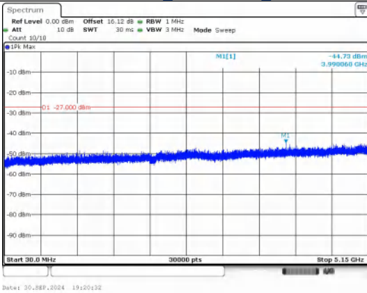
Spurious Emission:30.0~5150 MHz IEEE 802.11ac_Channel 64_20MHz
