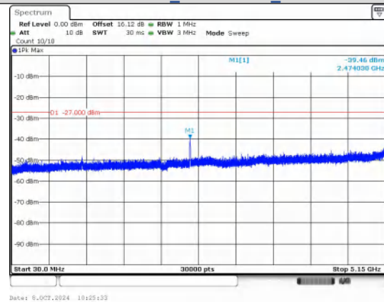
Spurious Emission: 30.0~5150 MHz IEEE 802.11n_Channel 40_20MHz
