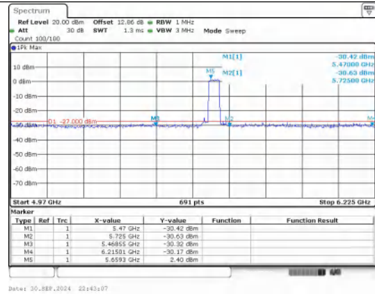
Out Of Band Emission IEEE 802.11n Channel 134 40MHz
