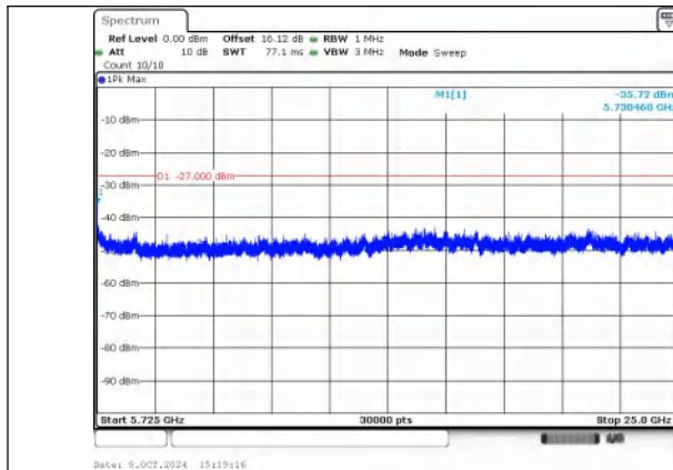
Spurious Emission: 5725~25000.0 MHz IEEE 802.11a_Channel 140_20MHz
