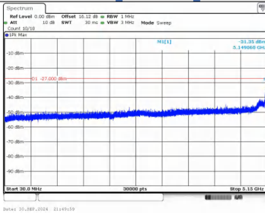
Spurious Emission: 30.0~5150 MHz IEEE 802.11ac Channel 42 80MHz
