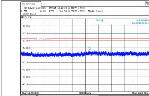
Spurious Emission:5350~25000.0 MHz IEEE 802.11ac Channel 36 20MHz
