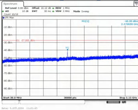
Spurious Emission:30.0~5150 MHz IEEE 802.11a_Channel 52_20MHz
