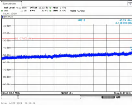
Spurious Emission:30.0~5470 MHz IEEE 802.11ac_Channel 106_80MHz
