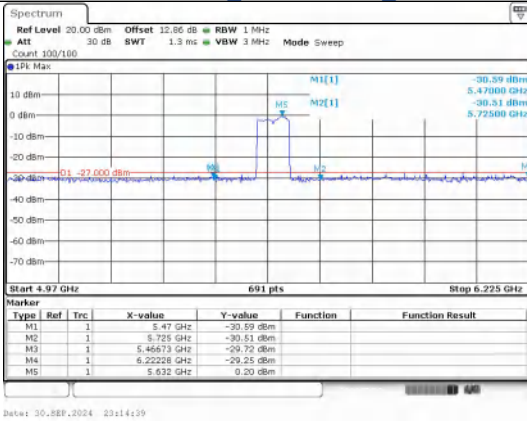
Out Of Band Emission IEEE 802.11ac_Channel 122_80MHz
