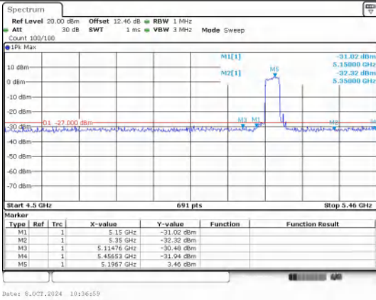
Out Of Band Emission IEEE 802.11n Channel 38 40MHz
