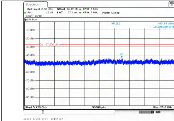
Spurious Emission: 5725~25000.0 MHz IEEE 802.11n Channel 116 20MHz
