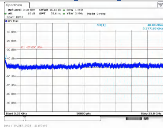
Spurious Emission: 5350~25000.0 MHz IEEE 802.11ac Channel 42 80MHz
