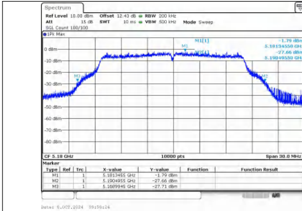
IEEE 802.11a Channel 36 20MHz Antenna 0
