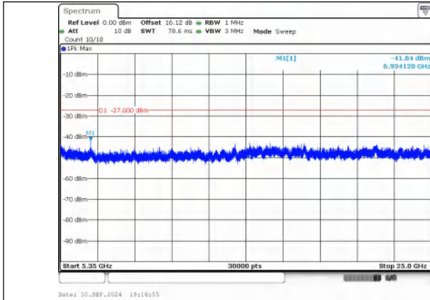
Spurious Emission:5350~25000.0 MHz IEEE 802.11ac_Channel 60_20MHz
