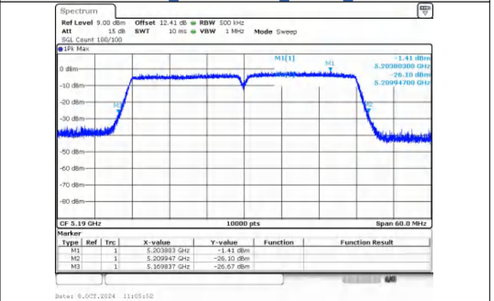
IEEE 802.11ac Channel 38_40MHz_Antenna 0
