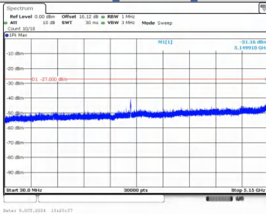
Spurious Emission: 30.0~5150 MHz IEEE 802.11n_Channel 36_20MHz
