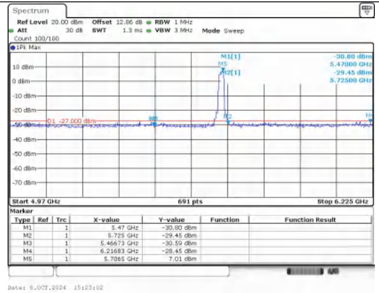
Out Of Band Emission IEEE 802.11n Channel 140 20MHz
