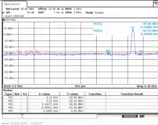
Out Of Band Emission IEEE 802.11a_Channel 60_20MHz
