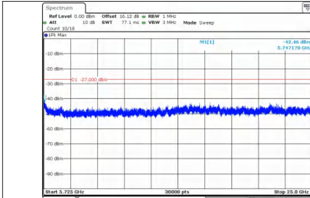
Spurious Emission: 5725~25000.0 MHz IEEE 802.11ac Channel 134 40MHz
