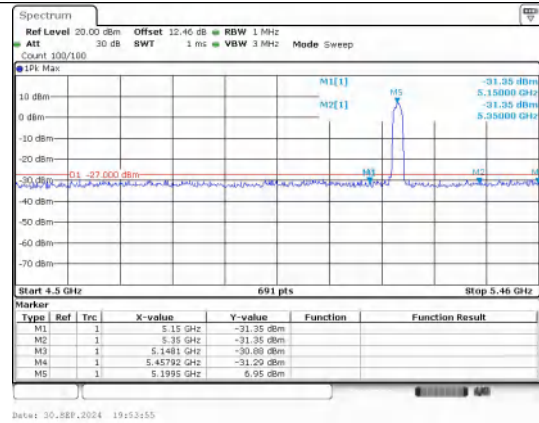
Out Of Band Emission IEEE 802.11a_Channel 40_20MHz
