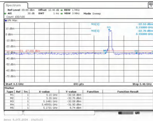
Out Of Band Emission IEEE 802.11n_Channel 36_20MHz
