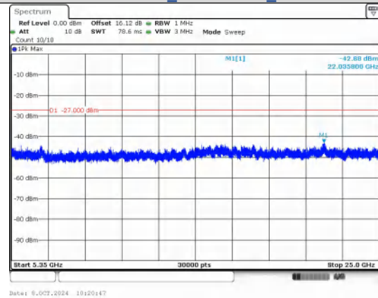
Spurious Emission: 5350~25000.0 MHz IEEE 802.11n_Channel 36_20MHz
