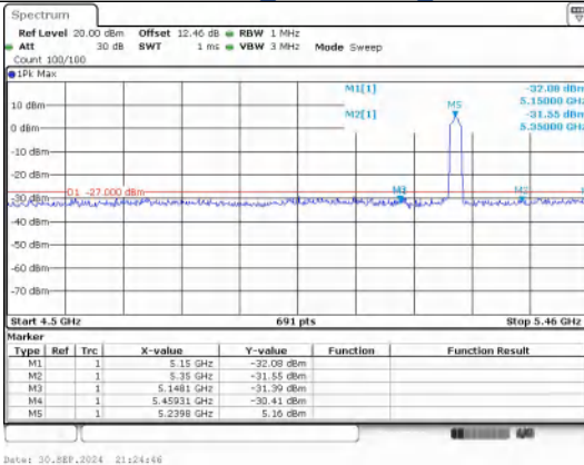
Out Of Band Emission IEEE 802.11ac Channel 48 20MHz
