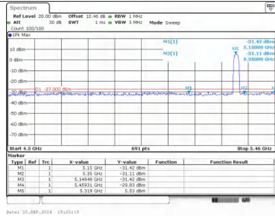
Out Of Band Emission IEEE 802.11ac_Channel 64_20MHz
