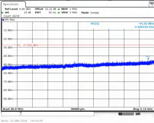
Spurious Emission:30.0~5150 MHz IEEE 802.11a_Channel 40_20MHz
