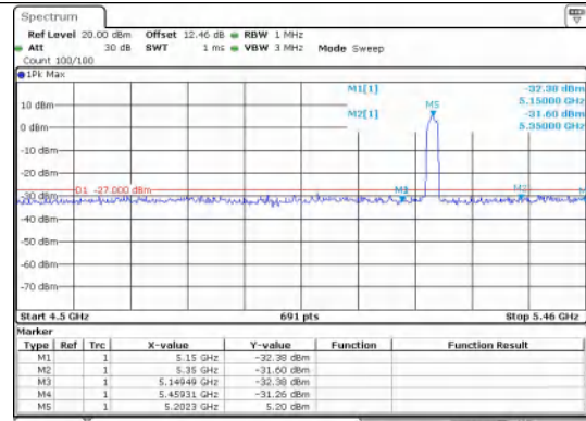
Out Of Band Emission IEEE 802.11ac Channel 40 20MHz
