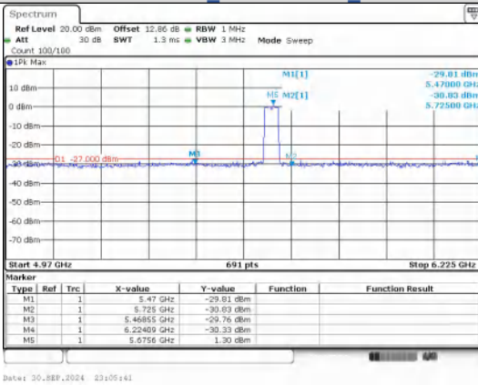
Out Of Band Emission IEEE 802.11ac_Channel 134_40MHz
