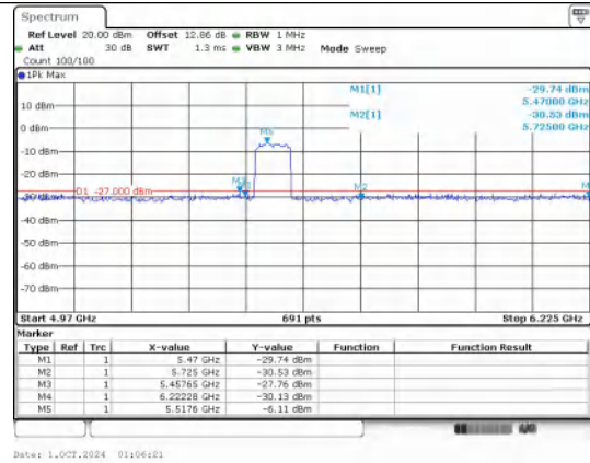
Out Of Band Emission IEEE 802.11ac_Channel 106_80MHz
