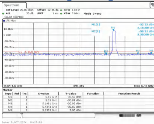
Out Of Band Emission IEEE 802.11n_Channel 40_20MHz
