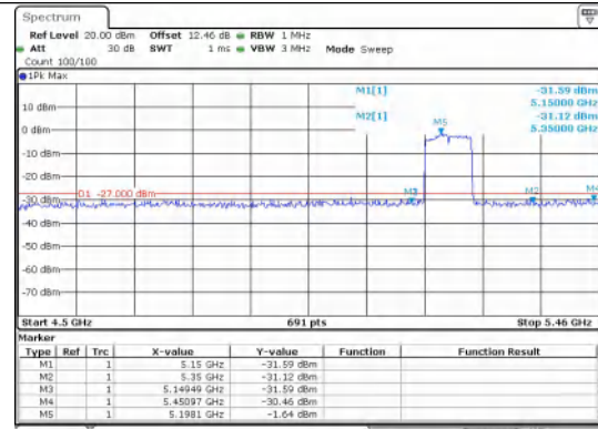
Out Of Band Emission IEEE 802.11ac Channel 42 80MHz
