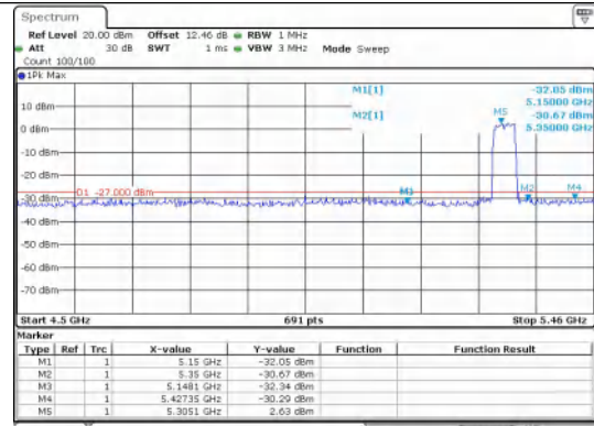
Out Of Band Emission IEEE 802.11n_Channel 62_40MHz
