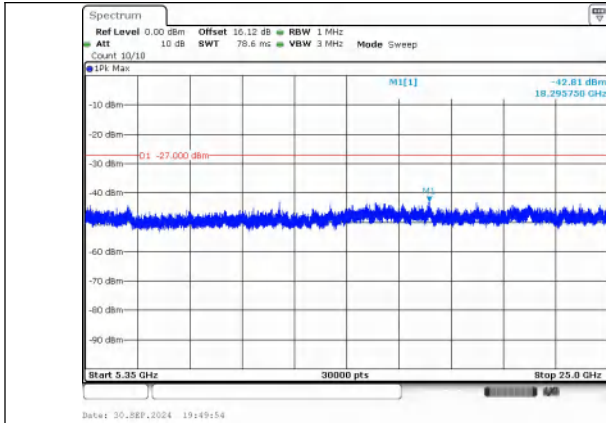
Spurious Emission:5350~25000.0 MHz IEEE 802.11a_Channel 36_20MHz
