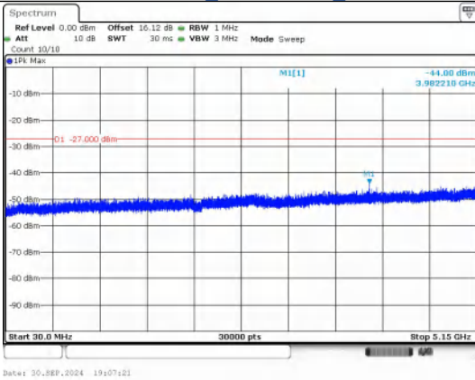
Spurious Emission:30.0~5150 MHz IEEE 802.11n_Channel 62_40MHz
