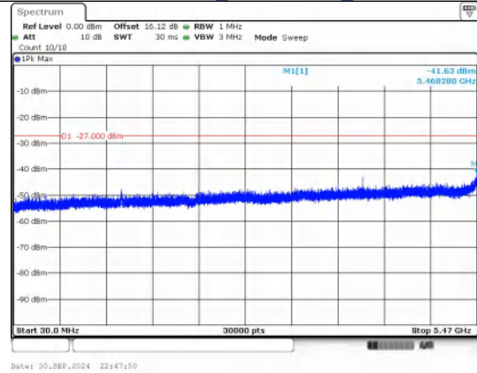
Spurious Emission:30.0~5470 MHz IEEE 802.11ac_Channel 100_20MHz
