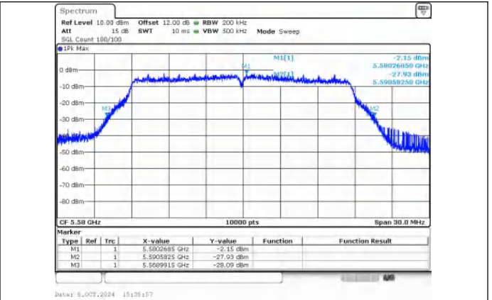
IEEE 802.11ac Channel 116_20MHz_Antenna 0
