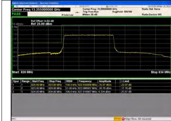
Band 5 5MHz/826.5/Low QPSK 25@0
