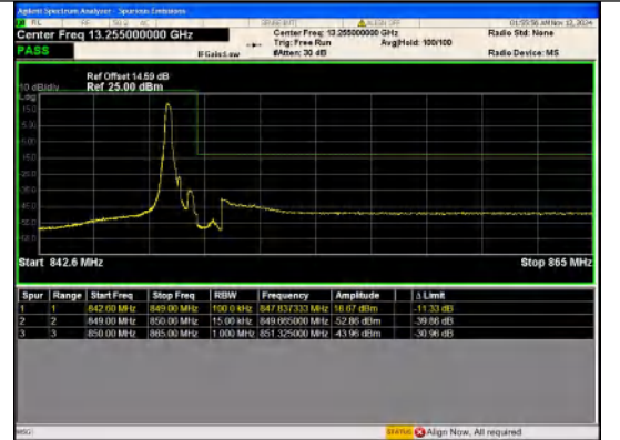
Band 5 1.4MHz/848.3/High 16QAM 1@0
