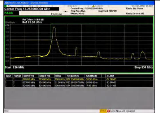
Band 5 5MHz/826.5/Low 16QAM 1@0
