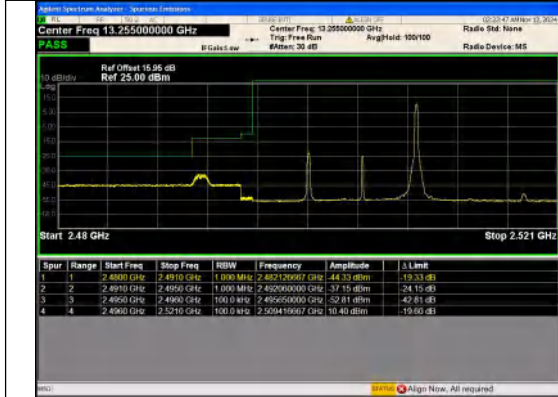
Band 7 10MHz/2505.0/Low 16QAM 1@49
