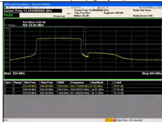
Band 5 10MHz/844.0/High 16QAM 50@0
