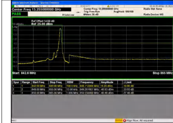
Band 5 1.4MHz/848.3/High 16QAM 1@5
