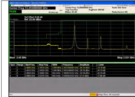
Band 7 10MHz/2505.0/Low QPSK 1@0
