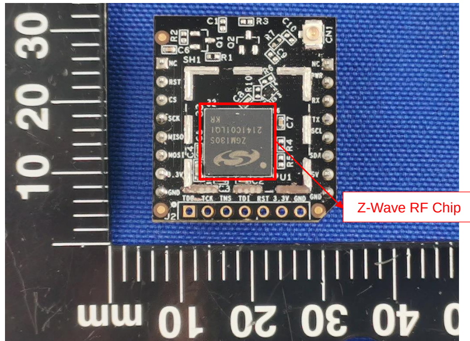
SECONDARY BOARD 1 TOP VIEW (WITHOUT SHIELDING)
